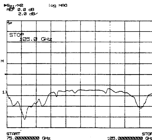
Fig. 5 S_{21} of test circuit at W-band
