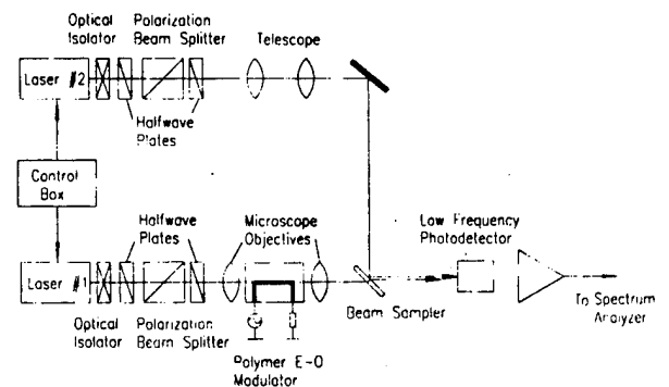
FIG. 1. The experiment setup for optical heterodyne detection of millimeter wave electro-optic modulation from a polymer phase modulator. Two diode pumped Nd:YAG lasers were in open loop running condition.
