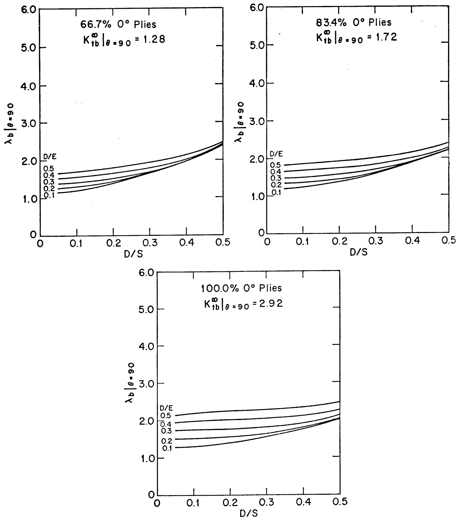
Figure 17 (Cont'd). Loaded Hold Finite Size Correction Factors, \lambda_b|_{\theta=90} , for [0/±45] Boron-Epoxy Laminates
