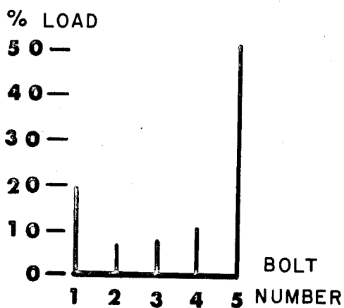
(c) Specimen 3
