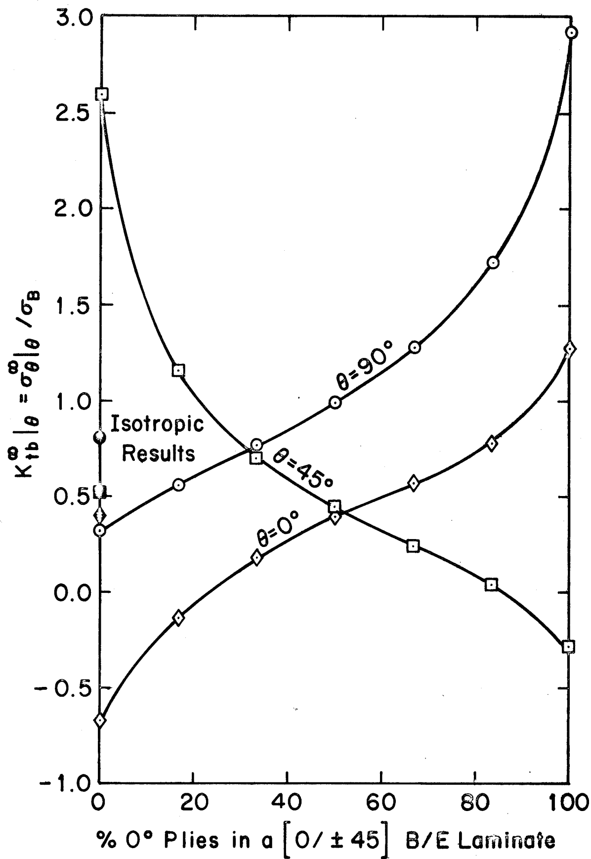
Figure 11. Infinite Plate Stress Concentration Factors, K_{tb}^{\infty} , for a Loaded Hole in [0/\pm 45] Boron-Epoxy Laminates tb .
