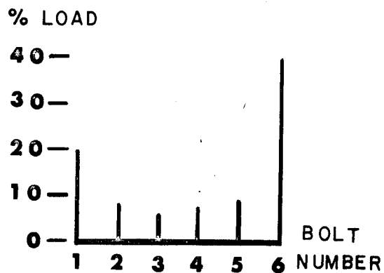
(a) Specimen 1
