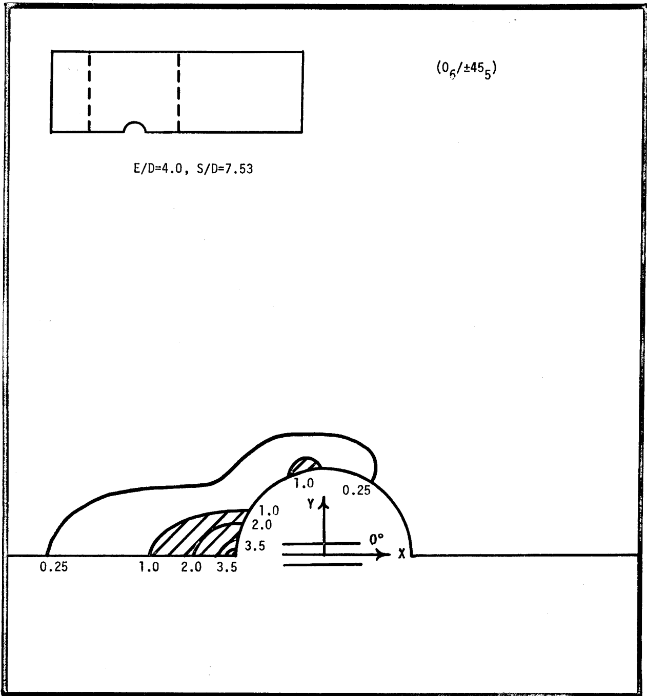
Figure A-9. Bearing Failure: THC Contour Plot, 0^\circ Plies
