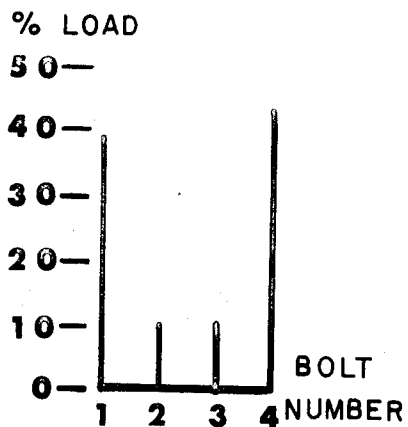
(e) Specimen 5
