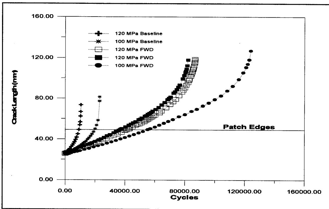
Figure 60. 100 vs. 120 MPa Baseline and FWD Crack Growth
