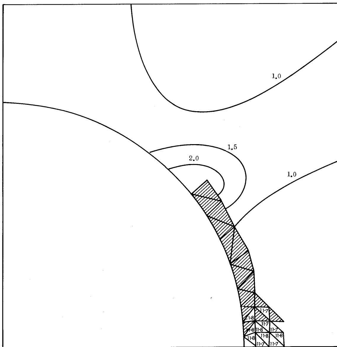
Fig. 16 — Failed elements and octahedral shear stress contours (normalized) Computer run 8A-19-25, applied stress increment 11-9
