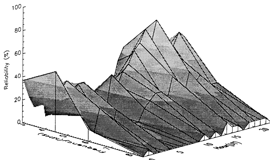
Figure 8.3 Measured reliability, Andøya-Alta (285 km), March/April 1988, days where Q > 4 . Two different viewing angles
