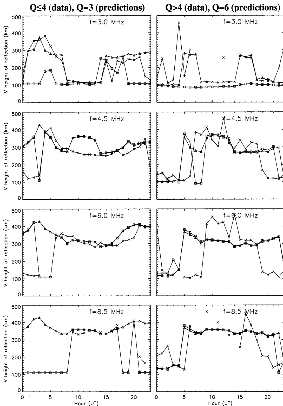
Figure 8.8 Virtual height of reflection for median of measured data (X), unmodified predictions (Δ) and predictions with both the F&T-model and mode availability included (□). Path Andøya-Alta (285 km), March/April 1988
