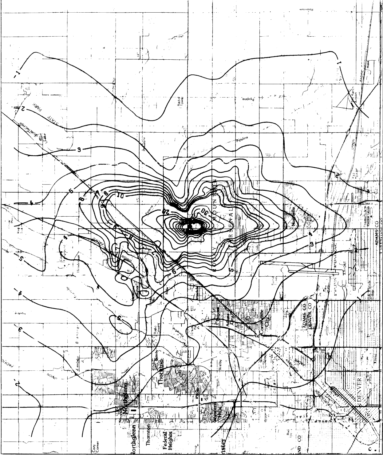
FIGURE 6-1 FIVE YEAR AVERAGE CONCENTRATION ISOPLETH ( \mu\text{gm}/\text{m}^3 )
