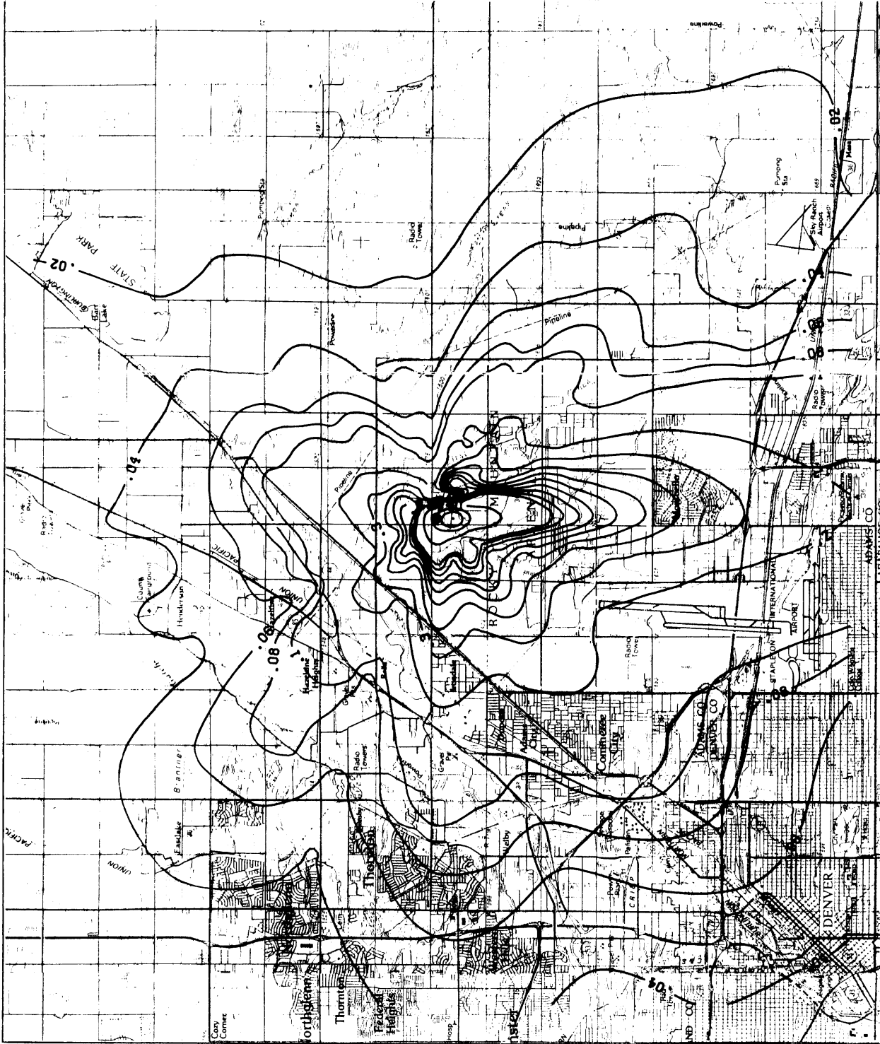
FIGURE 6-4 FIVE YEAR AVERAGE TOTAL DEPOSITION ISOPLETH (gm/m 2 )
