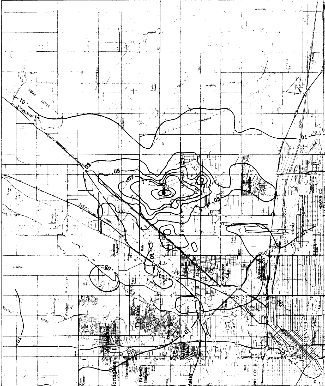
FIGURE 6-2 FIVE YEAR AVERAGE DRY DEPOSITION ISOPLETH (gm/m 2 )
