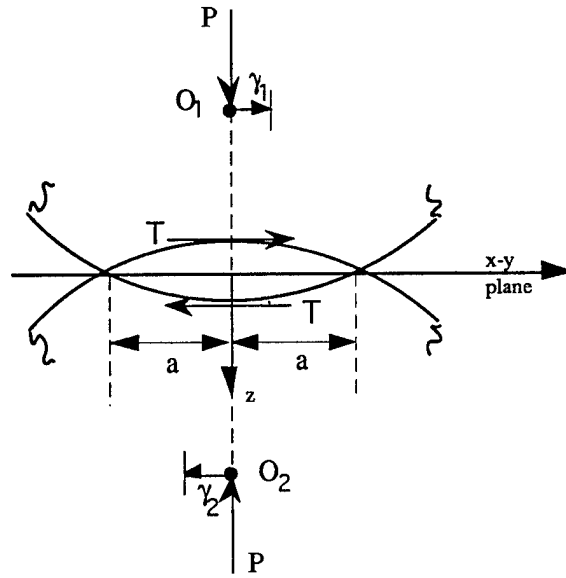
Figure 32. Tangential displacements of two contacting cylinders.
