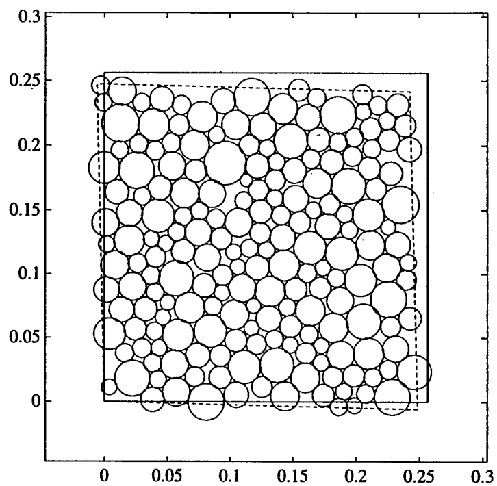
Figure 30. Deformed configuration for the 196-particle assembly; mean particle radius = 0.0092 units.
