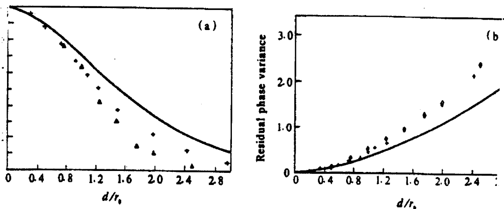
Fig. 2 Strehl ratio (a) and residual phase variance vs d/r_0
