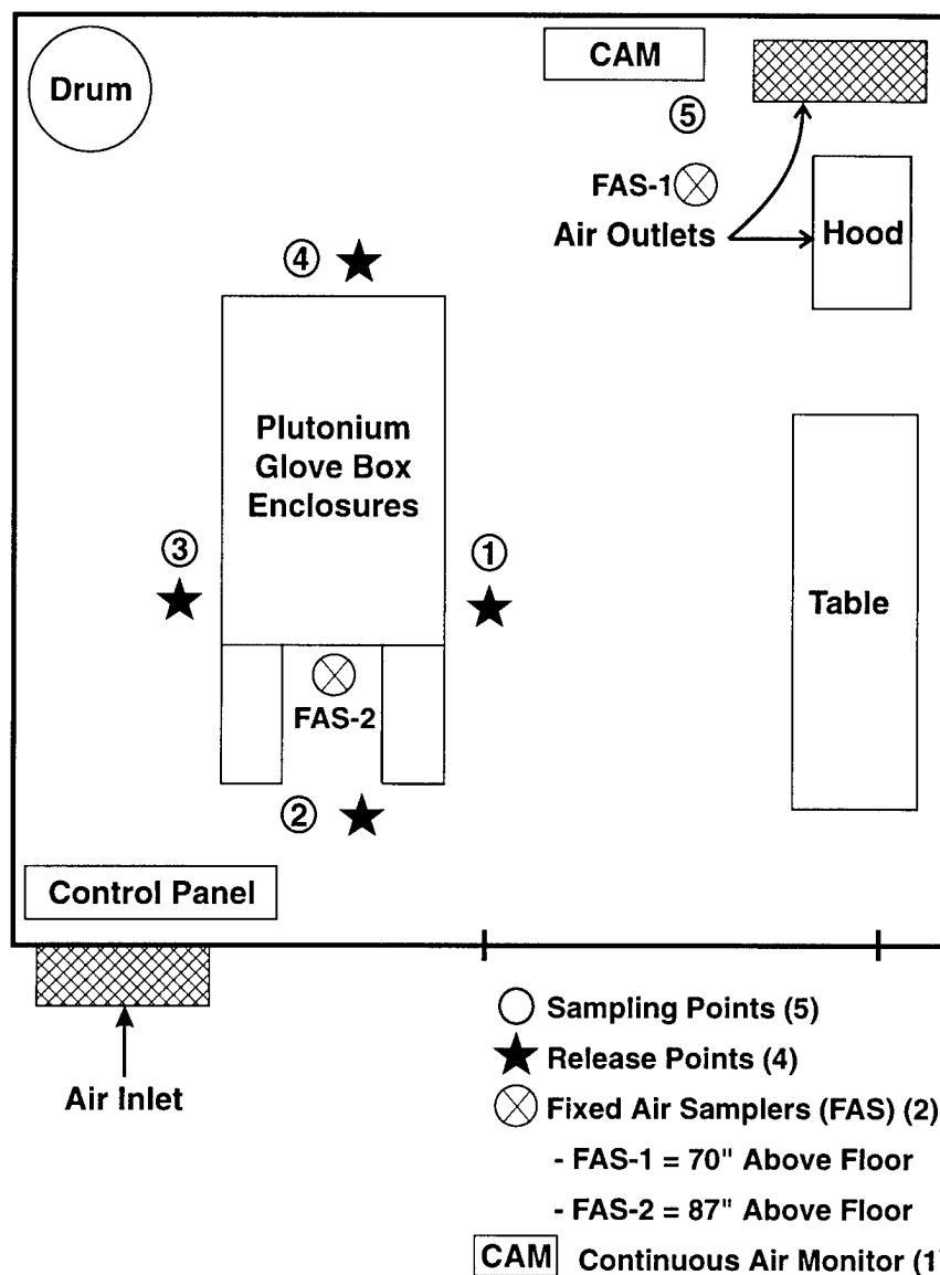
Figure 1. Sketch of the inhalation exposure test room showing the five sampling points and the four points for release of \text{SF}_6 . Inlet air passed through a 20" x 24" filter, 12" above the floor. Exhaust exited through a 20" x 24" filter, 85" above the floor.
