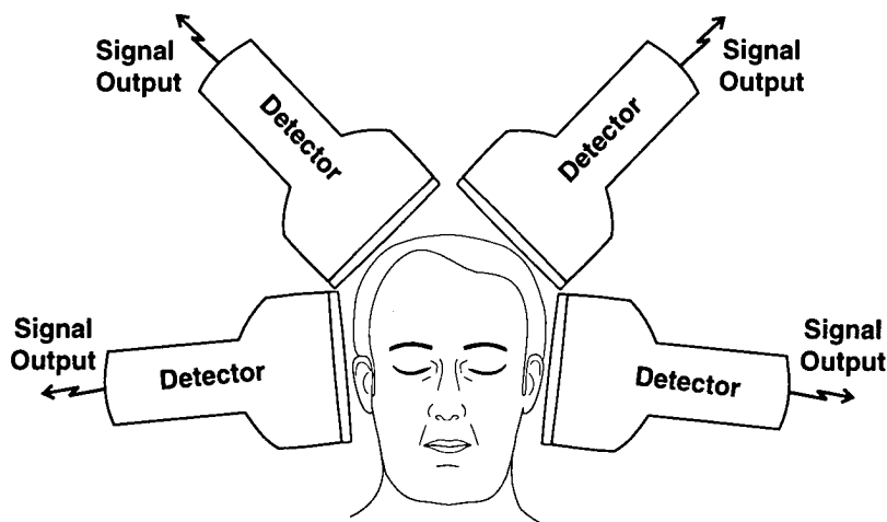
Figure 1. Detector positioning geometry for measuring ^{210}\text{Pb} in vivo .
