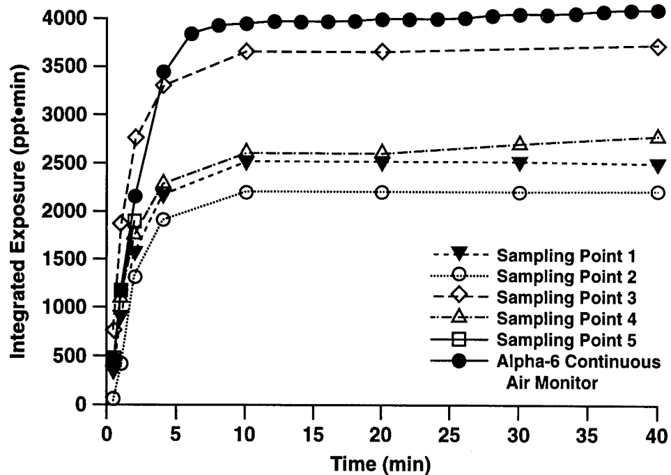
Figure 2. Graph of the integrated exposure, \Sigma(\text{ppt} \times \text{min}) , concentration of \text{SF}_6 measured at the various sampling points in the test room after release of \text{SF}_6 at position 2.
