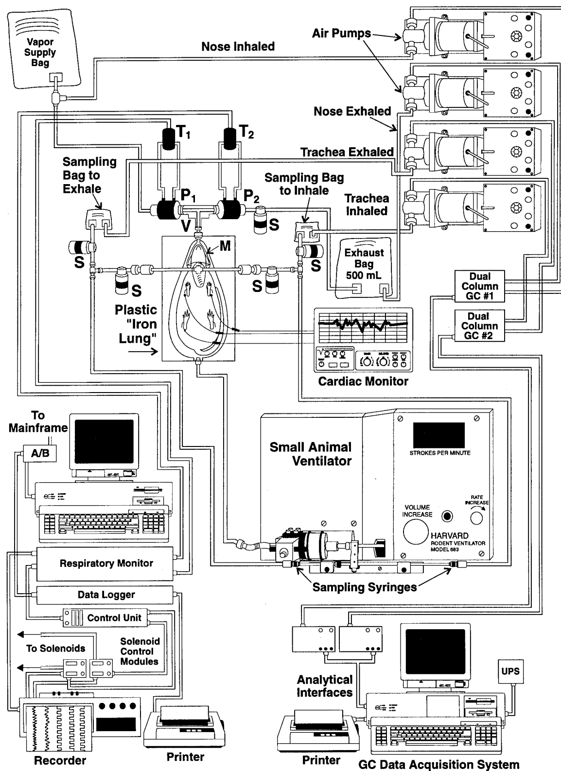
Figure 1. Schematic of the exposure system.
