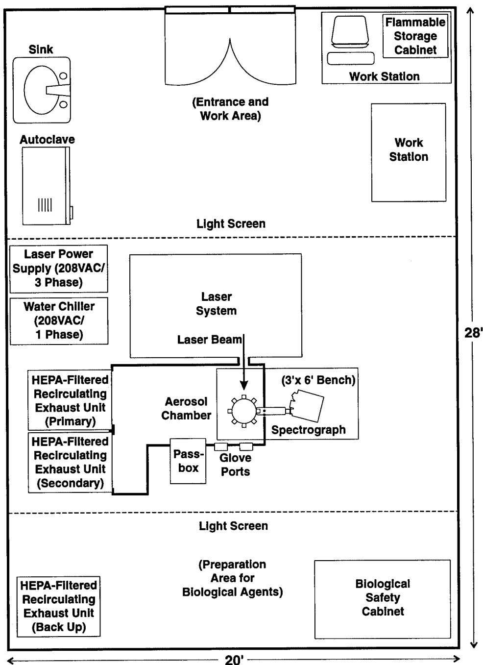
Figure 1. Floor plan of the ITRI Biosafety Level II Laboratory for testing of the SNL laser-based, real-time instrument for rapid detection of biological aerosols.
