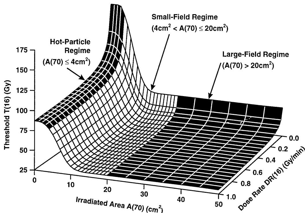
Figure 1. Response-surface for the beta radiation threshold (in Gy) for moist desquamation in skin as a function of irradiated area, A(70) in \text{cm}^2 , and the absorbed dose rate, DR(16) in Gy. For \beta radiation, equivalent doses and equivalent dose rates will be identical to the indicated absorbed doses and dose rates, respectively.
