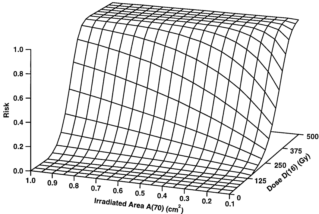
Figure 2. Risk surface for acute ulceration as a function of the irradiated area, A(70) in cm 2 , and absorbed dose, D(16) in Gy. Corresponding equivalent doses will be identical to D(16) .
