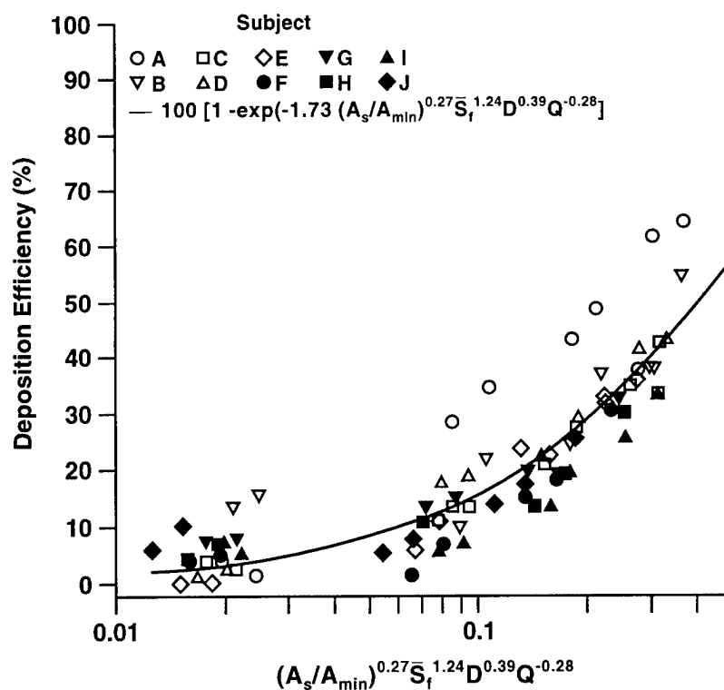
Figure 1. Nasal (nasal-pharyngeal-tracheal) deposition during inspiration as a function of a geometry-related diffusion parameter. The solid line is the best-fitting equation from the MIXNLIN procedure.
