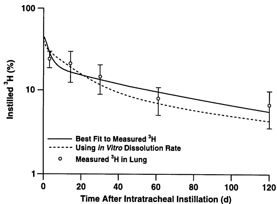
Figure 2. Retention of tritium in the rat lung after intratracheal instillation of titanium tritide particles. Experimental data (mean and standard deviation) are compared to results of a simulation model using (1) best-fit parameters for the measured ^3\text{H} retention and (2) the dissolution rate parameter from a previous in vitro study.
