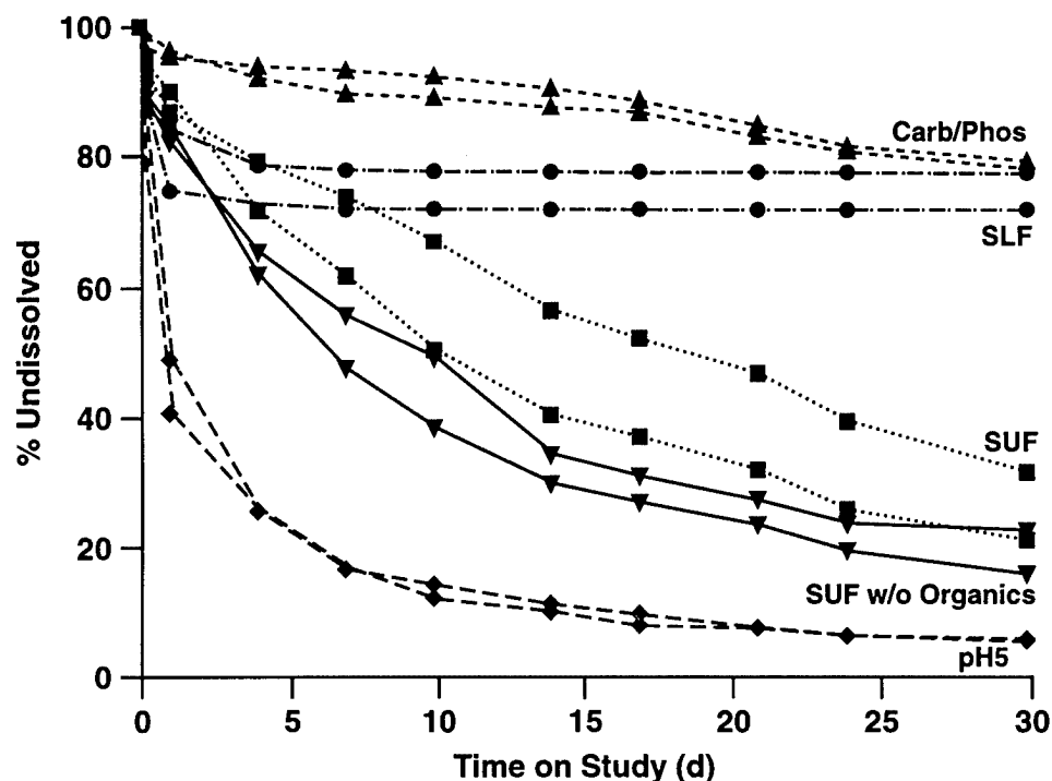
Figure 1. Dissolution of U_3O_8 uranium mill product in different solvent systems.
