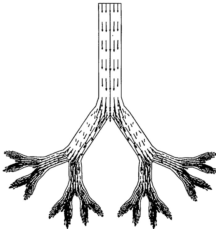
Figure 2. Illustration of the computed flow velocity vectors on the central bifurcation plane of the fluid dynamics model of the human lung (flow condition of Re = 700 ).
