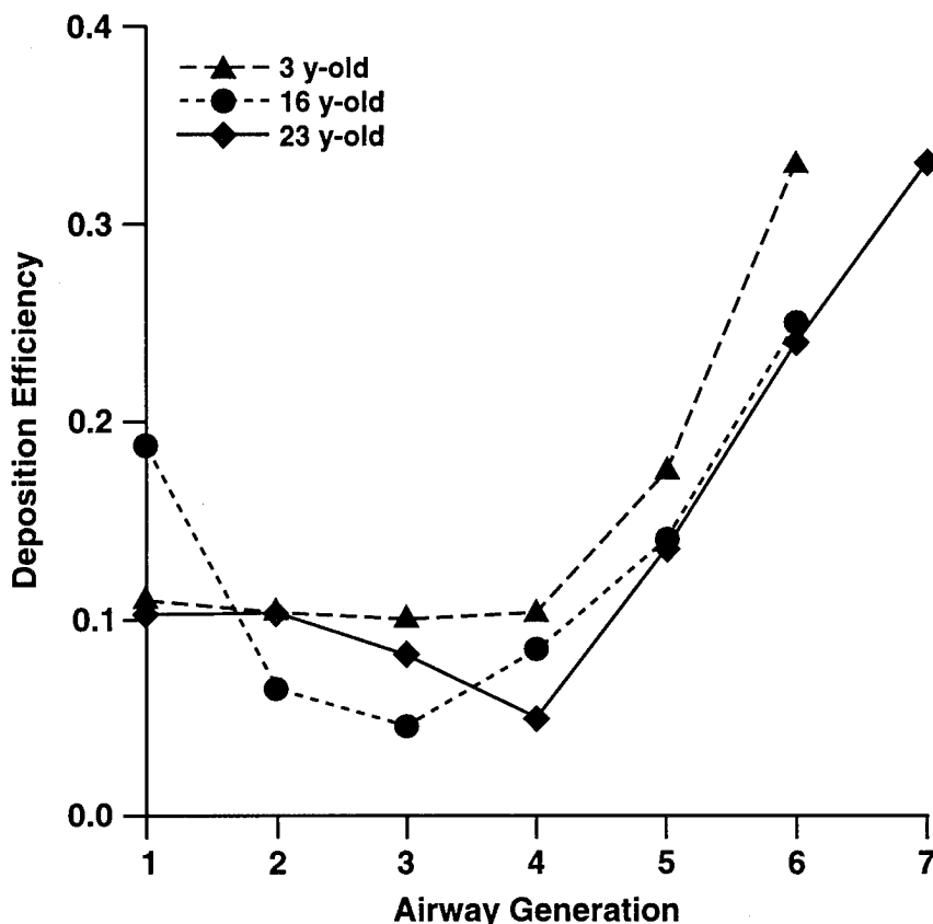
Figure 2. Average deposition by airway generation during inhalation at rest for 1.7 nm particles in the morphological models of humans. (Trachea is generation 1, main bronchi are generation 2, and so on.)
