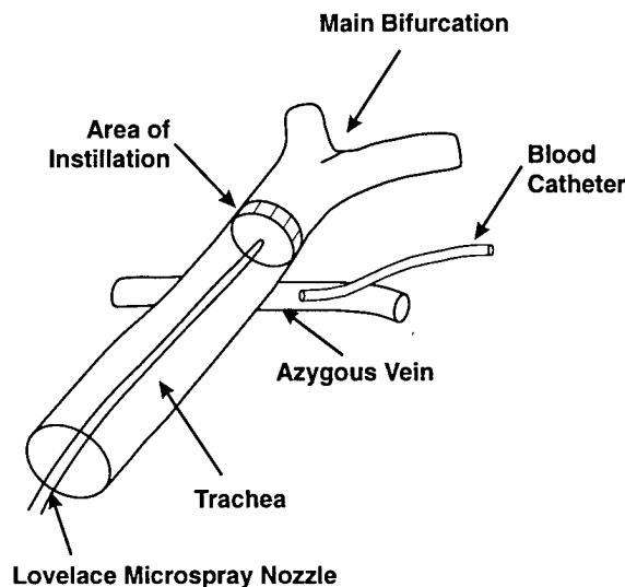
Figure 1. Schematic of the area of instillation in the distal trachea, including the location of the blood catheter in the azygous vein.
