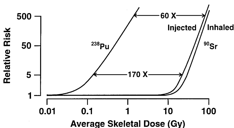
Figure 1. Estimates of the relative risk in a proportional hazards model for bone cancer in dogs that inhaled ^{238}\text{PuO}_2 , dogs that inhaled ^{90}\text{SrCl}_2 , and in dogs injected with ^{90}\text{Sr} . The increase in average skeletal dose for a relative risk of 5 and 500 between inhaled ^{238}\text{PuO}_2 and injected ^{90}\text{Sr} is shown.
