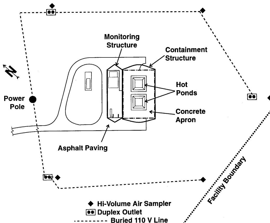
Figure 1. Layout of the ITRI hot pond site, showing the location of the concrete ponds, the containment and monitoring structures, and the perimeter air monitoring system.
