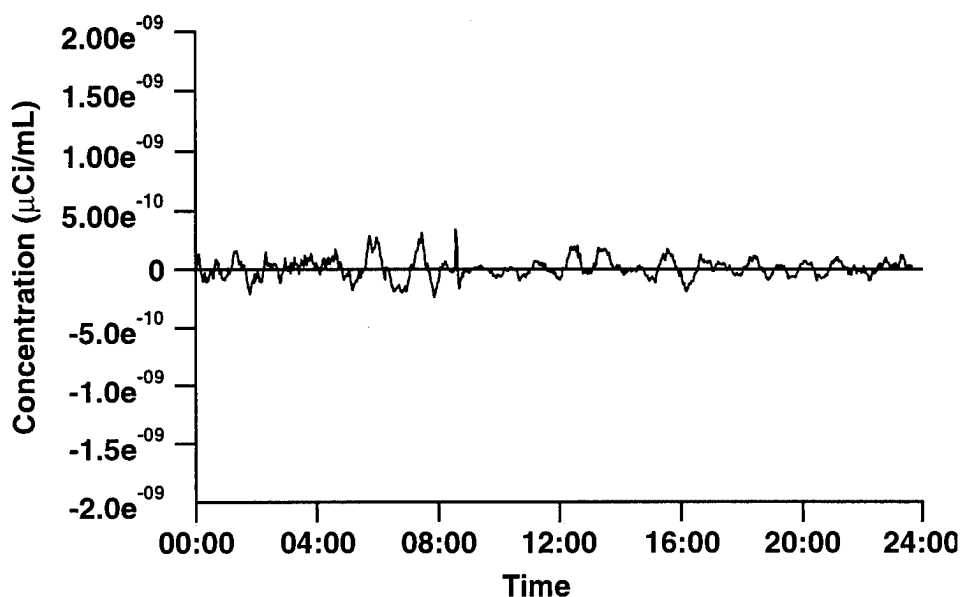
Figure 2. Graph of the workplace air concentration of beta-emitting radionuclides detected by the AMS-4 continuous air monitor during removal of contaminated concrete at the ITRI hot pond site. The alarm set point was 8.0 \times 10^{-8} \mu\text{Ci/mL} .
