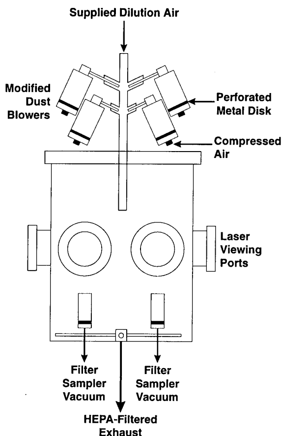
Figure 2. Schematic diagram of the modified dust blower system and the aerosol test chamber for laser-based detection of biological agents.
