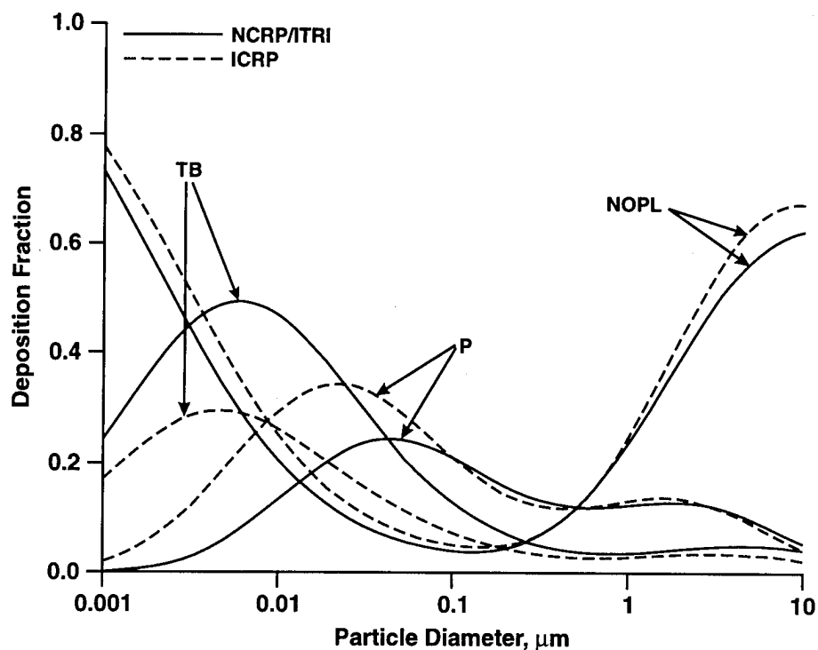
Figure 2. Comparison between the NCRP/ITRI and ICRP66 models for deposition of inhaled polydisperse aerosols ( \sigma_g = 2.5 , particle density = 1.0 \text{ g/cm}^3 , tidal volume = 770 mL, breathing frequency = 13/min, functional residual capacity = 3000 mL). TB = tracheobronchial; P = pulmonary; NOPL = naso-oro-pharyngo-laryngeal.
