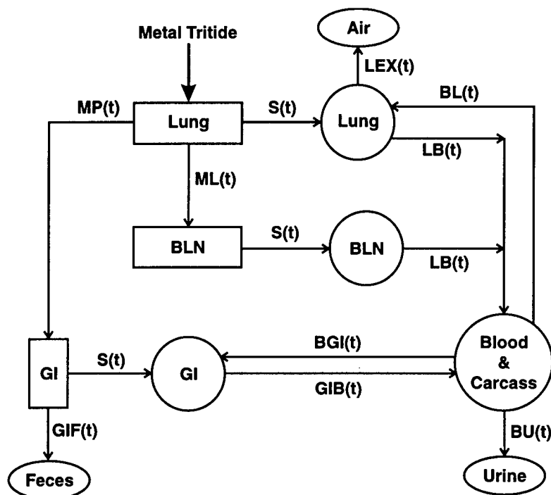
Figure 1. Schematic diagram of a metabolic simulation model of distribution and clearance of metal tritides in rats.
