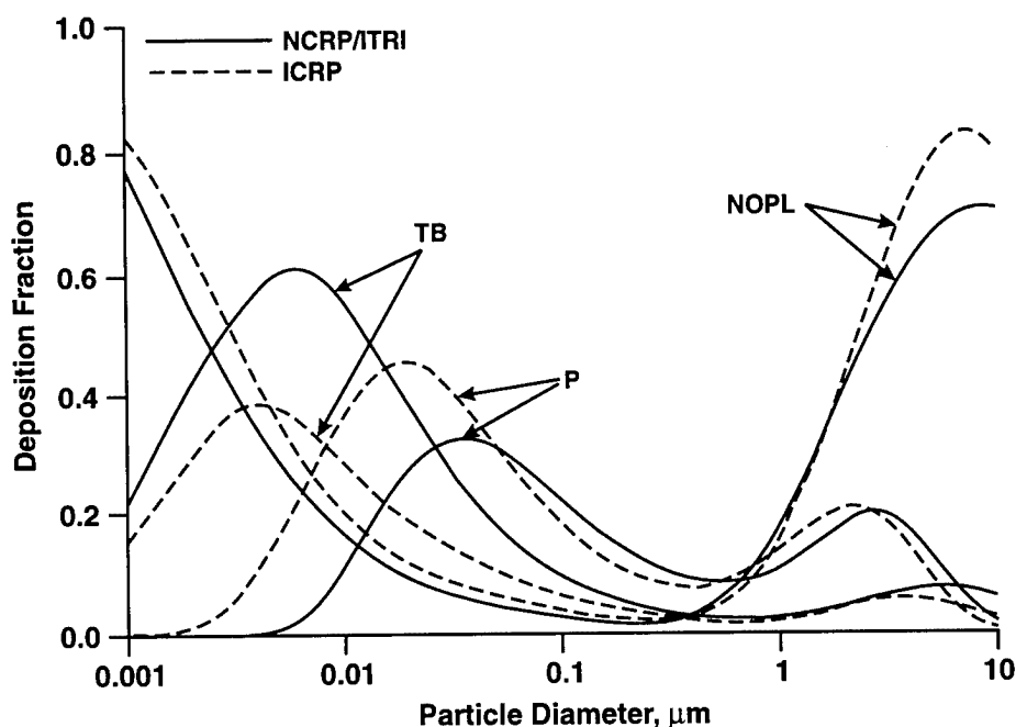
Figure 1. Comparison between the NCRP/ITRI and ICRP66 models for deposition of inhaled monodisperse aerosols ( \sigma_g = 1.0 , particle density = 1.0 \text{ g/cm}^3 , tidal volume = 770 mL, breathing frequency = 13/min, functional residual capacity = 3000 mL). TB = tracheobronchial; P = pulmonary; NOPL = naso-oro-pharyngo-laryngeal.
