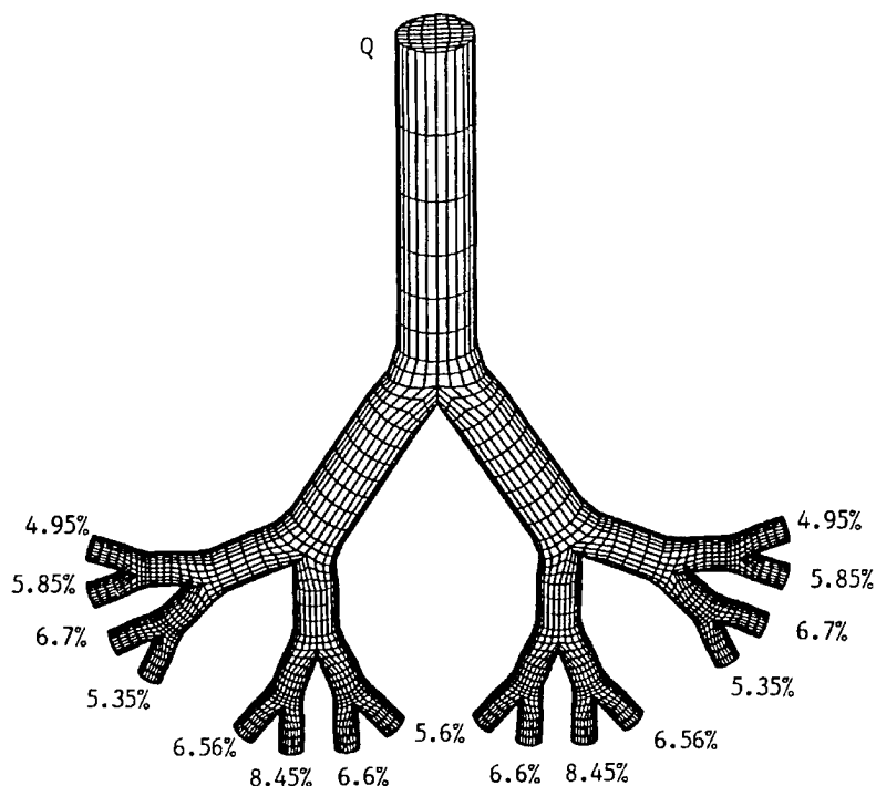
Figure 1. Illustration of the finite element mesh used in the three-dimensional fluid dynamics model of the human tracheobronchial tree. The calculated distribution of flow rates through the airways is also shown.
