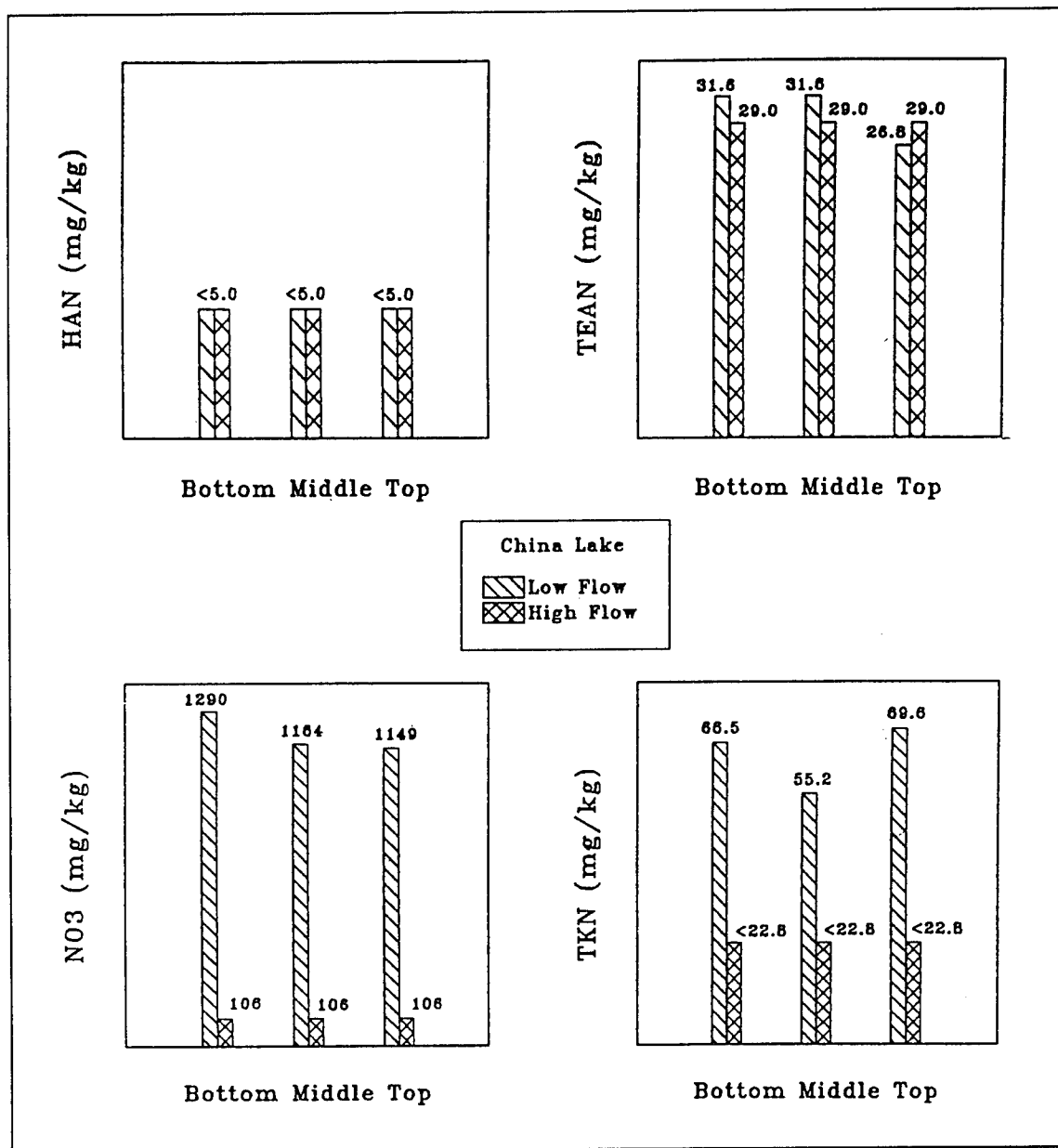
Figure 11. Residual concentrations of HAN, TEAN, NO 3 , and TKN in China Lake soil after completion of washing (Concentrations are milligrams per kilogram of wet soil)
