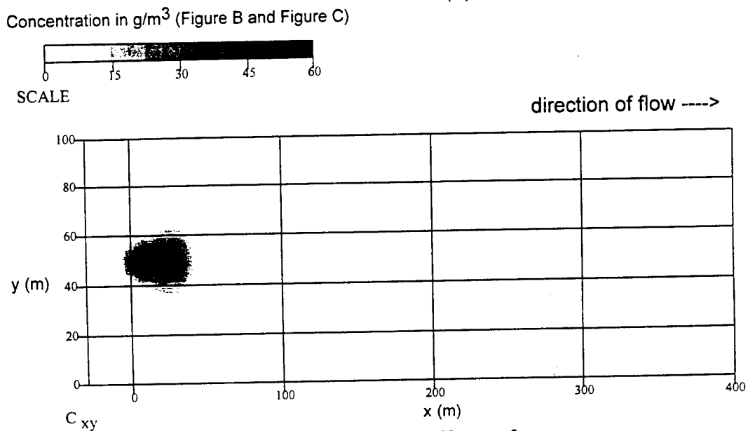
B. Top view of aquifer surface.
