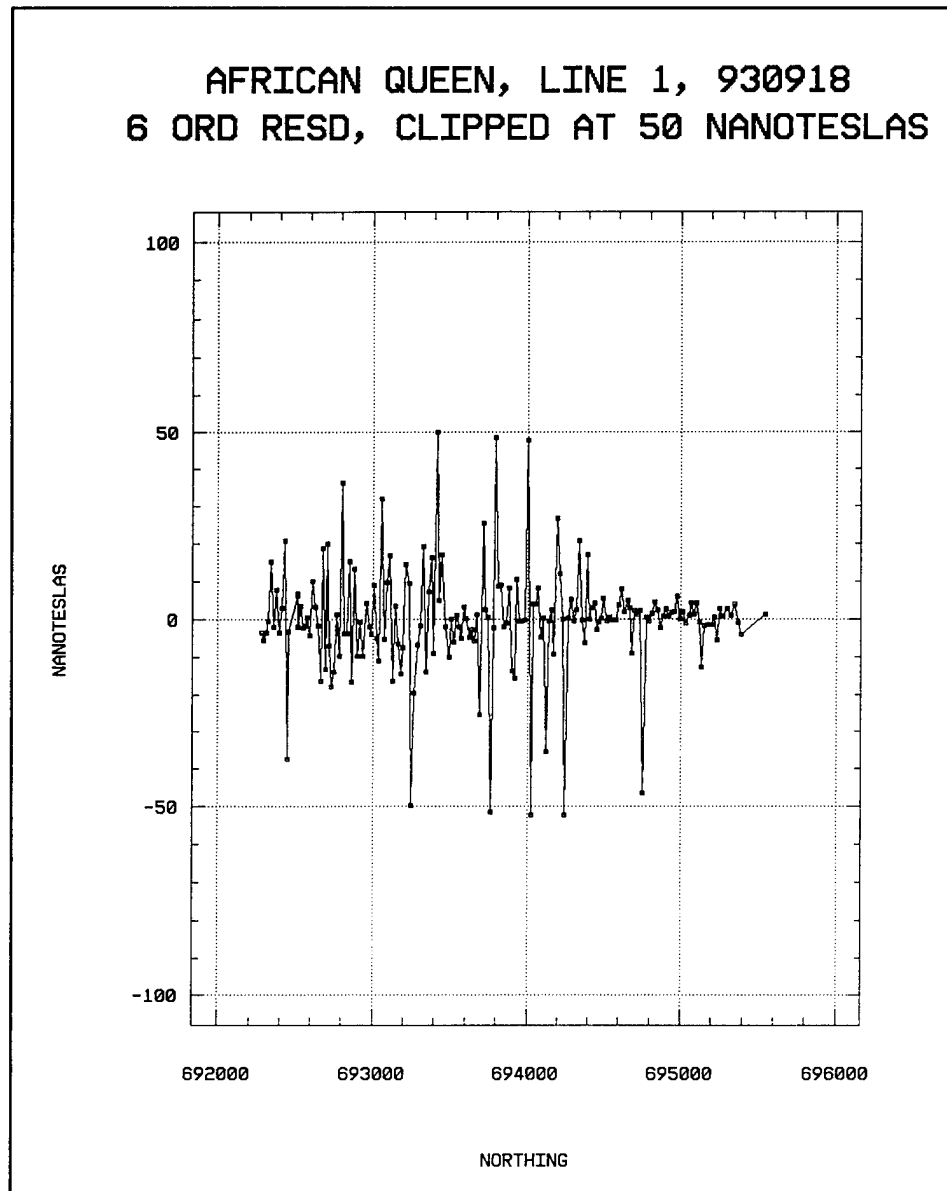
Figure 28. Total field magnetic data from the R/V African Queen Line I. Data are diurnal drift corrected, regional effects removed, and responses clipped above \pm 50 nanoTeslas
