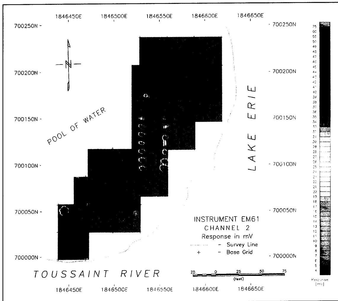
Figure 15. EM-61 response from inert ordnance items buried on the Toussaint River spit test site
