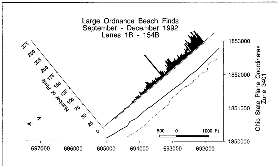
Figure 59. EODT large ordnance beach finds, September-December 1992 data for Lanes 1B-154B
