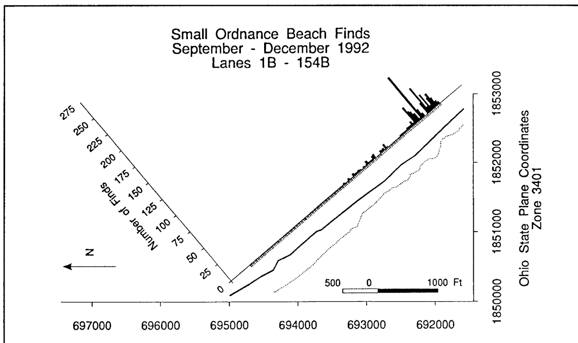
Figure 60. EODT small ordnance beach finds, September-December 1992 data for Lanes 1B-154B
