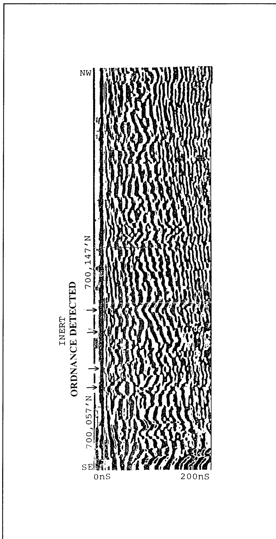
Figure 41. Longitudinal 100-MHz profile over sand spit, Line 1,846,555 , with inert ordnance buried between 87'N and 147'N
