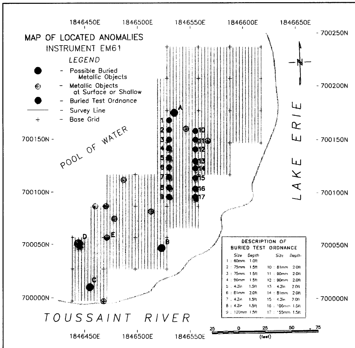
Figure 14. Inert ordnance items buried on the Toussaint River spit test site
