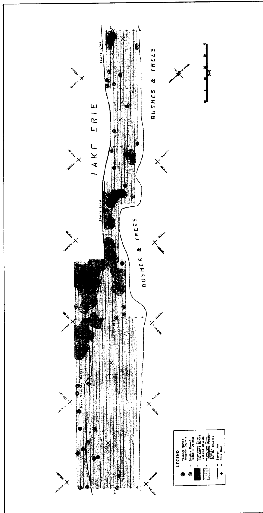
Figure 19. EM-61 anomalies located on East Beach from all collected channels of data
