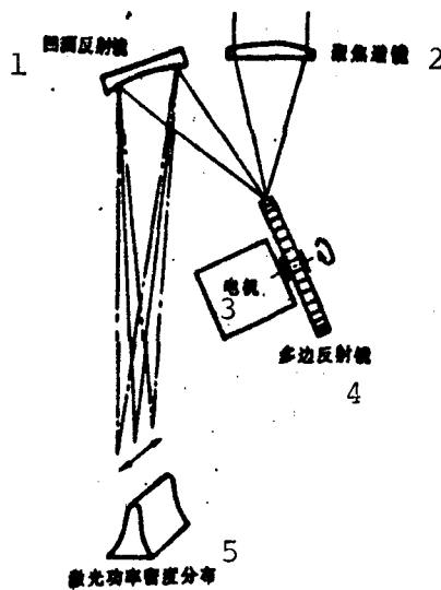
Fig. 2. Polygonal reflective mirror scanning system KEY: 1 - concave surface reflective mirror 2 - focusing lens 3 - electric motor 4 - polygonal reflective mirror 5 - distribution of laser power density
