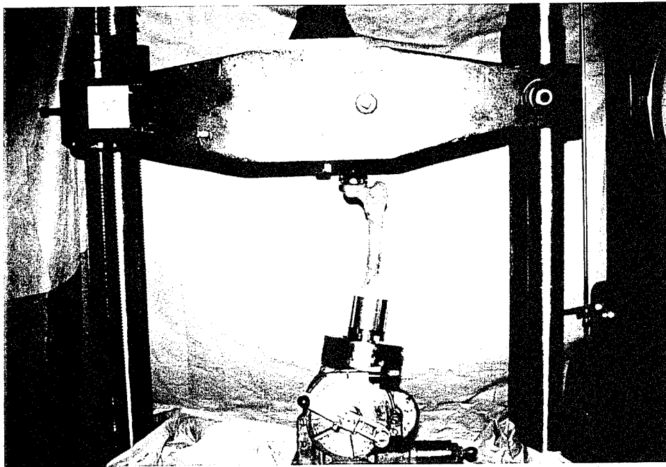
Figure 3: Femur in Universal Testing Machine.
