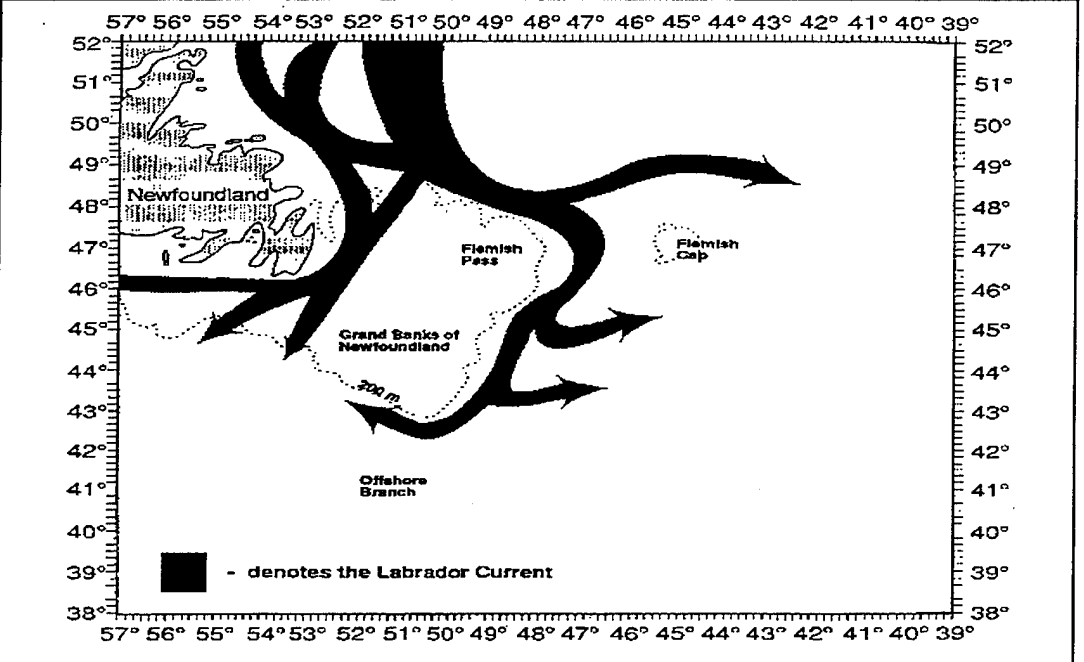
Figure 2. The Labrador Current in the IIP operating area in the North Atlantic. From Ref. (U.S. Coast Guard, 1991).
