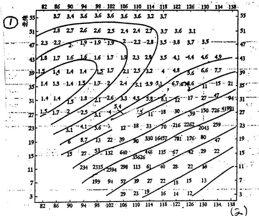
Fig.2 Distribution Chart for Nanjing-Kunming Synchronous Observation \sigma_{\Delta\lambda}^2 ( i = 90\frac{1}{2}, H = 3500 kilometers)
