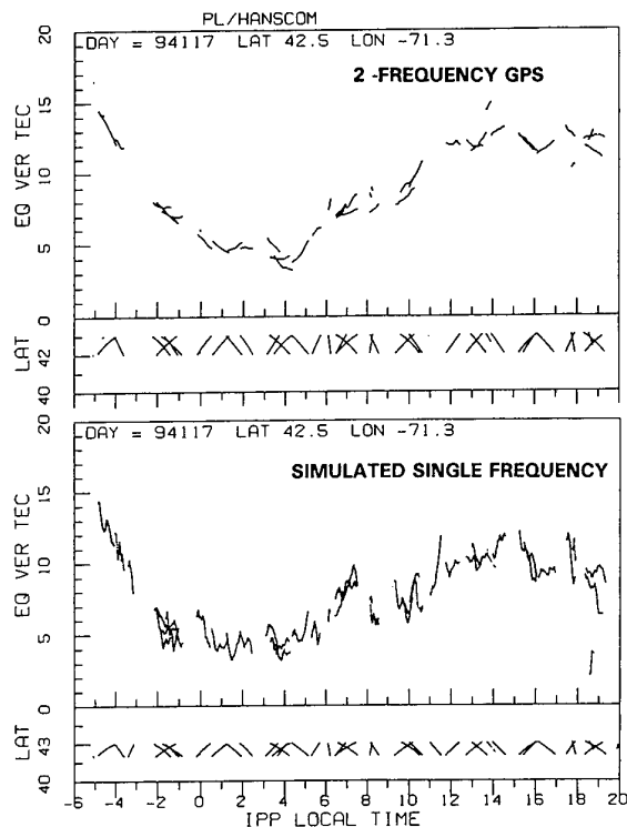
Figure 13. Comparison of simulated GPS single-frequency TEC measurements (derived using a new technique based on ionospheric self-calibration) to GPS two-frequency TEC results.
