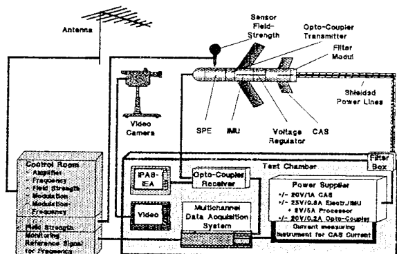
Figure 4.1-2: Test Setup
