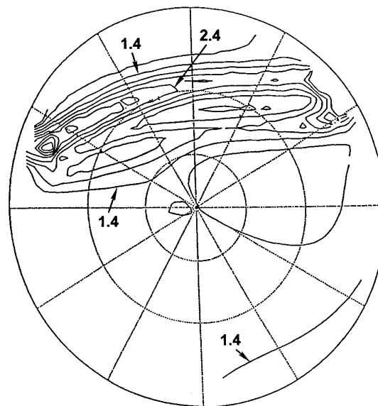
Figure 14. Example of a sky map of the impact of the ionospheric trough region on range error corrections from a model. In the middle of the trough the correction is too great by a factor of > 2.4 .
