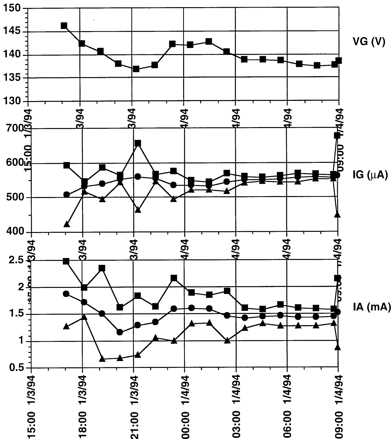
Figure 3: Lifetime test for 232,230-tip array of 4 μm column emitters with 6 μm tip-to-tip spacing. Upper chart shows corrected gate potential in volts. Center chart shows gate current in microamps, and the lower chart shows anode current in milliamps. These two charts show the mean and +/- 3 standard deviation values of the measured current.
