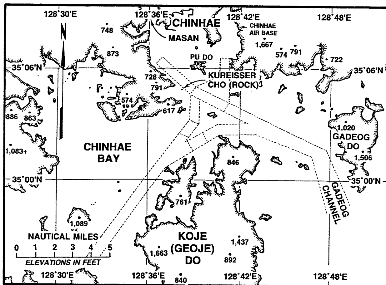
Figure VII-27. Approaches to Chinhae harbor.
