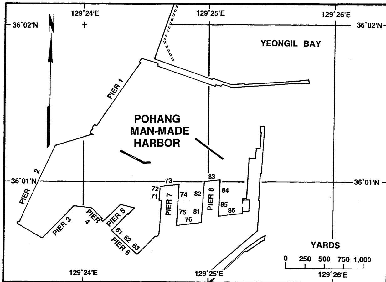
Figure VII-39. Pohang Harbor.
