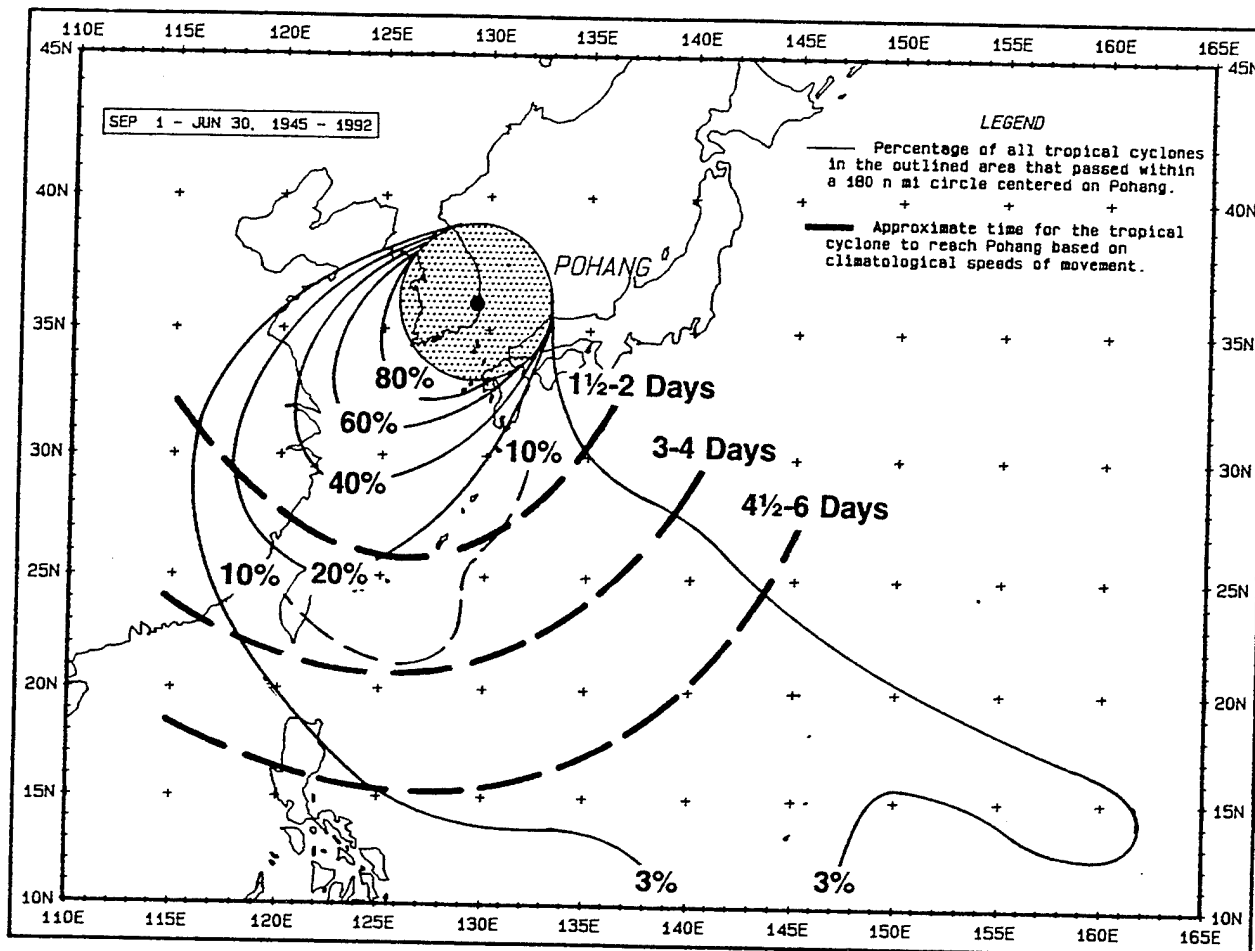
Figure VII-45. Probability that a tropical storm or typhoon will pass within 180 nmi of Pohang (circle), and approximate time to closest point of approach, during the period September through June.
