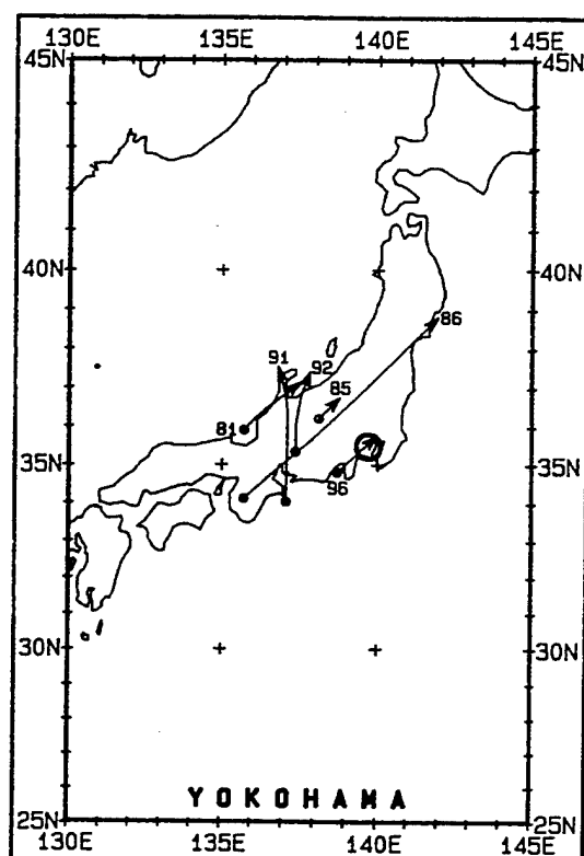
Figure V-208. Track segments of the six tropical storms or typhoons causing sustained winds of at least 34 kt at Yokohama or Tokyo International Airport during the 20-year period 1973-1992. The numbers shown correspond to the index numbers listed in Table V-48.
