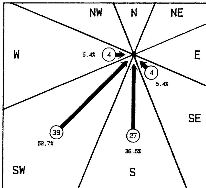
Figure VII-32. Directions of approach for the 74 tropical cyclones passing within 180 nmi of Chinhaie during the 48-year period of record.
