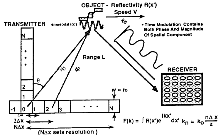
Figure 5: Fourier Telescopey Concept
