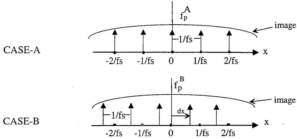
Figure IV.4. Two Different Cases for Sampling Points
