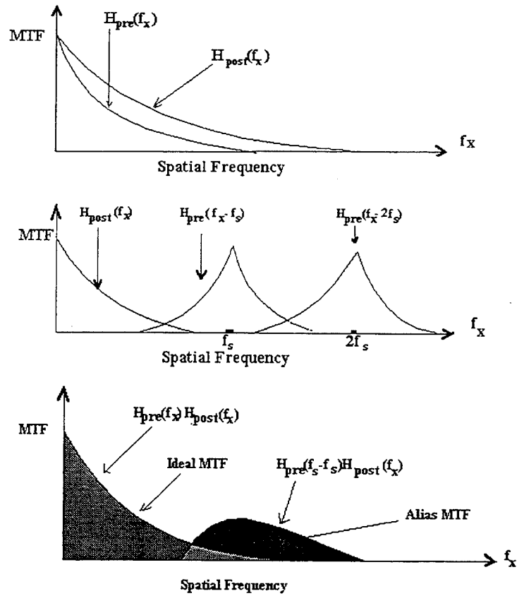
Figure IV.2. Presentation of Aliasing by Using MTF
