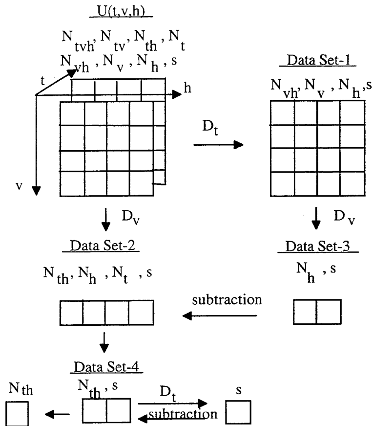
Figure B.1. Application of D Operator
