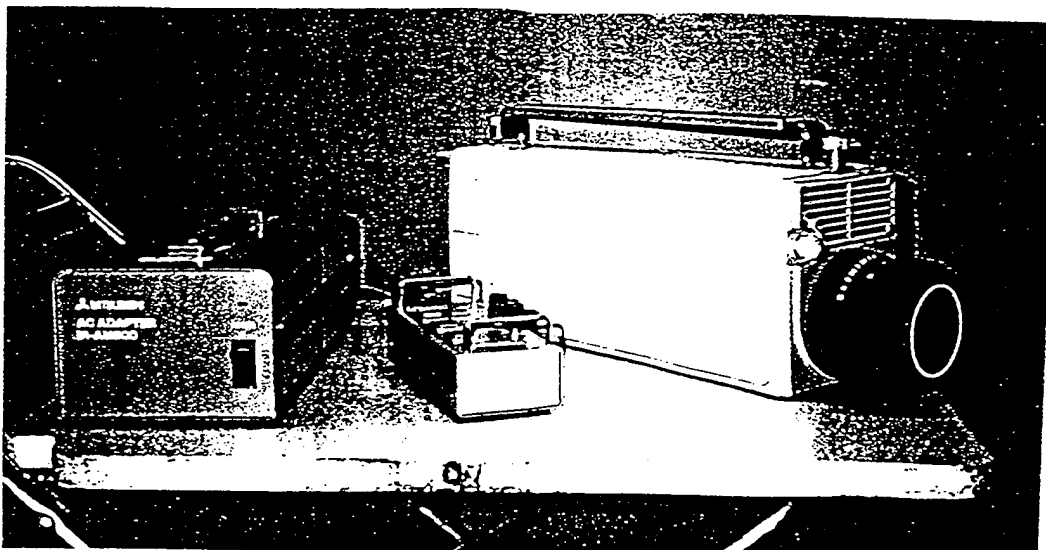
Figure V.3. Mitsubishi IR-M500 Thermal Imager
