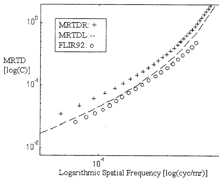
Figure II.3. Logarithmic Presentation of MRTD Models
