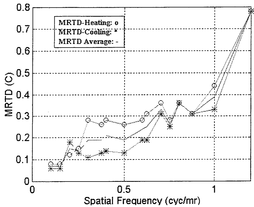
Figure C.3. Mitsubishi System Measured MRTD h
