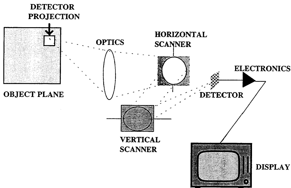
Figure I.2. A Simplified Scanning TIS ( From Ref.1 )
