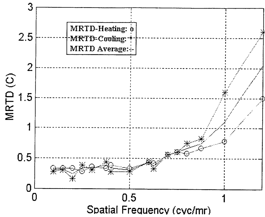
Figure C.1. Amber System Measured MRTD h
