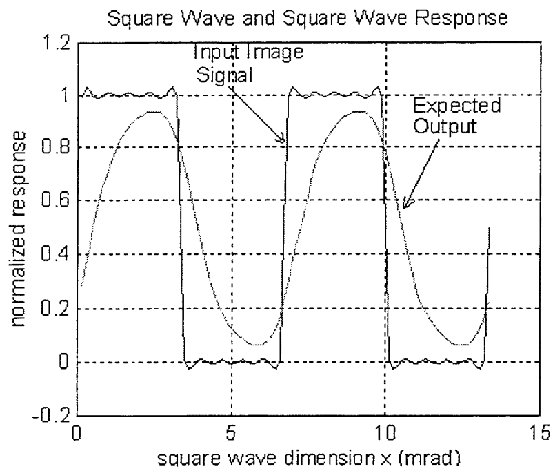
Figure IV.5. Square Wave Image Signal and Expected Image Output Signal ( After Ref. [8] )
