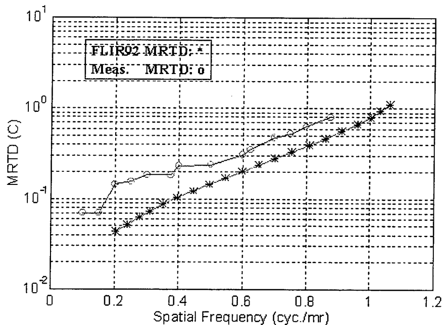
Figure VI.6. Logarithmic Comparison of the FLIR92 MRTD to the Measured MRTD for Mitsubishi System
