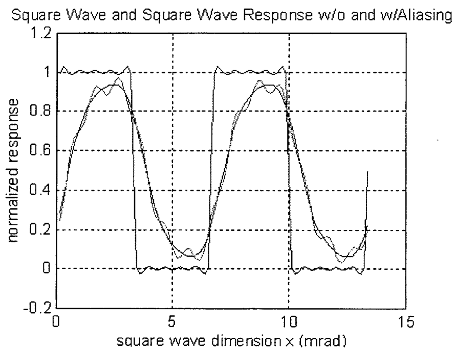
Figure IV.8. Square Wave Image Signal, Expected Image Output
