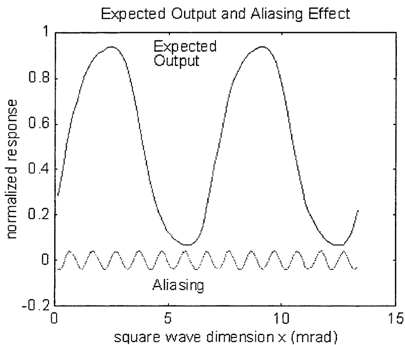
Figure IV.6. Expected Image Output Signal and Aliasing
