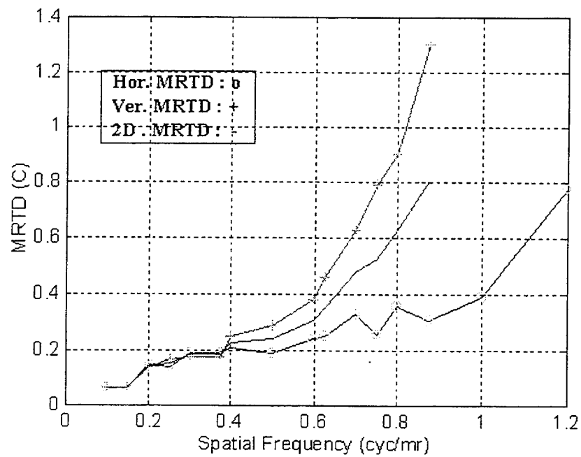
Figure V.6. MRTD Measurements for Mitsubishi IR-M500 Thermal Imager
