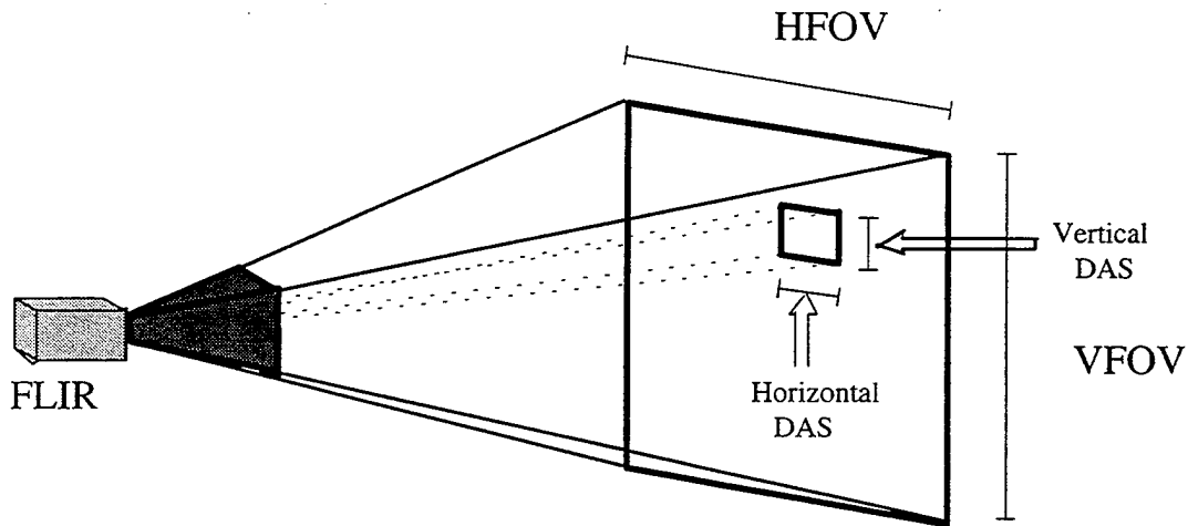
Figure I.3. Detector Angular Subtense ( From Ref. 1)
