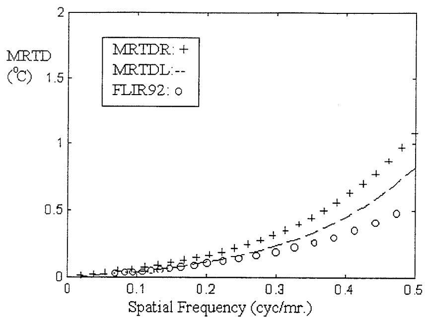
Figure II.2. Ratches, Lloyd, and FLIR92 MRTD Models
