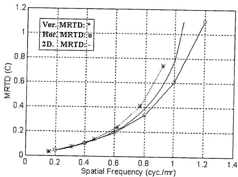
Figure. VI.4. FLIR92 MRTD Values for Mitsubishi System
