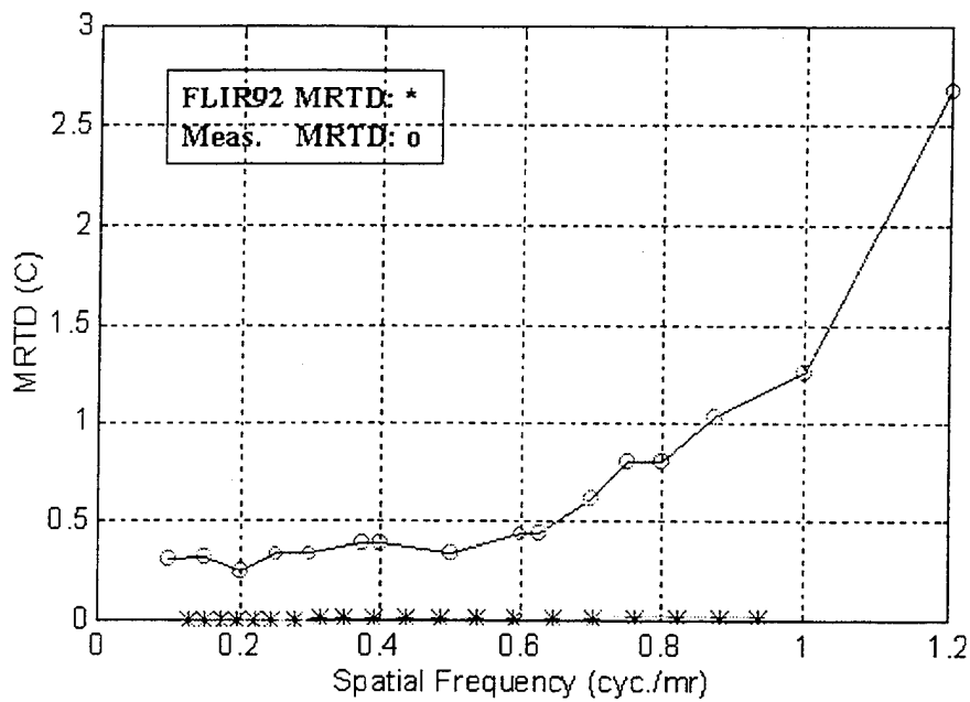
Figure VI.2. Comparison of the FLIR92 MRTD to the Measured MRTD for Amber System
