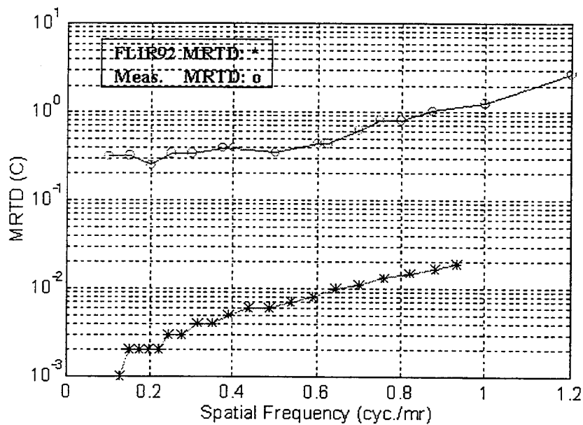
Figure VI.3. Logarithmic Comparison of the FLIR92 MRTD to the Measured MRTD for Amber System
