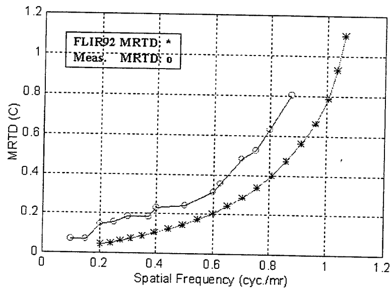
Figure VI.5. Comparison of the FLIR92 MRTD to the Measured MRTD for Mitsubishi System
