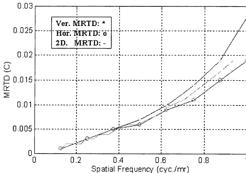
Figure VI.1. FLIR92 MRTD Values for Amber System
