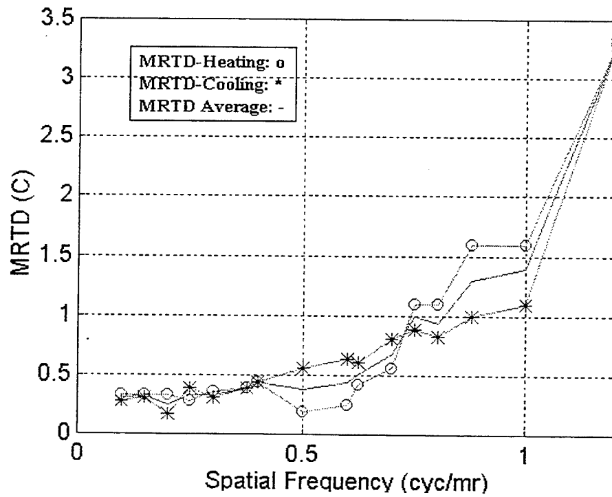
Figure C.2. Amber System Measured MRTD v
