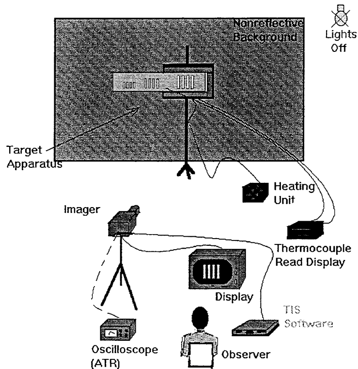
Figure V.1. Laboratory Setup
