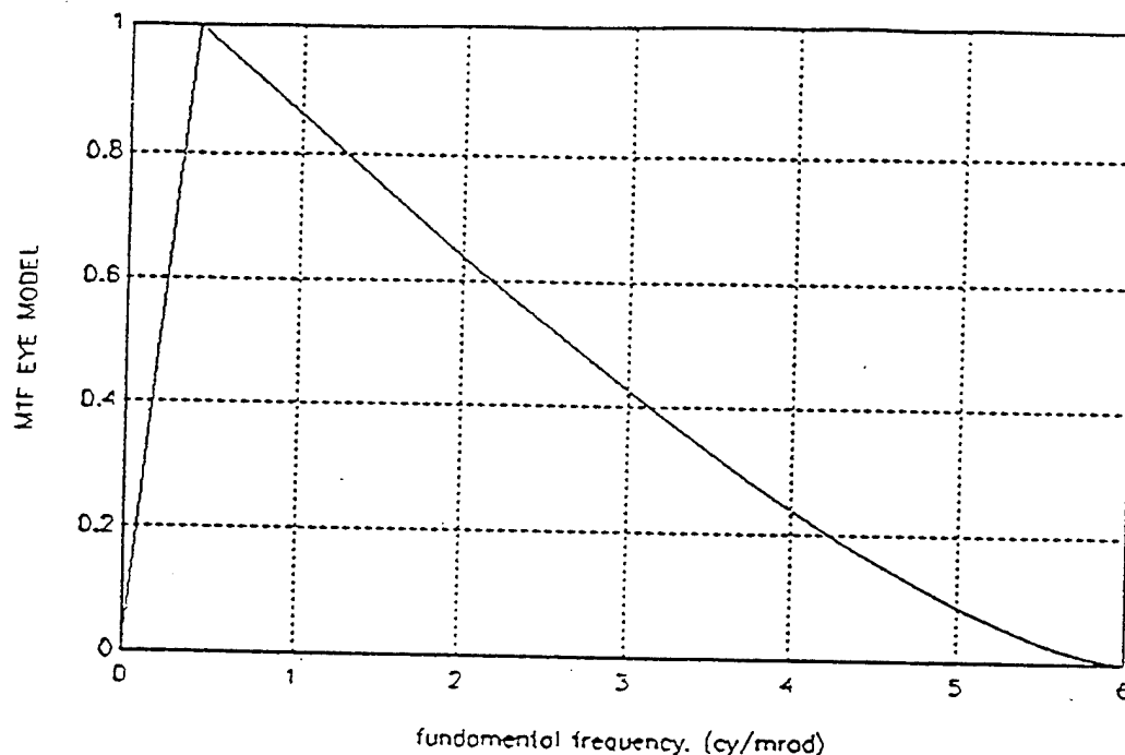
Figure I.1. A Simple Eye MTF Model ( From Ref.[8] )
