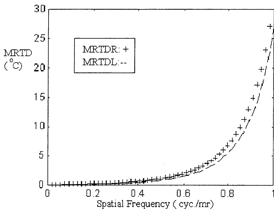
Figure II.1 Ratches and Lloyd MRTD Models
