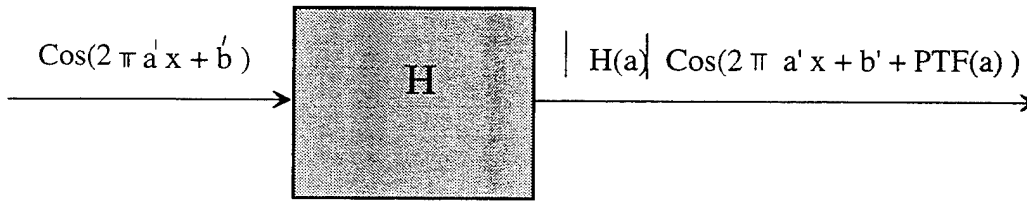
Figure IV.5. The H-Rule ( a' and b' are arbitrary constants)
