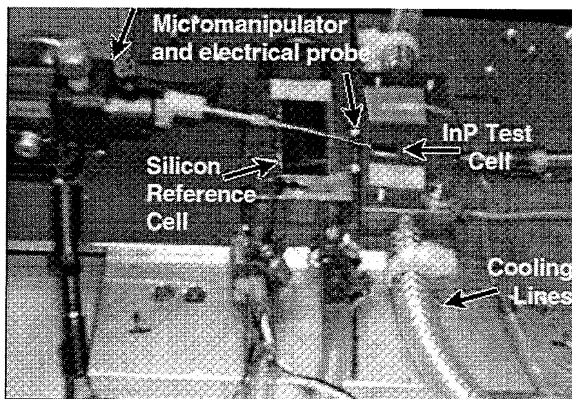
Figure 6. 2 Experimental Setup with both Reference and Test Cells affixed to Brass Test Stands. A Micromanipulator which Controls Placement of the Electrical Probe is Indicated as well as the Thermal Control Cooling Lines.
