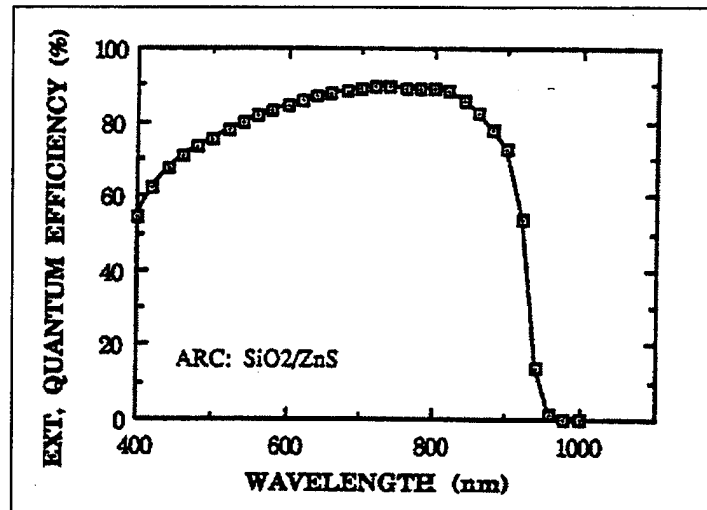
Figure 6. 1 Quantum Efficiency vs. Wavelength of Incident Light of the Nippon Mining InP Solar Cells used in this Research. [Ref. 33:p. 3]
