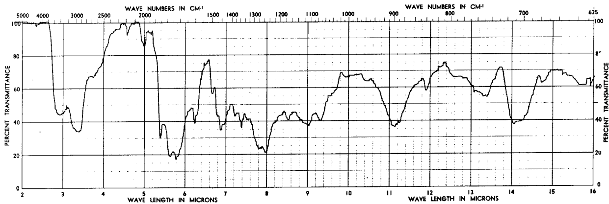
Figure 15. Polyester pyrolyzate
