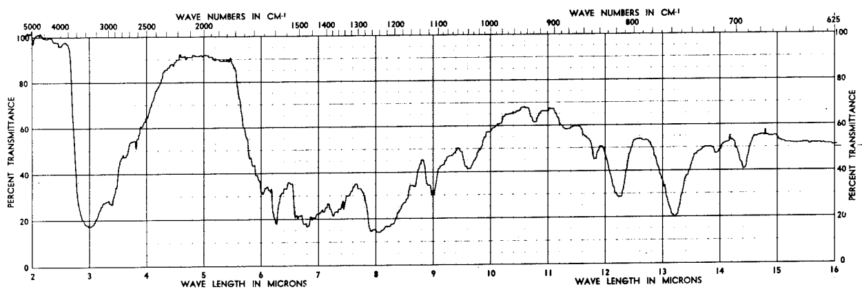
Figure 8. Phenolic pyrolyzate
