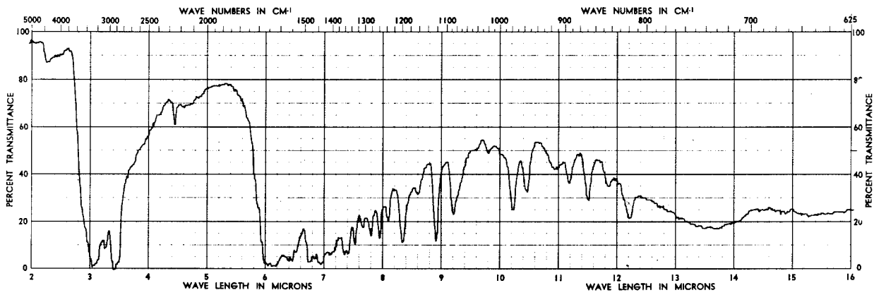
Figure 6. Polyamide film ("Capran") pyrolyzate
