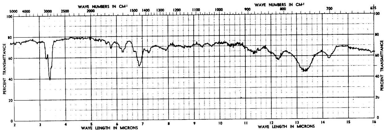
Figure 16. PVC pyrolyzate from ("Tygon") tubing extracted with methylethyl ketone and acetone
