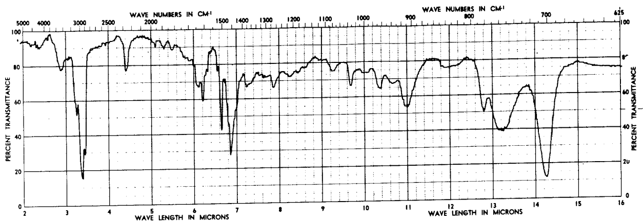
Figure 7. ABS pyrolyzate
