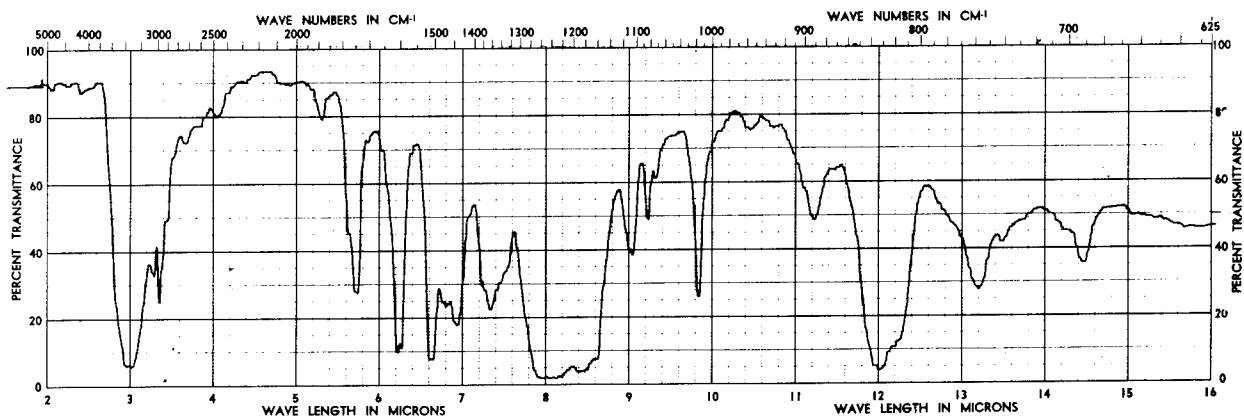
Figure 9. Polycarbonate pyrolyzate
