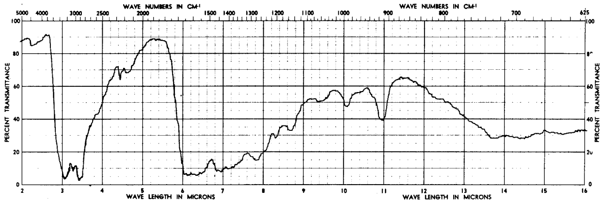
Figure 5. Nylon 6/6 pyrolyzate
