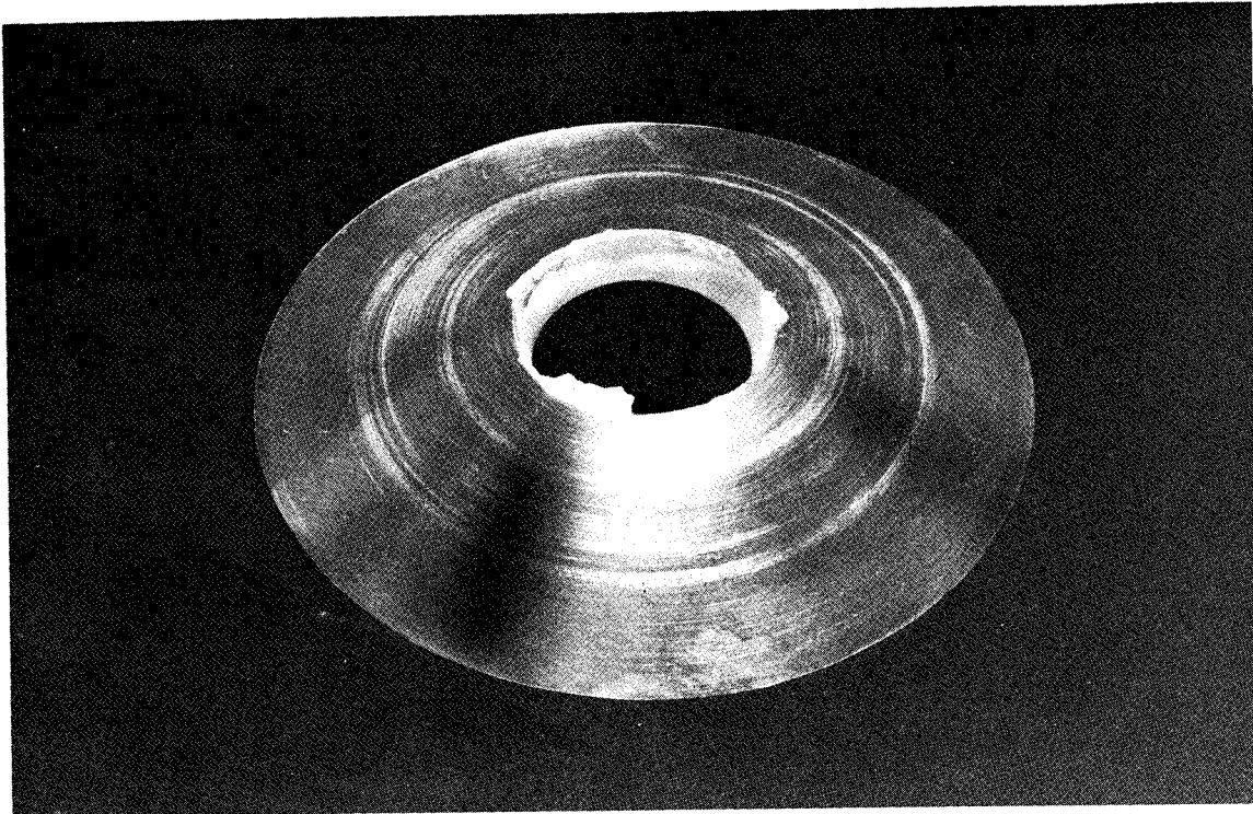
Figure B-36. Failed 1-inch-diameter, 150^\circ , 0.5 t/D ratio window, low-pressure face.
