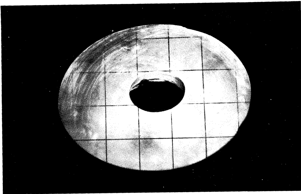
Figure B-37. Failed 1-inch-diameter, 150^\circ , 0.5 t/D ratio window, high-pressure face.
