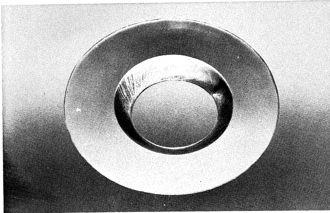
Figure B-24. Failed 1-inch-diameter, 120°, 0.625 t/D ratio window, high-pressure face.
