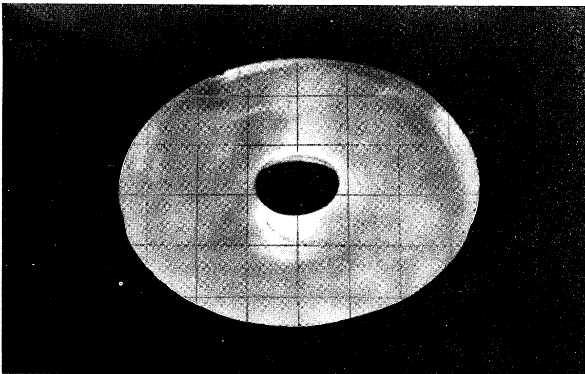
Figure B-39. Failed 1-inch-diameter, 150^\circ , 0.625 t/D ratio window, high-pressure face.
