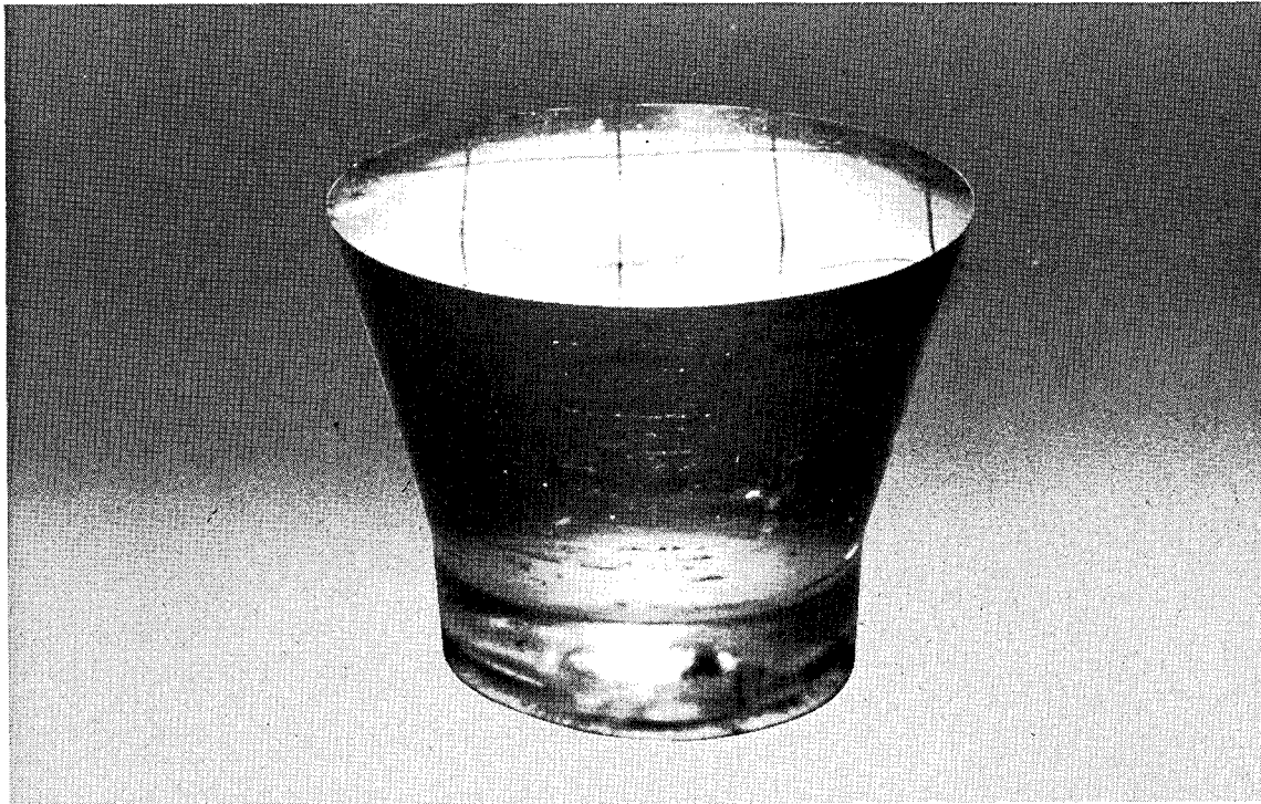
Figure B-1. Arrested failure of 1-inch-diameter, 30^\circ , 1.0 t/D ratio window at 24,000 psi, high-pressure face.
