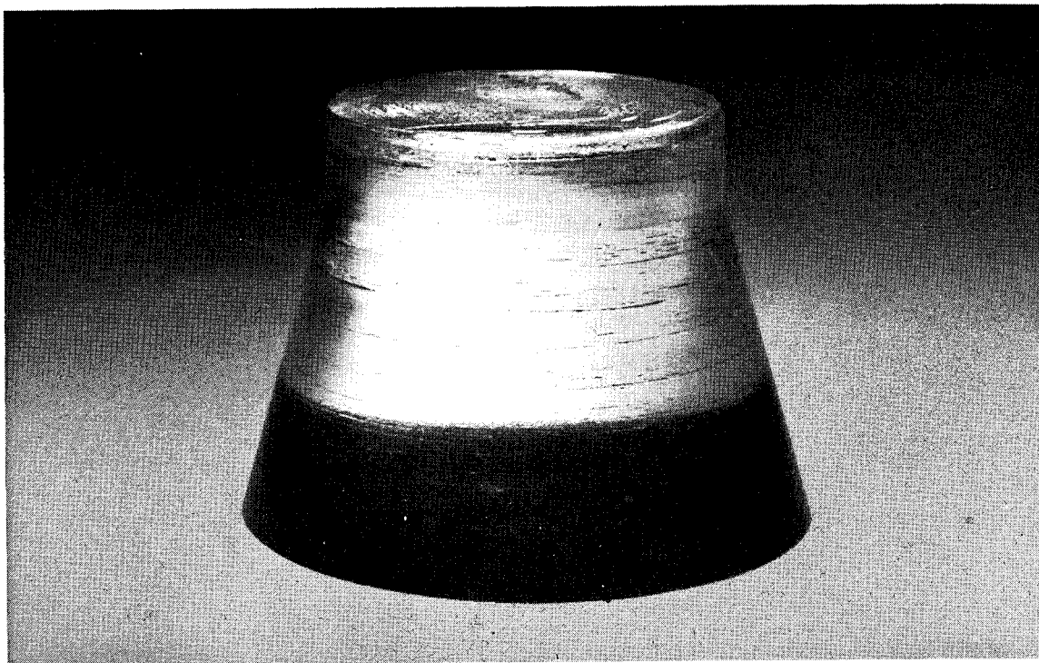
Figure B-2. Arrested failure of 1-inch-diameter, 30^\circ , 1.0 t/D ratio window at 24,000 psi, low-pressure face.
