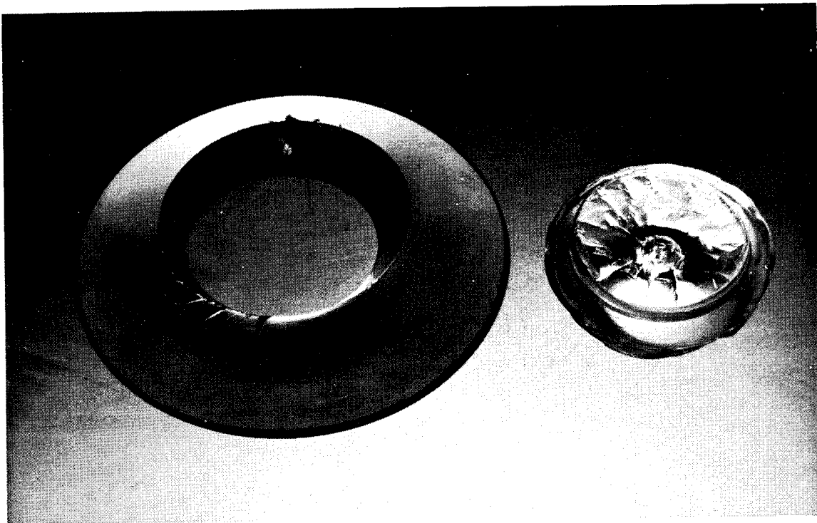
Figure B-25. Failed 1-inch-diameter, 120°, 0.5 t/D ratio window, low-pressure face, with center portion alongside.
