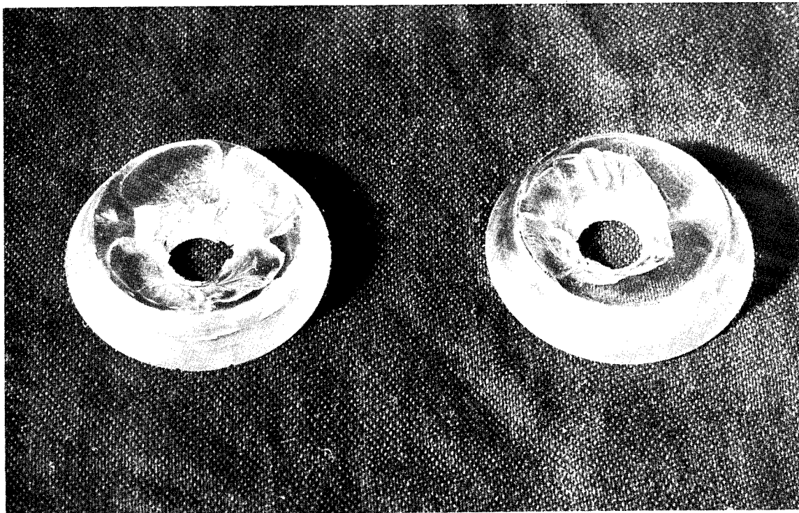
Figure B-3. Failed 1-inch-diameter, 60^\circ , 0.25 t/D ratio windows, low-pressure faces.
