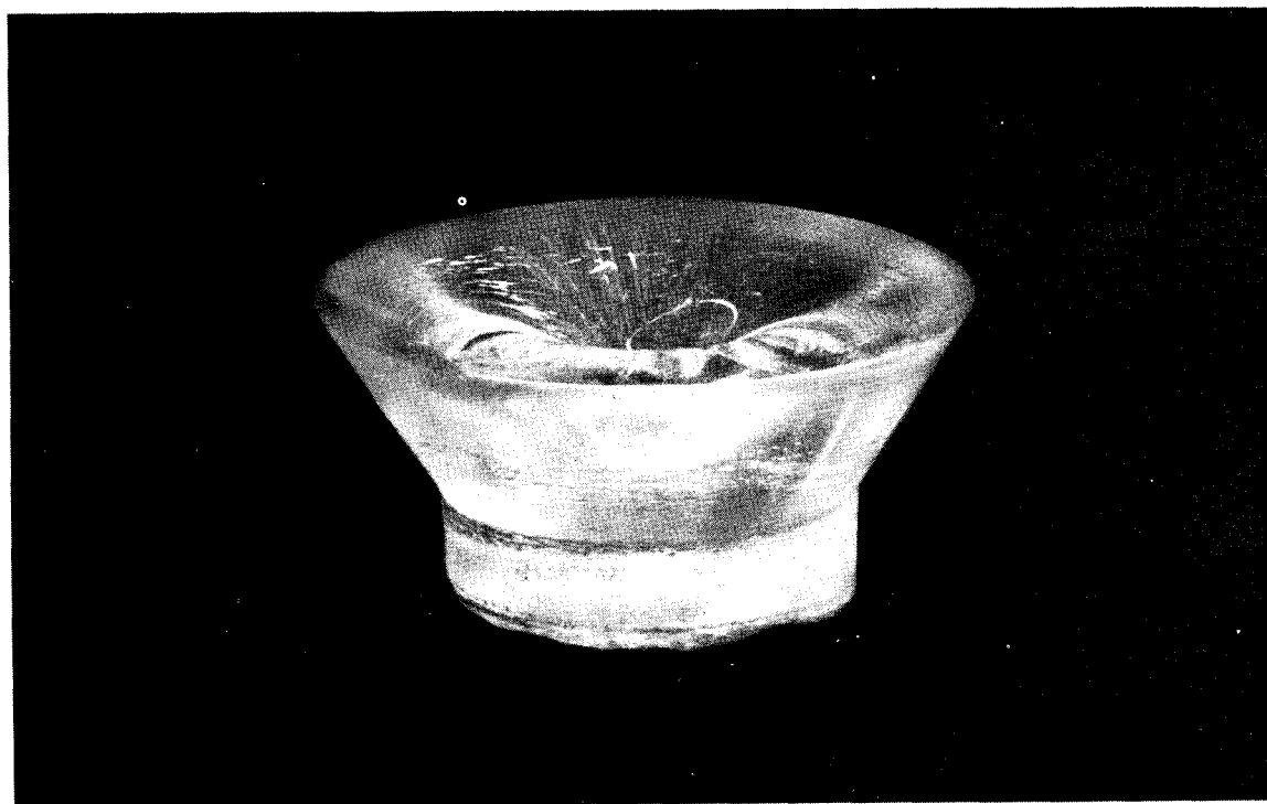
Figure B-6. Arrested failure of 1-inch-diameter, 60°, 0.625 t/D ratio window at 26,600 psi, high-pressure face.
