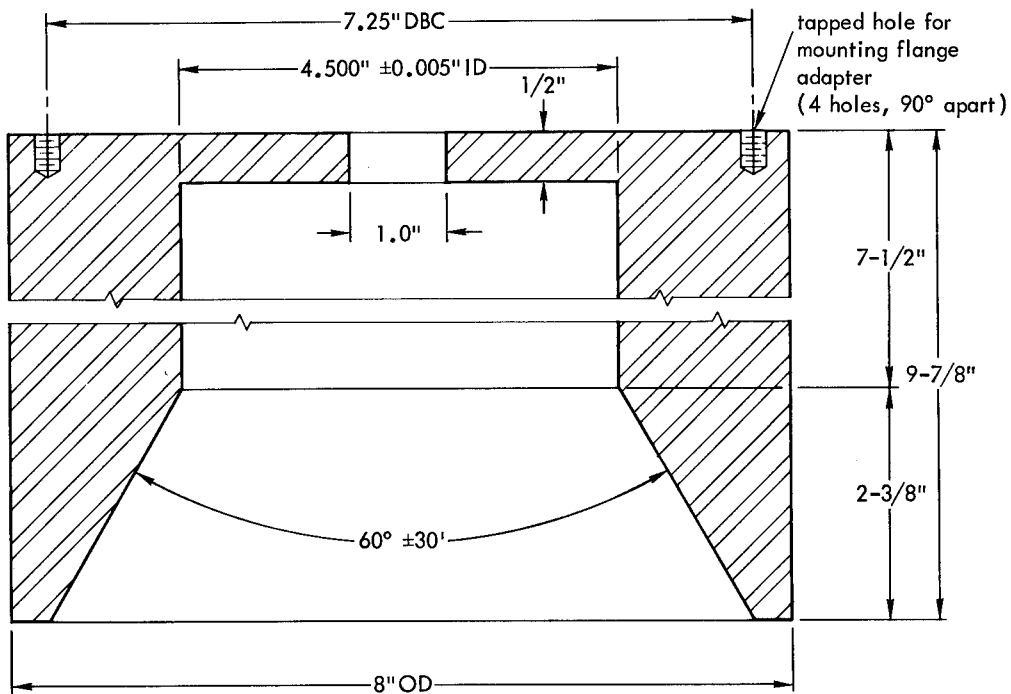
Figure E-2. DOL Type I configuration mounting flange for 4.5-inch-diameter, 60° conical window scaling factor validation tests.
