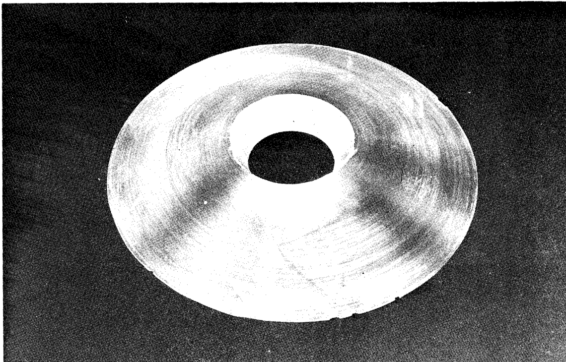
Figure B-38. Failed 1-inch-diameter, 150^\circ , 0.625 t/D ratio window, low-pressure face.
