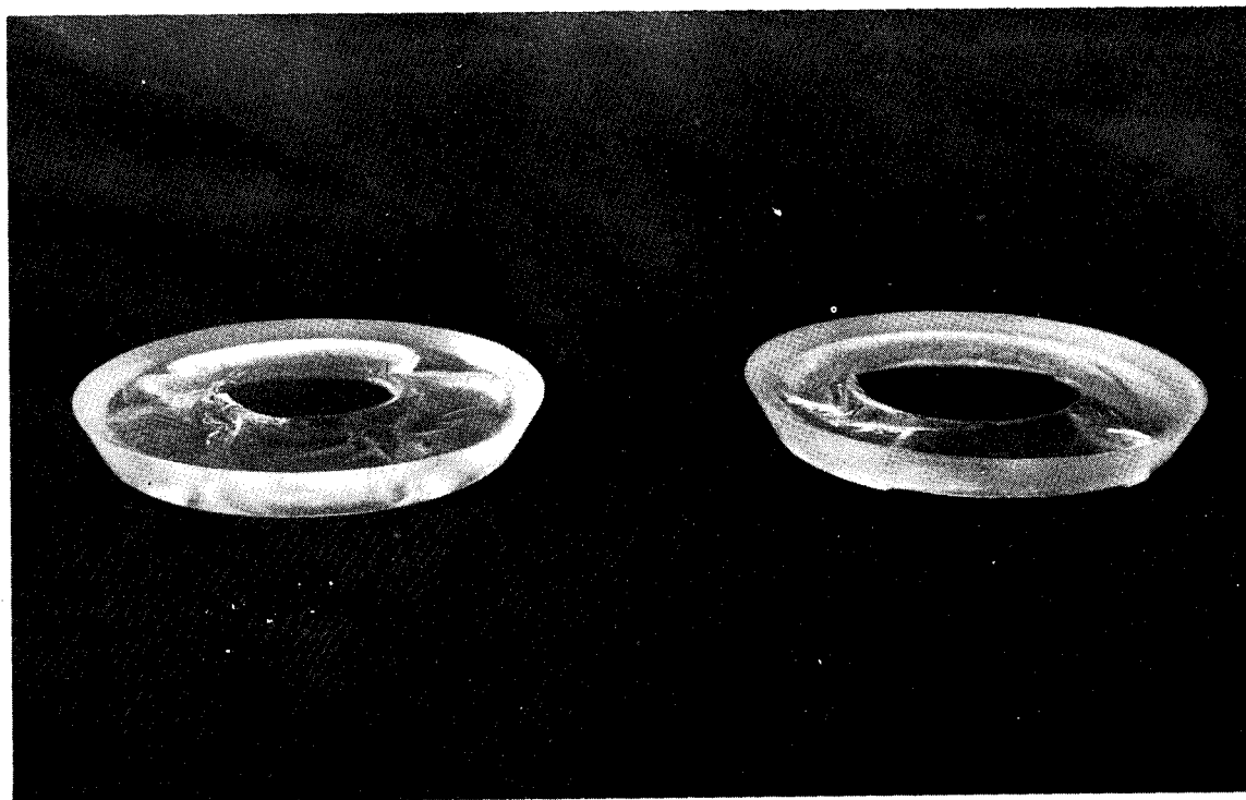
Figure B-4. Failed 1-inch-diameter, 60^\circ , 0.25 t/D ratio windows, high-pressure faces.
