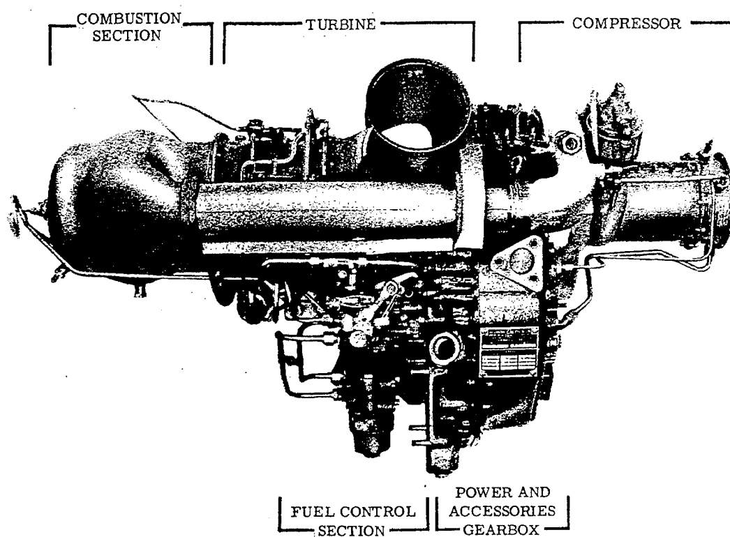
Figure 2.1. T63-A-700 Turboshift Gas Turbine Engine. "From Ref. [1] with permission from Allison Engine Co."
