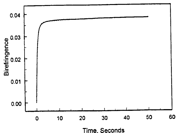
Figure 4. The experimental and biexponential fitted writing curve: Solid line: fitted curve; dots: experimental points.
