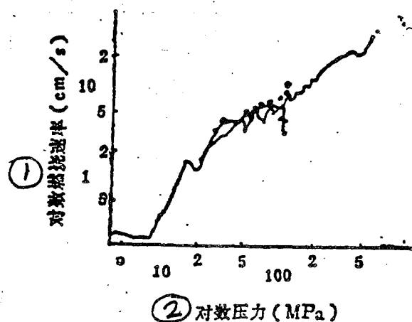
Fig.8 M43 Combustion Speeds With/Without Plasma
