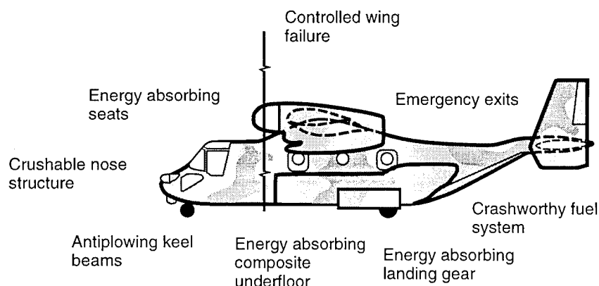
Figure B4.1.2.4-1 V-22 Crashworthy Design Features
