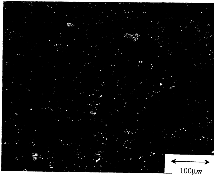
Figure 10: Polarized Light Optical Micrograph of the Al 6061-20 v/o Al 2 O 3 MMC Which Has Been Processed Only By Extrusions.
