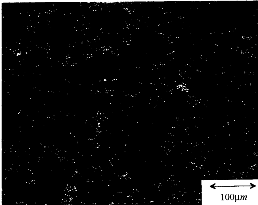
Figure 26: Polarized Light Optical Micrograph of the Al 6061-20 v/o Al 2 O 3 MMC Which Has Been Processed by Extrusions and Draw/Anneal Cycles (Underaged Condition, Gage Section).
