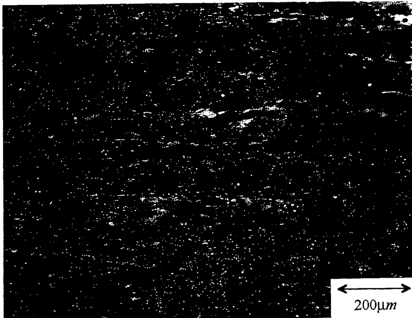
Figure 43: Polarized Light Optical Micrograph of the Al 6061-10 v/o Al 2 O 3 MMC After Hot Forging to a True Strain of 1.10 and Cold Working to a True Strain of 1.79 in the Channel Die Assembly.
