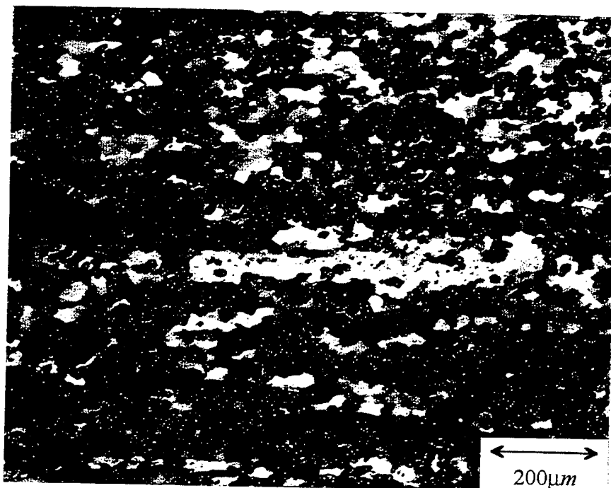
Figure 41: Polarized Light Optical Micrograph of the Al 6061-10 v/o Al 2 O 3 MMC After Hot Forging to a True Strain of 1.10.
