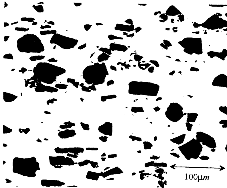
Figure 16: Optical Micrograph of the Al 6061-20 v/o Al 2 O 3 MMC Which Has Been Processed Only by Extrusions (Underaged Condition, Gage Section).
