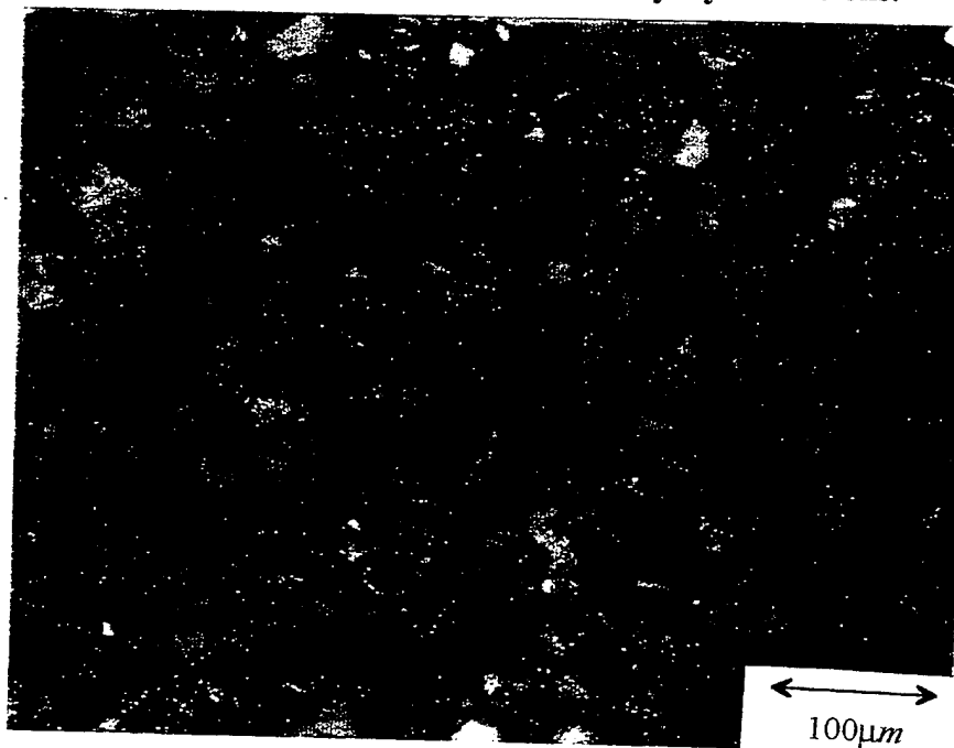
Figure 11: Polarized Light Optical Micrograph of the Al 6061-20 v/o Al 2 O 3 MMC Which Has Been Processed by Extrusions and Draw/Anneal Cycles .
