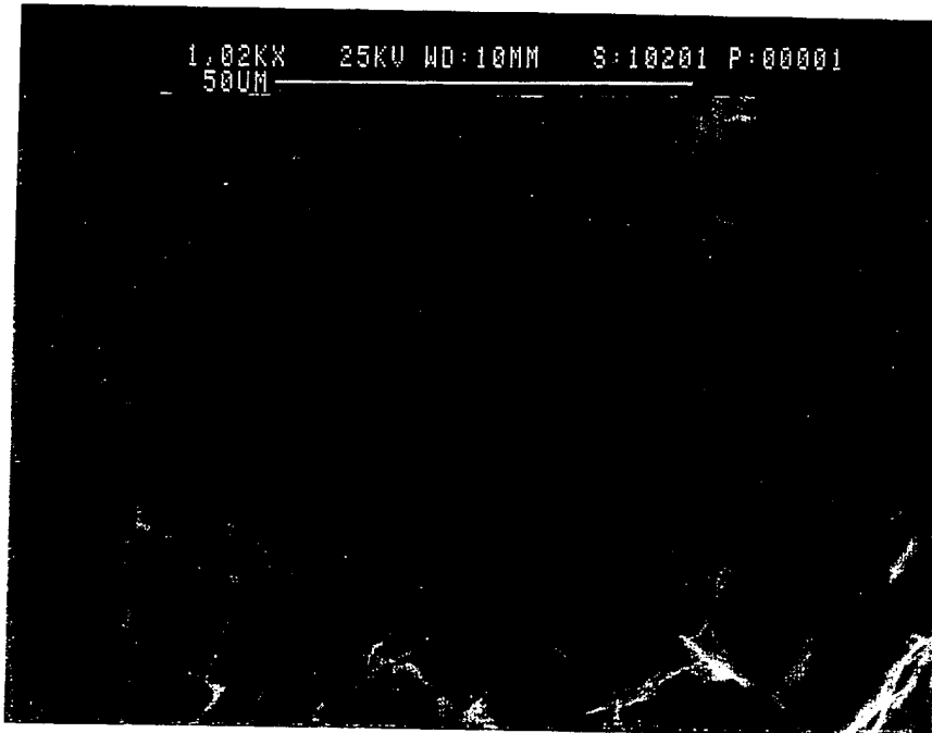
Figure 29: SEM Micrograph of the Fracture Surface of the Al 6061-10 v/o Al 2 O 3 MMC That Has Been Processed by Extrusions and Draw/Anneal Cycles (Underaged Condition).
