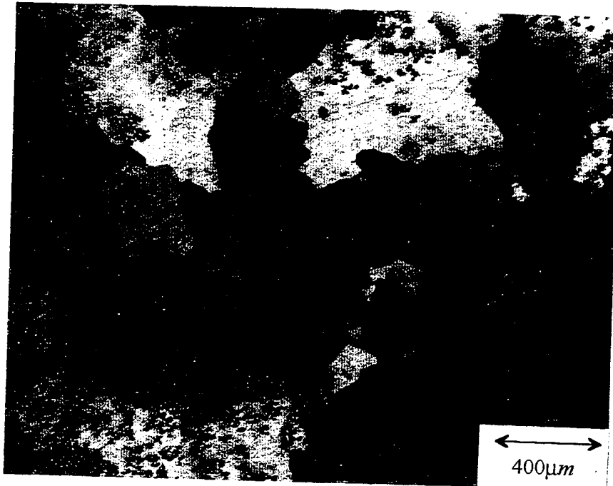
Figure 37: Polarized Light Optical Micrograph of the as Cast Billet of Al 6061-10 v/o Al_2O_3 .
