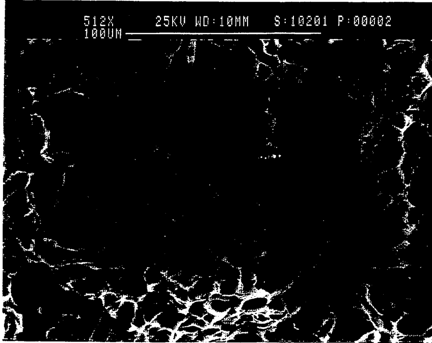
Figure 28: SEM Micrograph of the Fracture Surface of the Al 6061-10 v/o Al 2 O 3 MMC That Has Been Processed by Extrusions and Draw/Anneal Cycles (Underaged Condition).
