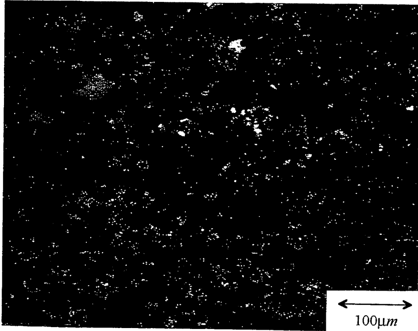
Figure 6: Polarized Light Optical Micrograph of the Al 6061-10 v/o \text{Al}_2\text{O}_3 MMC Which Has Been Processed Only by Extrusions.
