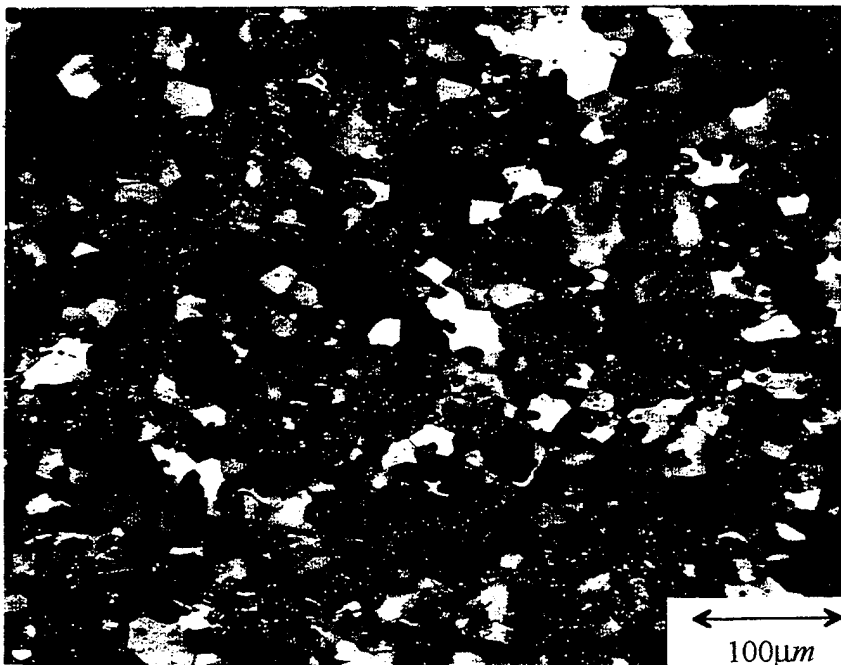
Figure 27: Polarized Light Optical Micrograph of the Al 6061-20 v/o Al 2 O 3 MMC Which Has Been Processed by Extrusions and Draw/Anneal Cycles (Peak Aged Condition, Gage Section).
