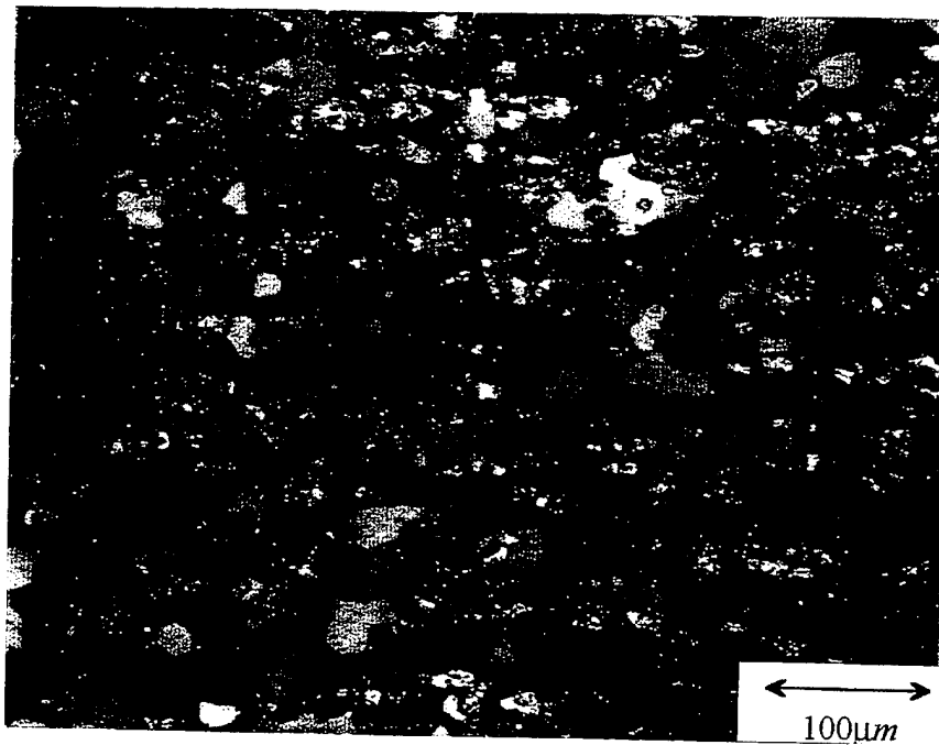
Figure 7: Polarized Light Optical Micrograph of the Al 6061-10 v/o \text{Al}_2\text{O}_3 MMC Which Has Been Processed by Extrusions and Draw/Anneal Cycles.
