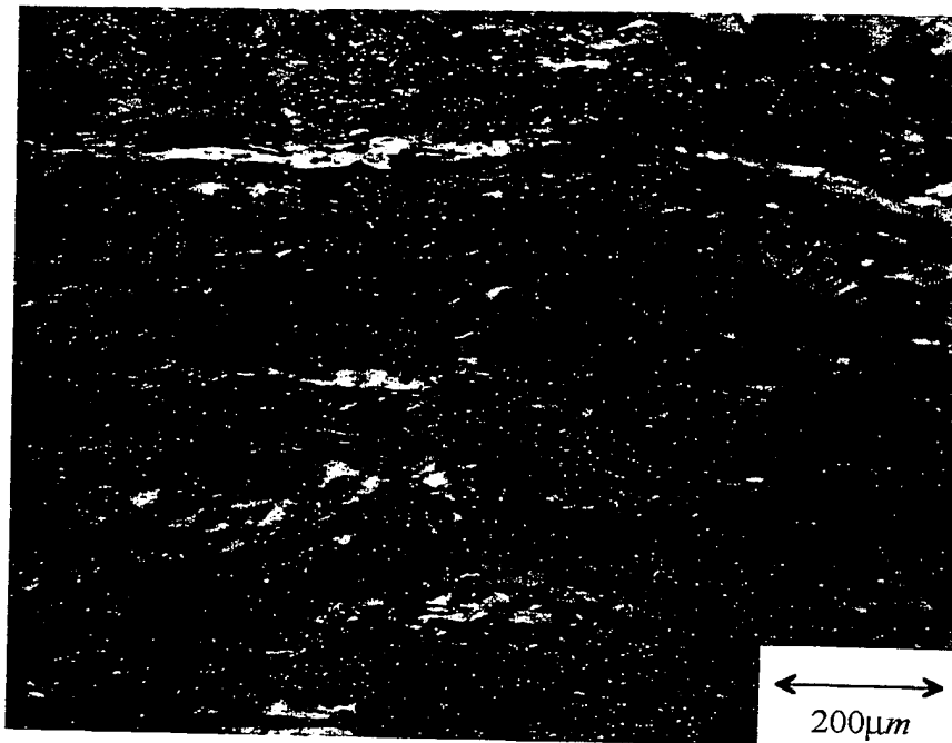
Figure 40: Polarized Light Optical Micrograph of the Al 6061-10 v/o Al 2 O 3 MMC After Hot Forging to a True Strain of 0.51 and Cold Working to a True Strain of 1.20 in the Channel Die Assembly.
