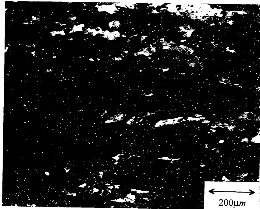
Figure 39: Polarized Light Optical Micrograph of the Al 6061-10 v/o Al 2 O 3 MMC After Hot Forging to a True Strain of 0.51 and Cold Working to a True Strain of 0.80 in the Channel Die Assembly.
