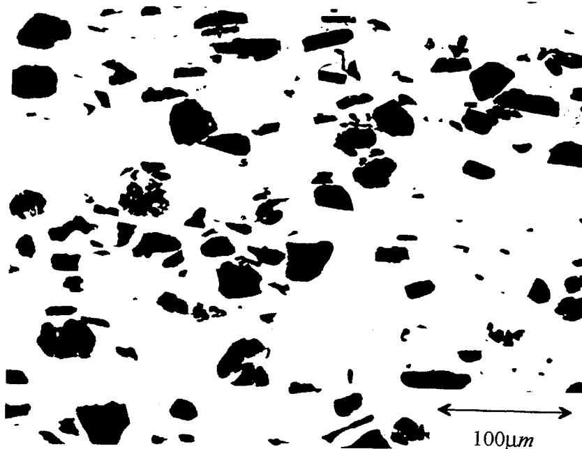
Figure 17: Optical Micrograph of the Al 6061-20 v/o Al 2 O 3 MMC Which Has Been Processed Only by Extrusions (Underaged Condition, Gage Section).
