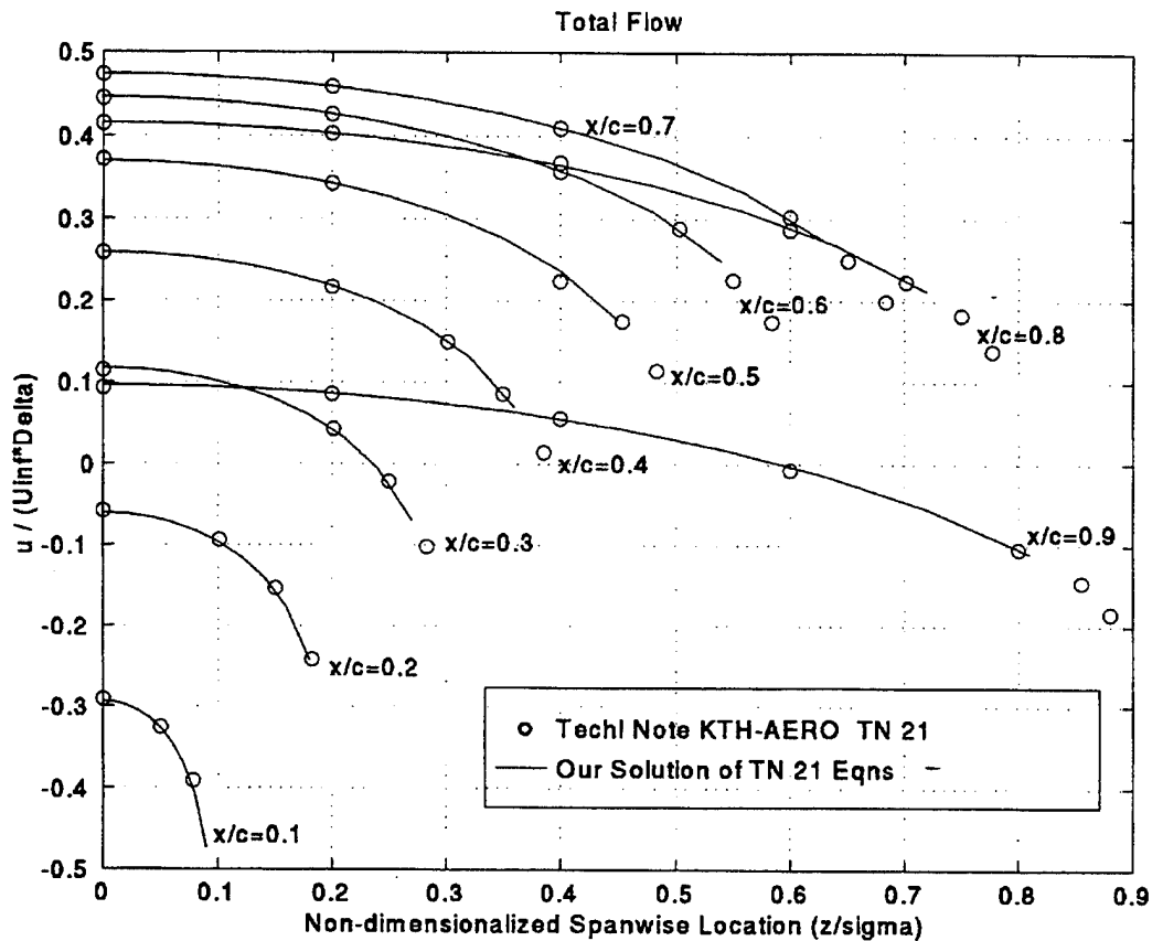
Figure 3.59 Comparison of The Combined u-Components of The Chordwise Basic Flow as a Function of Non-Dimensionalized Spanwise Location. Triangular Wing, Parabolic Arc Spanwise Section, AR=2/3, AOA=0 Degree.
