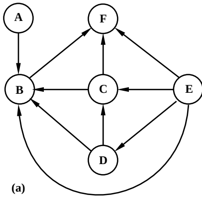
Figure 3.11: (a) Occlusion graph for the mechanism in Fig. 3.10, and (b) the visibility order produced by sorting the graph.
