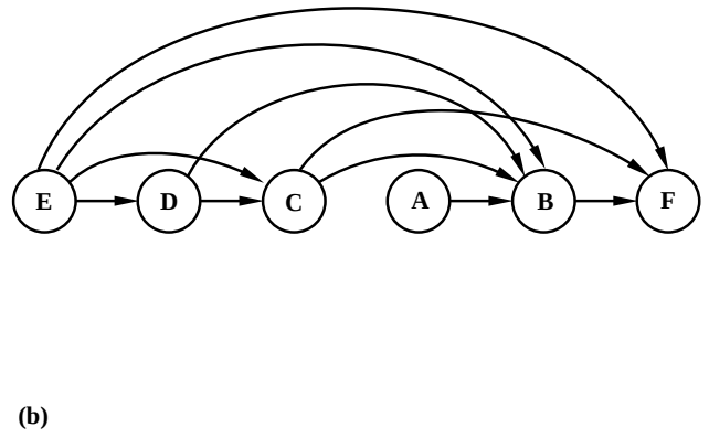
Figure 3.11: (a) Occlusion graph for the mechanism in Fig. 3.10, and (b) the visibility order produced by sorting the graph.
