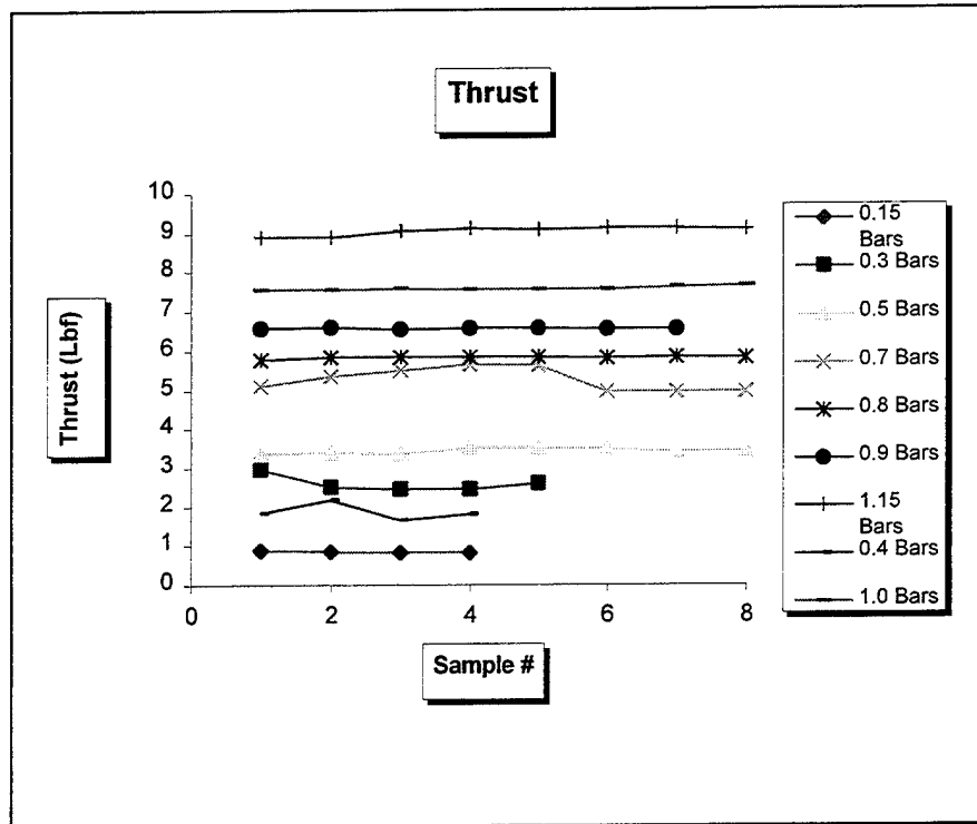
Figure 21 Thrust Measurements
