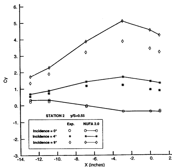
Figure 16 : Comparison of NUFA and Experimental Grid Loads Beneath Model M165 with Pylon at Mach 0.7 (c) Side Force Coefficient
