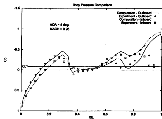
Figure 8. Surface Pressure Comparisons (Inboard and Outboard)
