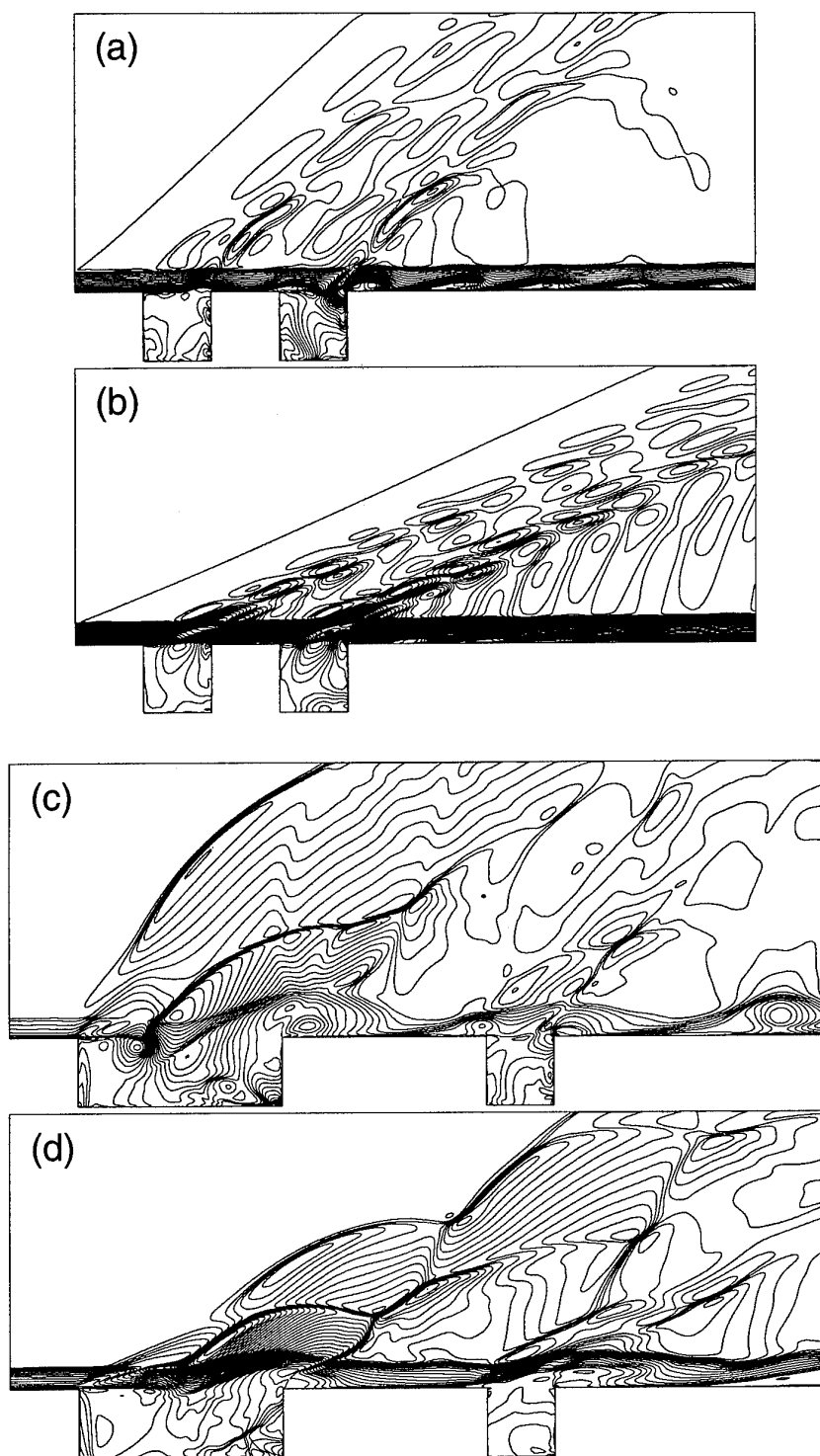
Figure 3: Instantaneous density contours: (a) type A configuration, M_\infty = 1.5 , \Delta\rho/\rho_\infty = 0.015 ; (b) type A configuration, M_\infty = 2.5 , \Delta\rho/\rho_\infty = 0.015 ; (c) type B configuration, M_\infty = 1.5 , \Delta\rho/\rho_\infty = 0.035 ; (d) type B configuration, M_\infty = 2.5 , \Delta\rho/\rho_\infty = 0.035 ;
