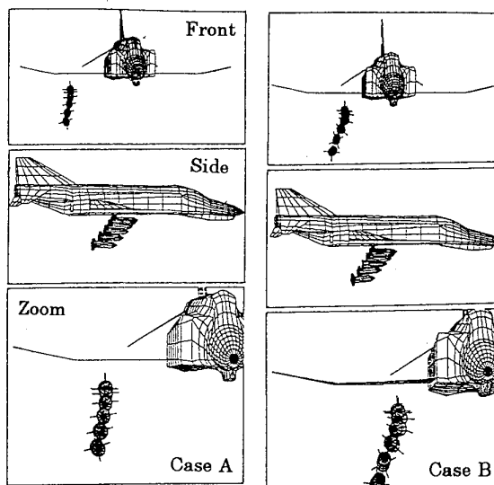
Figure 3. Store separation analyses by using a combined panel method/flow grid technique (16).
