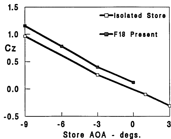
Figure 6 - FREESTREAM DATA
