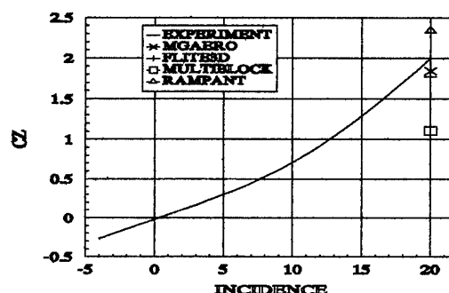
Figure 11: Predicted Normal Force For Store C
