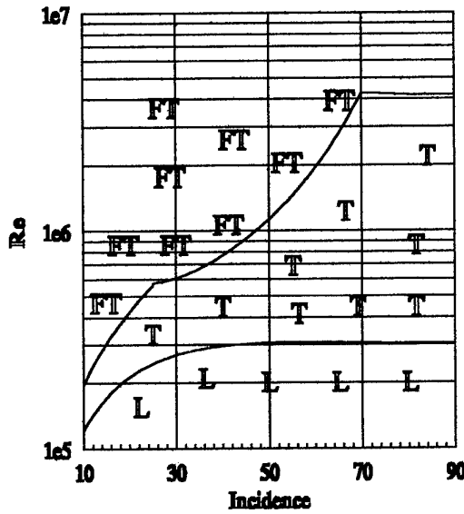
Figure 2: Critical Reynolds Number Boundaries
