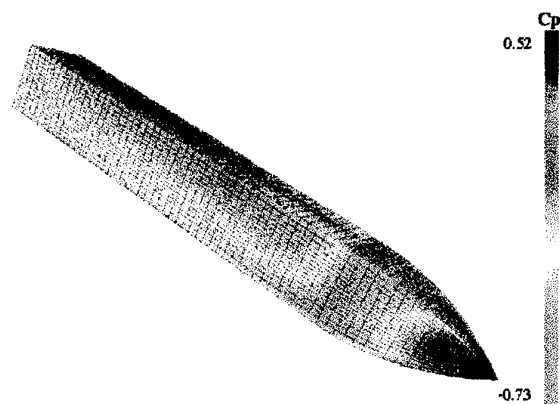
Figure 5: Surface C_p From MGAERO, Store D, M=0.9 , \alpha=20^\circ
