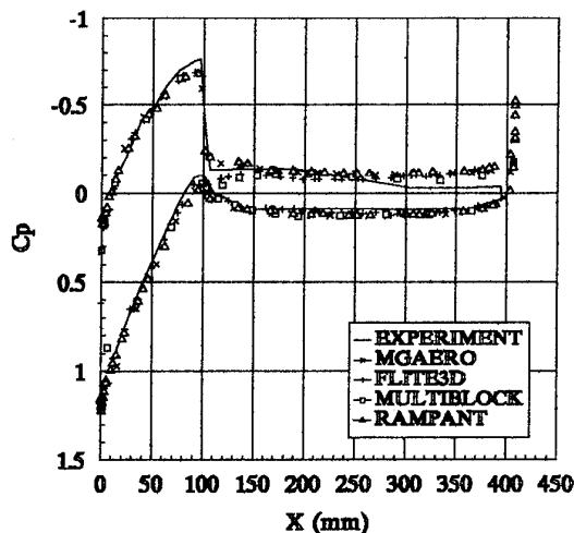
Figure 8: Store D Centre Line Pressure Coefficients Compared With Experiment.
