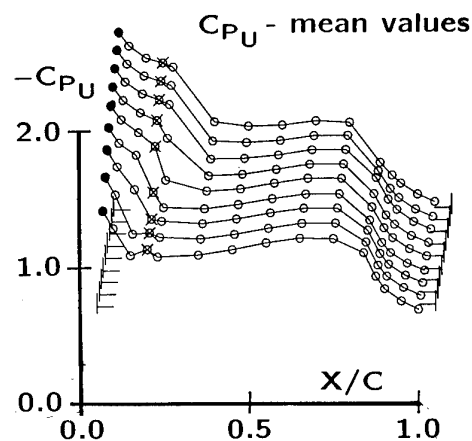
a) Mean pressure coefficients, upper wing surface, WS3.
