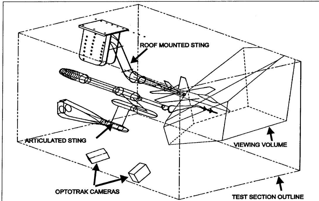
Figure 1 - GRID SURVEY RIG SCHEMATIC
