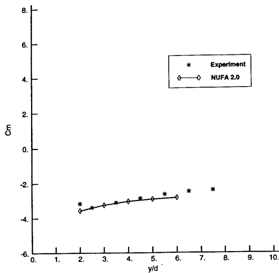
Figure 20 : Comparison of NUFA and Experimental Grid Loads. Traverse from Bay 1F. Bay 1F Cover Off. (b) Pitching Moment Coefficient
