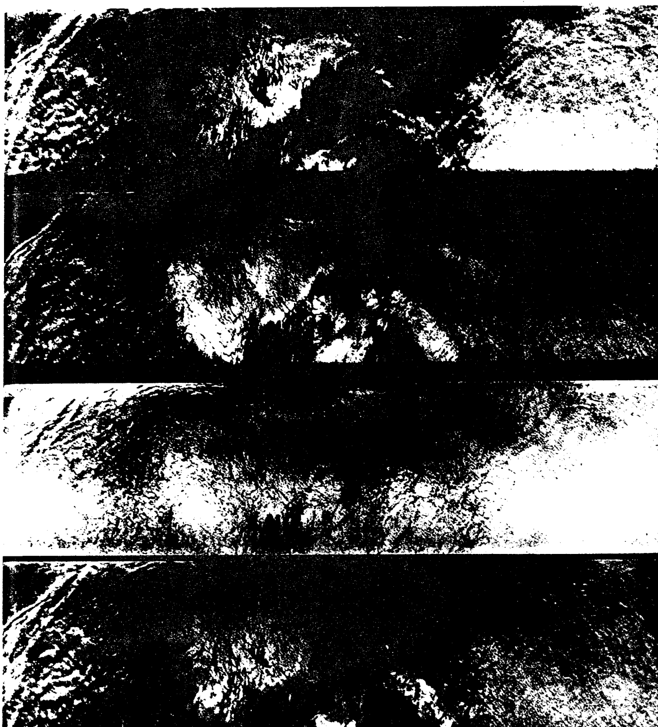
Figure 4-6. b) AIRSAR images at P, L, and C-bands/VV of the area made within the stripe on figure 4-6 (a). Significant differences exist between the AIRSAR images that relate to the surface roughness variations over the upwelling; these occur because what is "rough" at a short radar wavelength is often "smooth" at longer lengths -- the Rayleigh criterion for a rough surface. Radar crosssection reduction at C-band is in excess of 7 dB. The surface wind speed was uniformly 5 m/s throughout the entire region shown, thus illustrating the effects of air-sea interaction on radar backscatter (Richard Carande). PVV = Red, LVV = Green, CVV = Blue.
