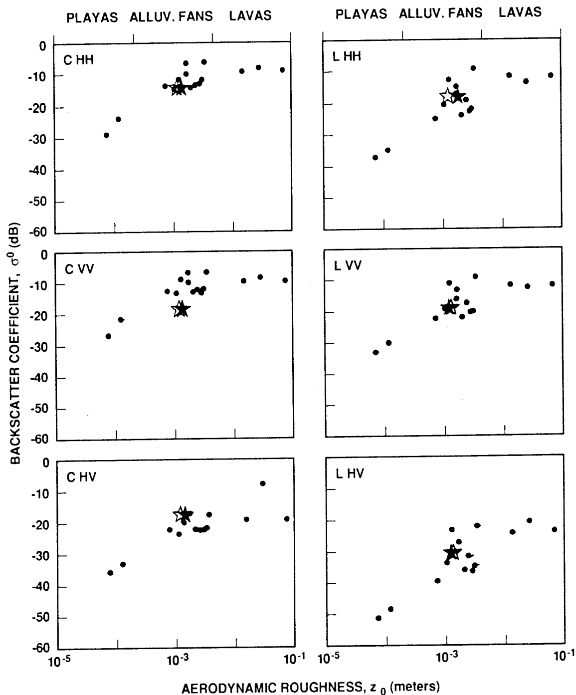
Figure 6-11. Radar backscatter observations of the SRL-1 super site at Stovepipe Wells, Death Valley, have been used to calculate aerodynamic roughness. The solid circles are from AIRSAR campaigns. Black star denotes prediction of Z_0 for the site. The models were based on AIRSAR data, the backscatter values were derived from SRL-1 data. The open star denotes the measured Z_0 value based on wind and temperature data collected in the field.
