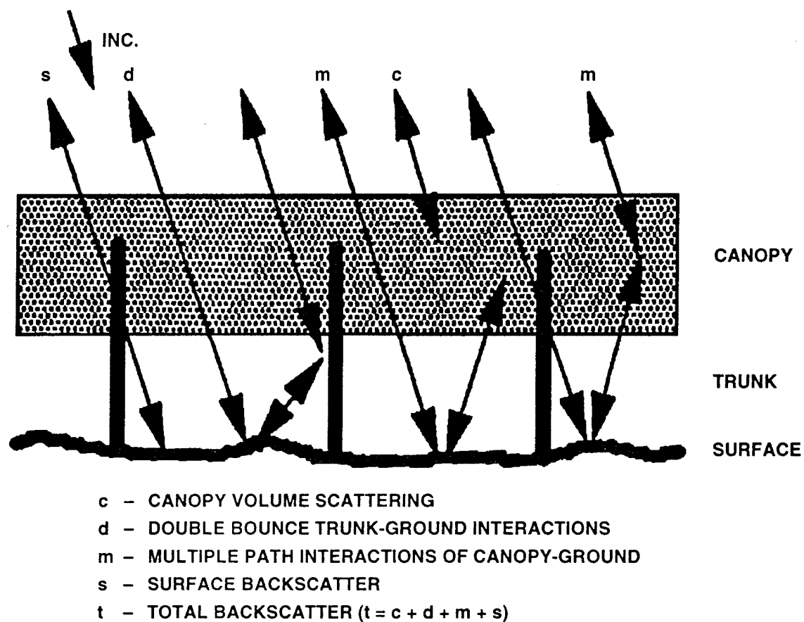
Figure 2-1. Schematic diagram of major scattering terms in microwave modeling of forest canopies (after Wang et al 1993c).
