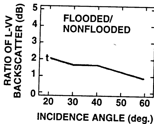
Figure 2-3. Use of theoretical models to understand radar scattering from vegetated surfaces. Model-predicted microwave scattering from a flooded forest on the floodplain of the Amazon River as a function of radar frequency and incidence angle (after Wang et al., 1995). "t" indicates total backscatter as shown in Figure 2-1.
