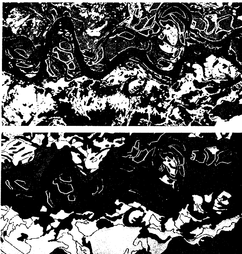
Figure 2-4. d) Images showing classification of natural vegetation/landcover (top) based on AIRSAR data of Bonanza Creek, Alaska and vegetation map (bottom) (Rignot and Way, 1994).
