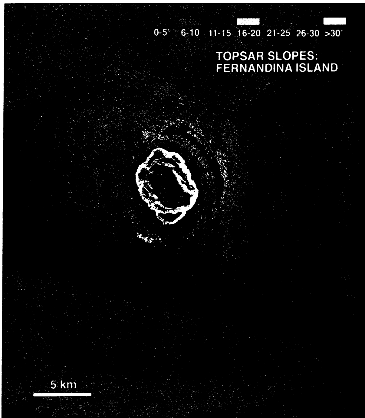
Figure 6-4. This map was prepared from TOPSAR airborne interferometry data obtained over the basaltic shield volcano Fernandina in the W. Galapagos Islands. The first derivative of the digital topographic data (obtained at 10 m/pixel resolution) has been calculated for an area 30 x 30 m in size so that the variation in slopes on the volcano can be identified. Here we see that the upper slopes on the outside of the caldera can exceed 30°, while the flanks near the coast all have slopes less than 5°. This type of analysis lends itself very well to many types of geomorphic studies (including an analysis of drainage basins, mountain ranges, and volcanoes), and is well suited to the regional view of topography that would be provided by an orbital radar interferometer.
