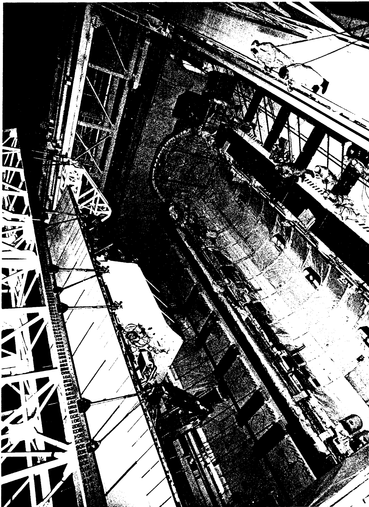
Figure 7-5. SIR-C/X-SAR being lowered into the cargo bay.
