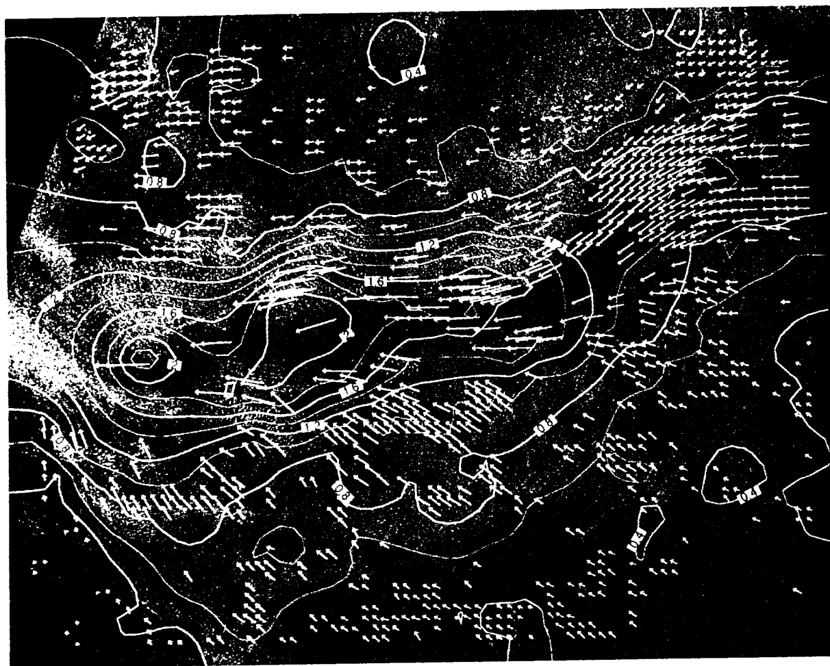
Figure 5-9. Surface velocity field of Jakobshavn Glacier (Fahnestock and others, 1993).
