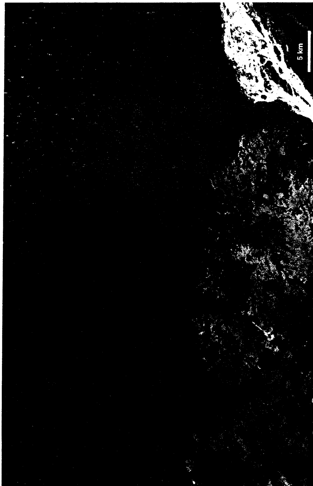
Figure 6-8. This SIR-C image shows the region around the site of the lost city of Ubar in southern Oman, on the Arabian Peninsula. The ancient city was discovered in 1992 with the aid of remote sensing data. Archeologists believe Ubar existed from about 2800 B.C. to about 300 A.D. and was a remote desert outpost where caravans were assembled for the transport of frankincense across the desert.
