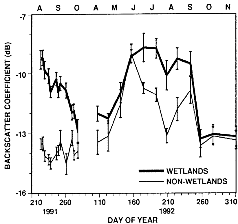
Figure 2-9. Seasonal variation in ERS-1 SAR backscatter for wetlands ("flooded") and non-wetlands ("moist/dry") for data collected over Barrow, Alaska (mean \pm standard error) (from Kasischke et al., 1995a).
