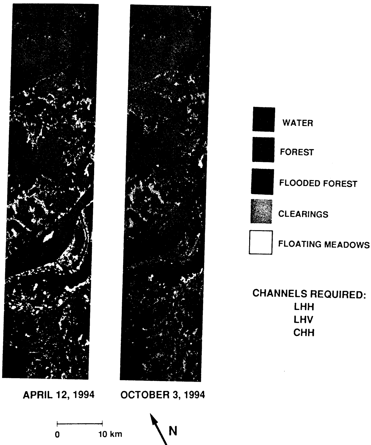
Figure 2-4. b) Maps of the flooding and land cover from data obtained by the SRL-1 on April 12, 1994 (left) and SRL-2 on October 3, 1994 (right). The rivers extending across the scenes are the Rio Negro (top) and Rio Solimoes (Center). Classification was prepared using L-band HH and HV polarizations, and C-band HH polarization. Field studies by boat, on foot, and in low flying aircraft done by UCSB in collaboration with Brazil's INPA and INPE during the SRL-1 and SRL-2 missions have validated the interpretation of the radar images (Hess, Melack, Filoso, and Wang, 1995).
