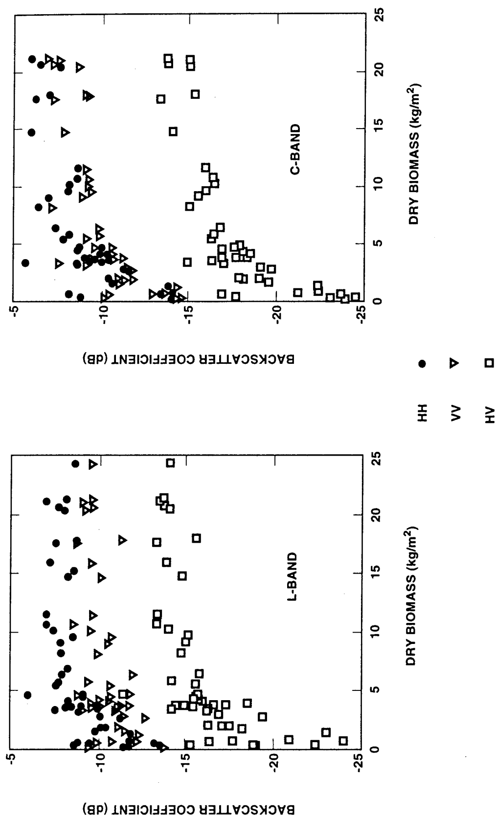
Figure 2-6. Dependence of L- and C-band SAR backscatter on aboveground biomass (from Dobson et al., 1995c).
