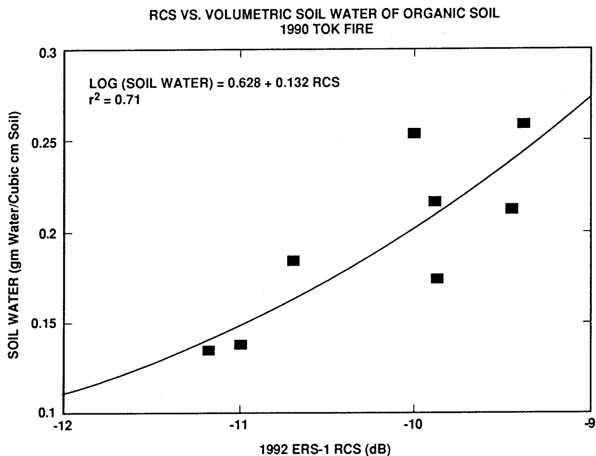
Figure 2-12. Relationship between ERS-1 SAR radar cross section and volumetric soil moisture from test sites in the 1990 Tok forest fire site (from Kasischke et al., 1995a).
