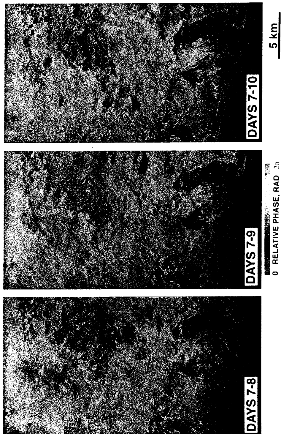
Figure 6-6. Comparison of the phase data collected over the Pu'u O'o eruption site of Kilauea volcano, Hawaii, on days 7 to 10 of the SRL-2 mission (October 7th-10th, 1994). The three images compare the phase data for October 7th with October 8th (left), 9th (center), and 10th (right). Particularly relevant are the patches of purple phase anomalies ~15-20 km inland (towards the top of the image). These anomalies are transient on a daily basis, and are interpreted to be due to the presence of rain cells at the time of data collection. They indicate that interferometric data needs to be collected frequently so that local atmospheric errors can be eliminated by excluding the worst scenes from the deformation comparisons.
