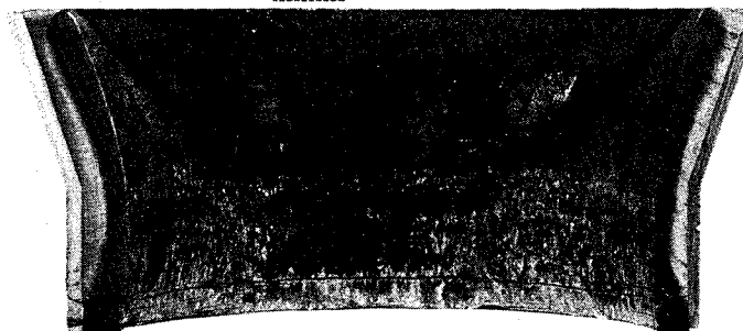
Figure 17. - Char formation, nozzle 9.
