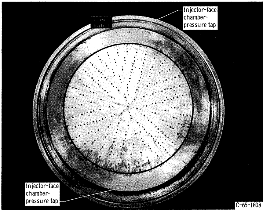
Figure 4. - Injector.
