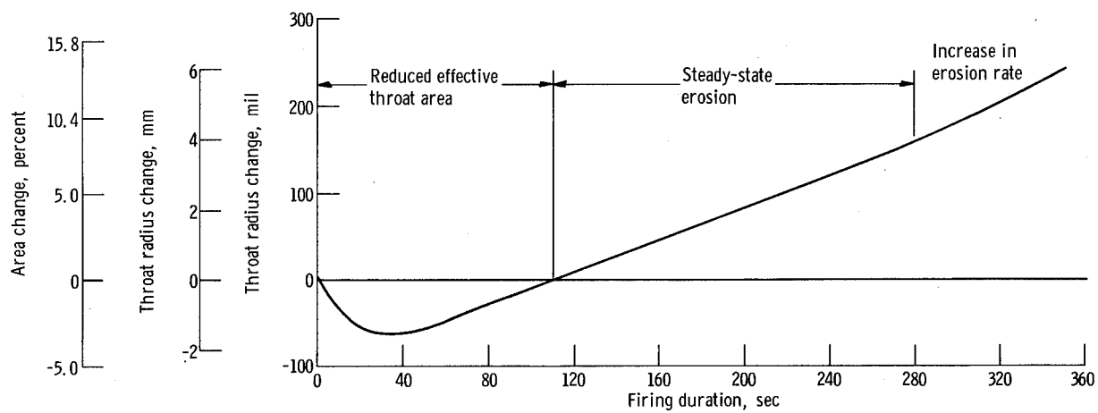
Figure 8. - Typical nozzle erosion curve.
