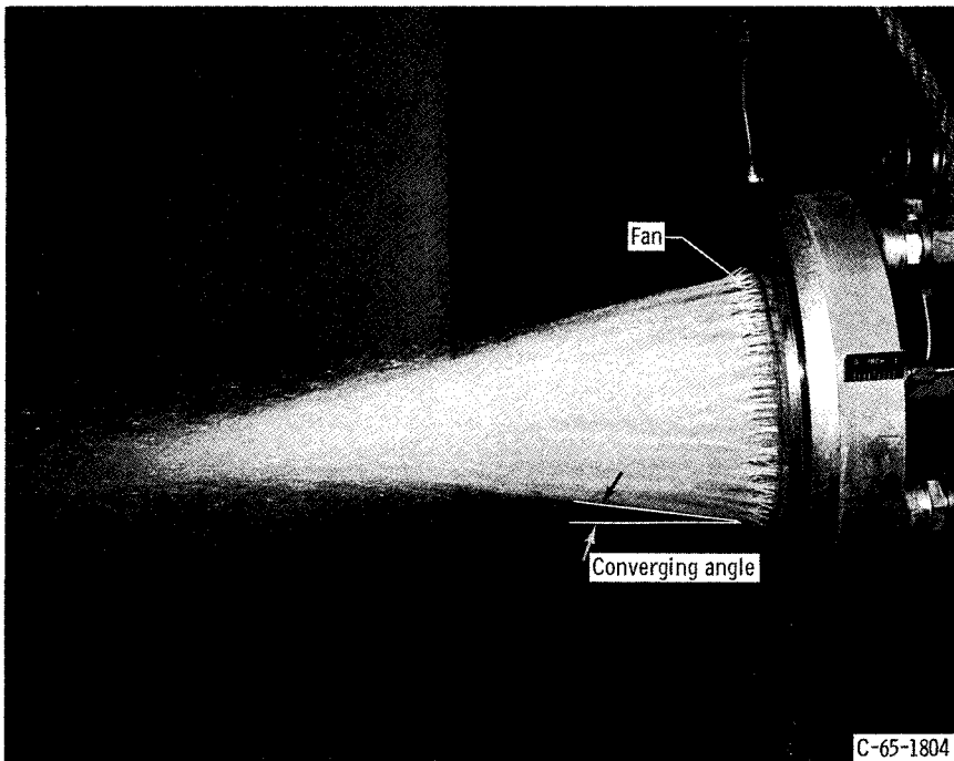
Figure 5. - Water-flow test.
