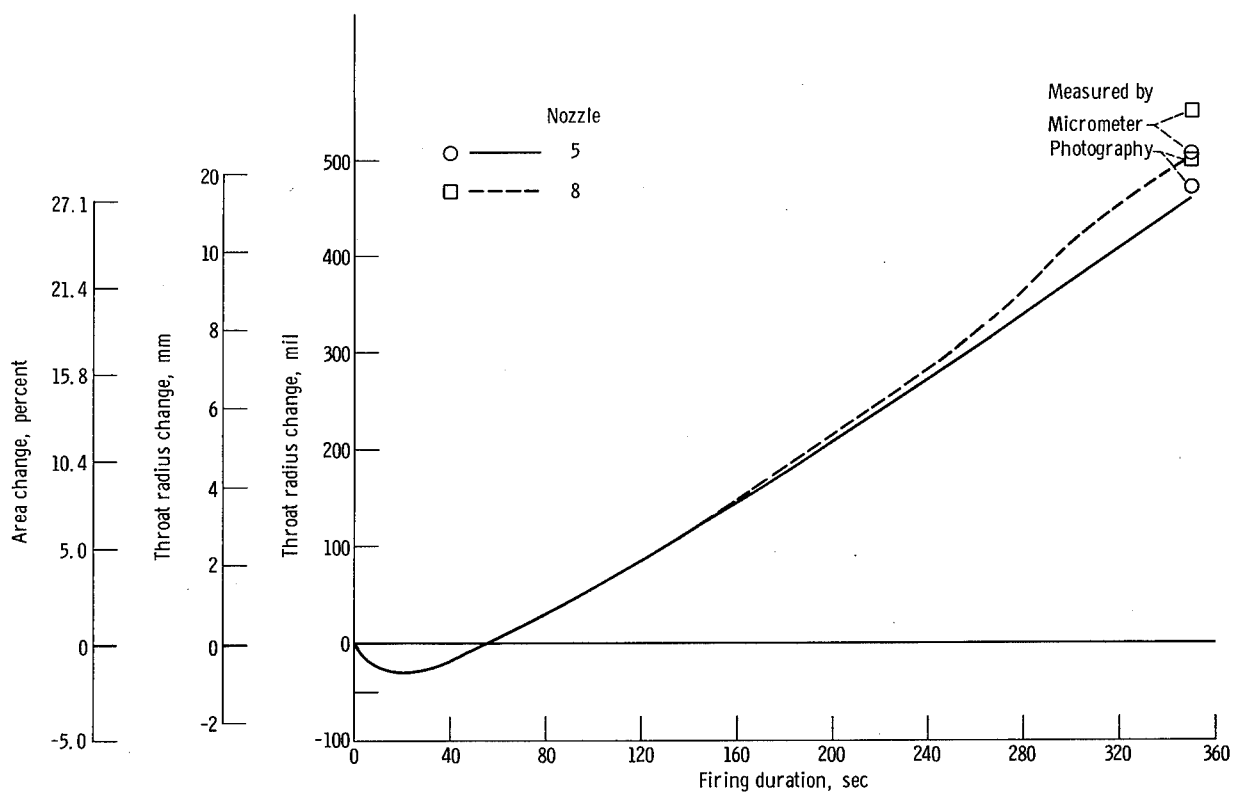
Figure 9. - Erosion for nozzle 5, small-diameter fiber, 90° fiber-orientation angle, and nozzle 8, large-diameter fiber, 90° fiber-orientation angle.
