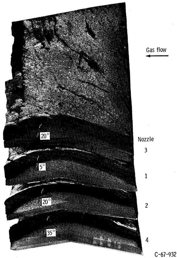
Figure 12. - Postfiring examination showing rosette layup angle of orientation.
