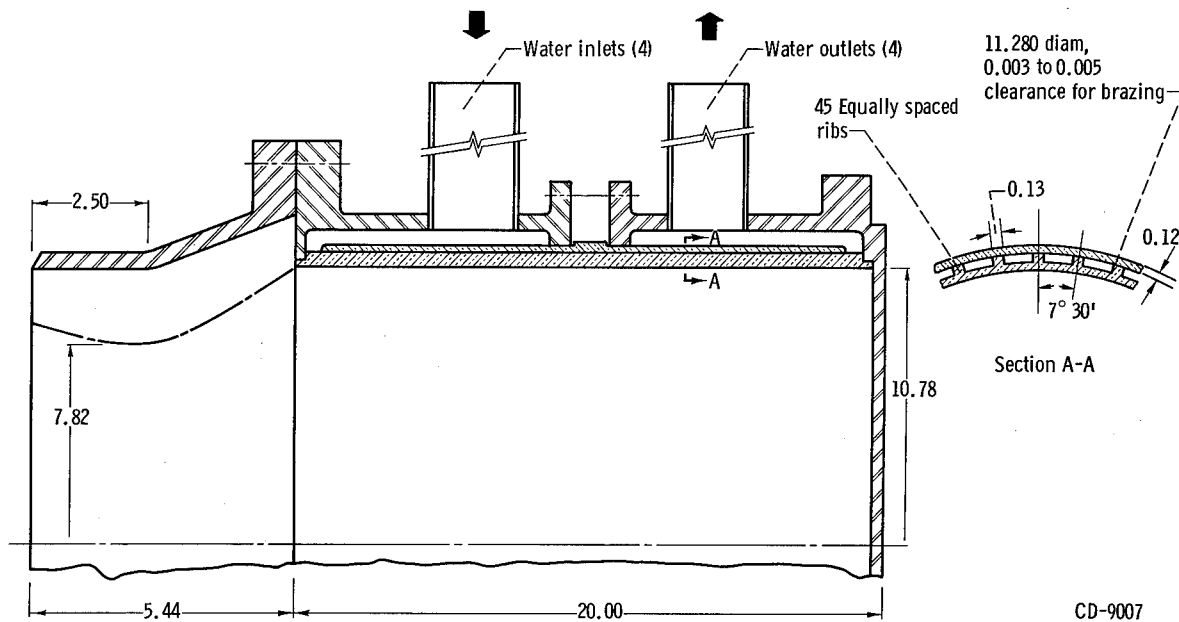
Figure 6. - Water-cooled combustion chamber and nozzle assembly. All linear dimensions are in inches. Multiply by 2.54 to convert to centimeters.
