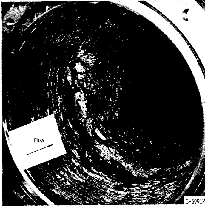
(c) Chunkout regions in the chamber section after 223 seconds.
