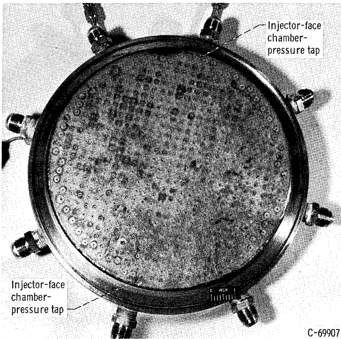
(a) After 313 seconds.
