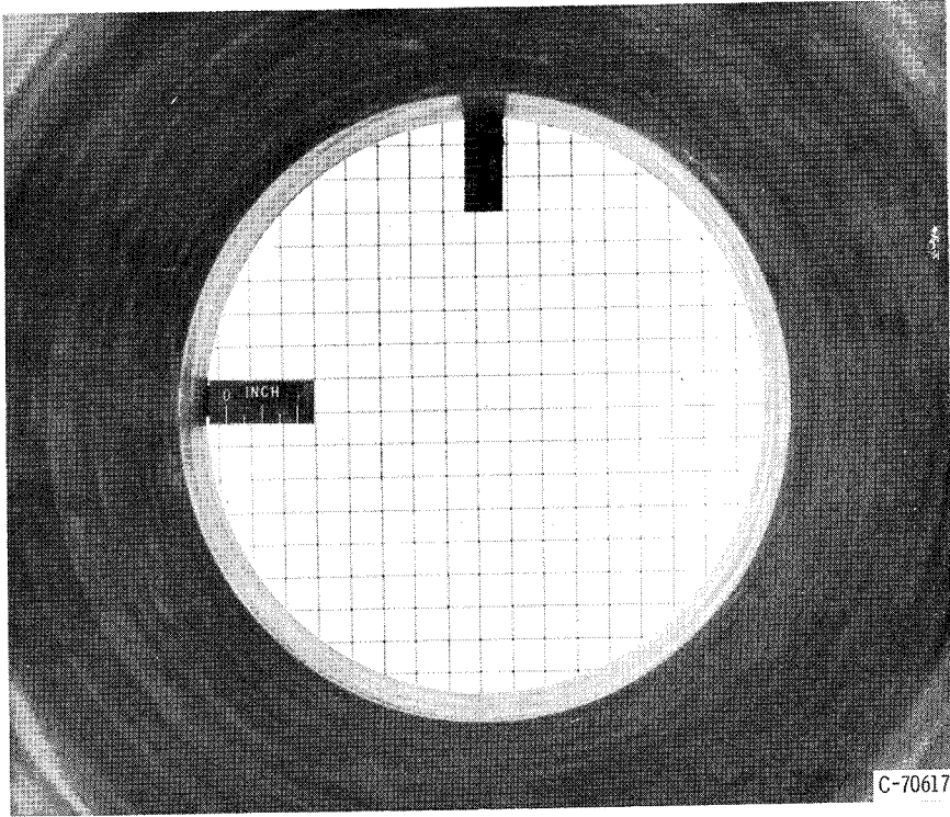
(a) Chamber 1, 0 seconds.
