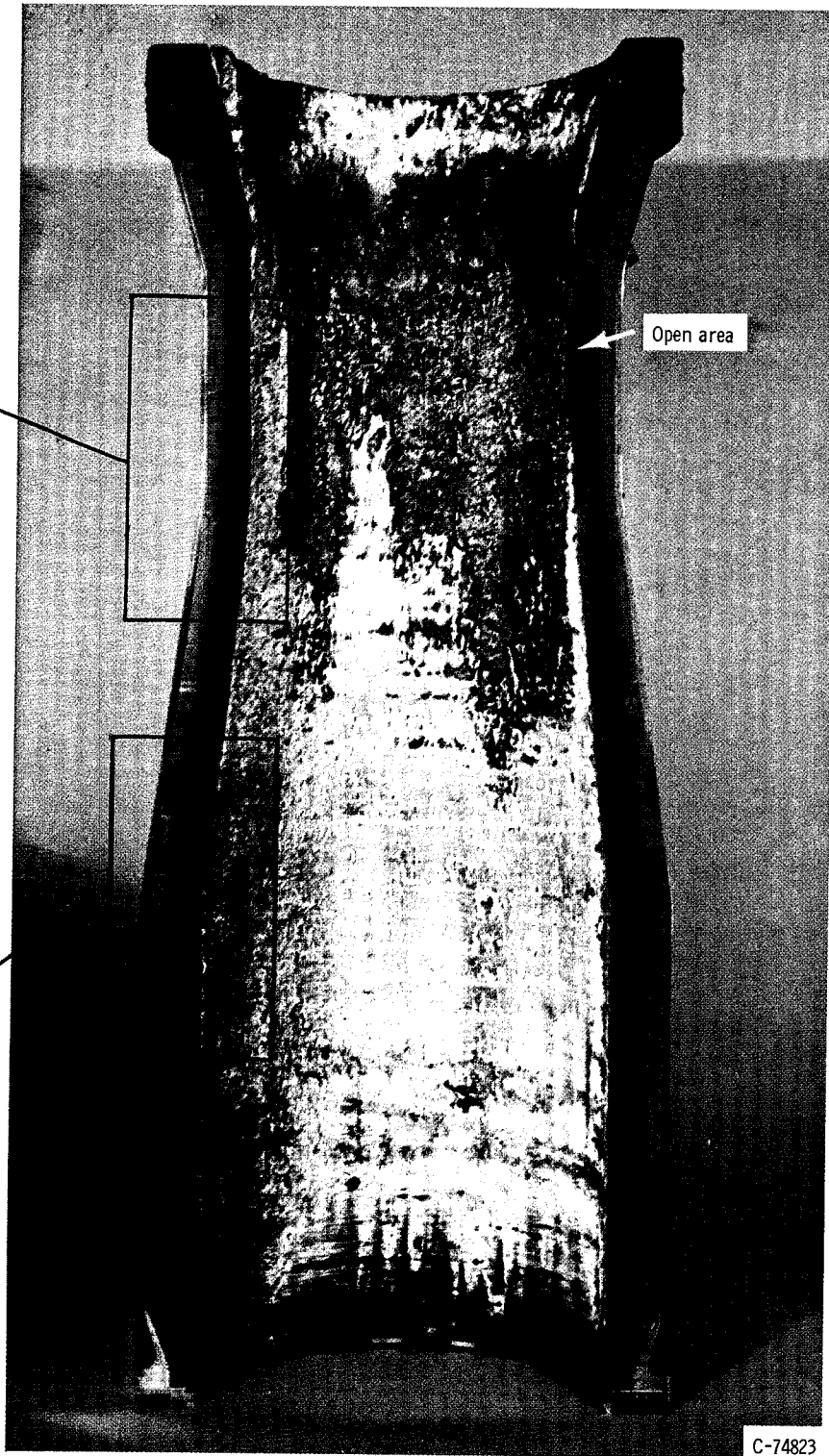
(c) Cross section of chamber after 592 seconds.
