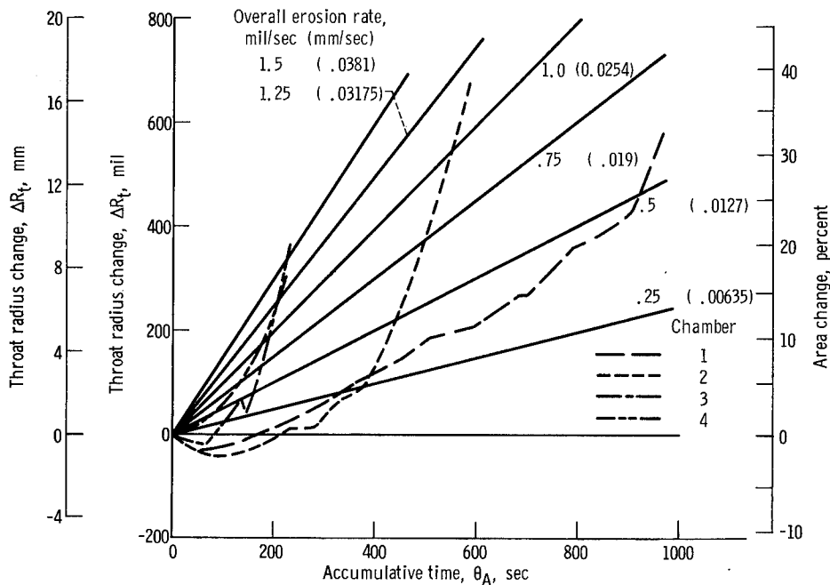
Figure 12. - Comparison of erosion of four ablative materials.
