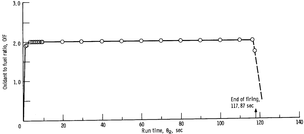
(b) Typical oxidant-to-fuel ratio.
