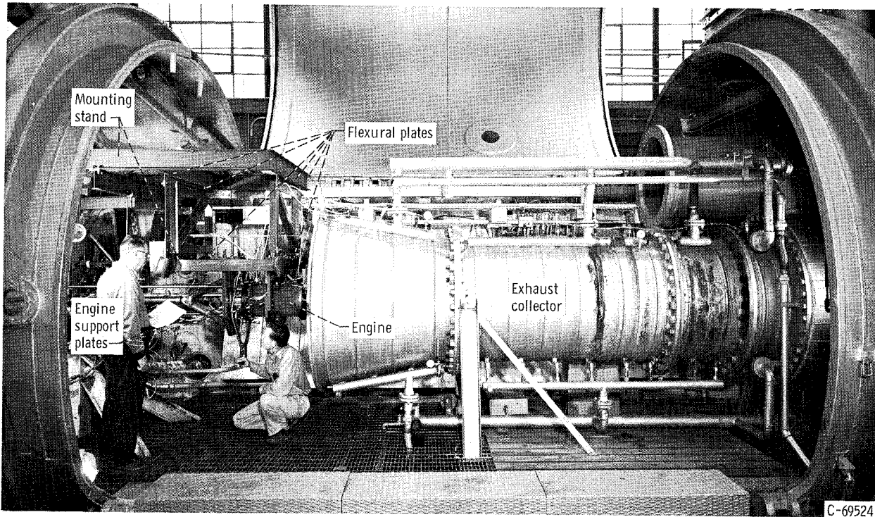
(a) Test chamber and engine.
