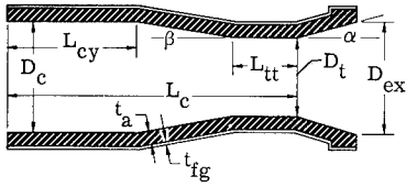
Configuration A. - Full-length tubular-throat ablative chamber.
