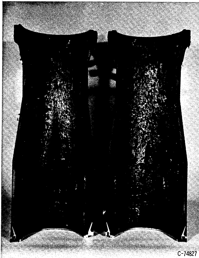
(b) Cross section of chamber after 223 seconds.
