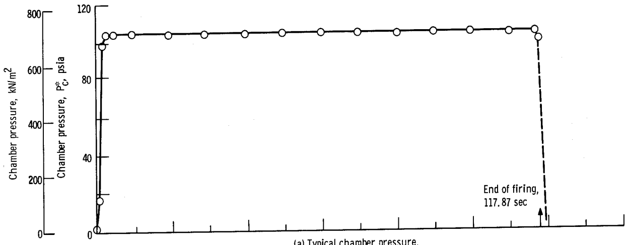
(a) Typical chamber pressure.
