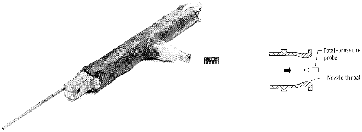
Figure 4. - Throat total-pressure probe.
