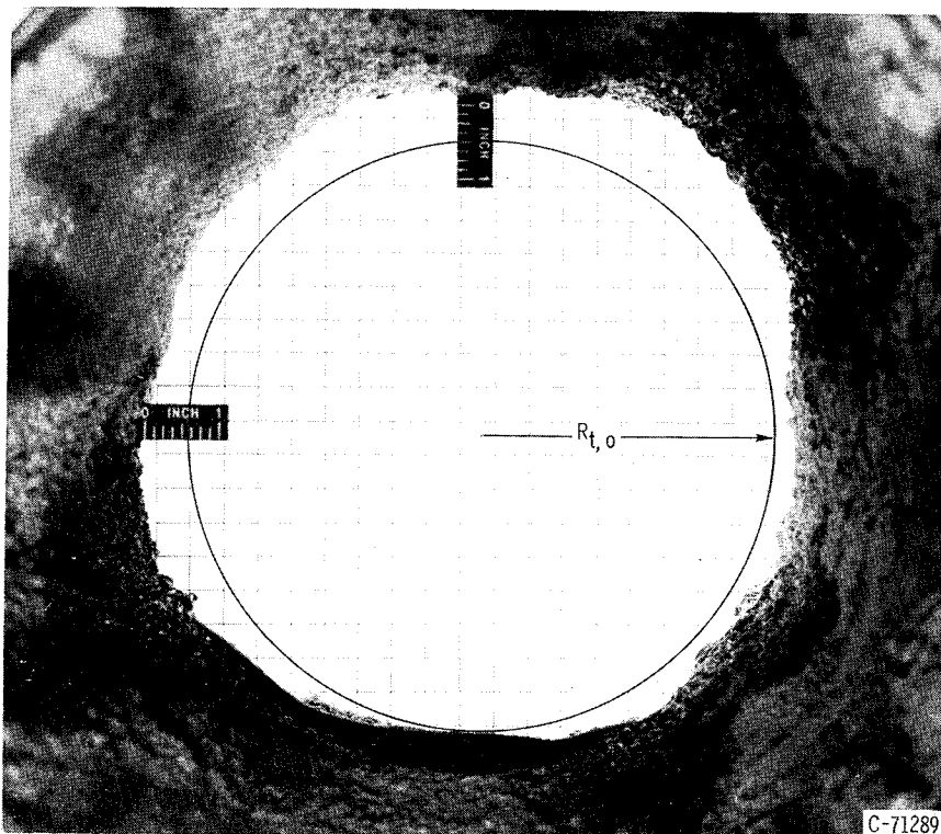
(b) Chamber throat after 967 seconds. Circle is original throat diameter of 7.82 inches.
