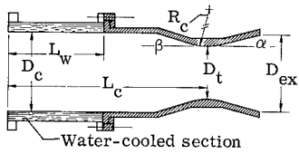
Configuration D. - Short steel heat-sink chamber.
