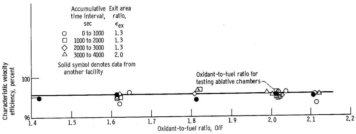
Figure 7. - Combustion performance.
