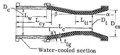
Configuration B. - Short tubular-throat ablative chamber.
