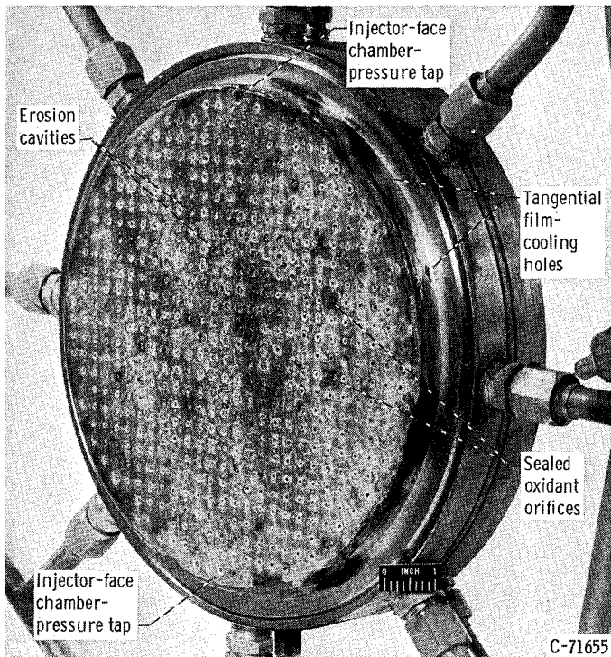
(b) After 3558 seconds.
