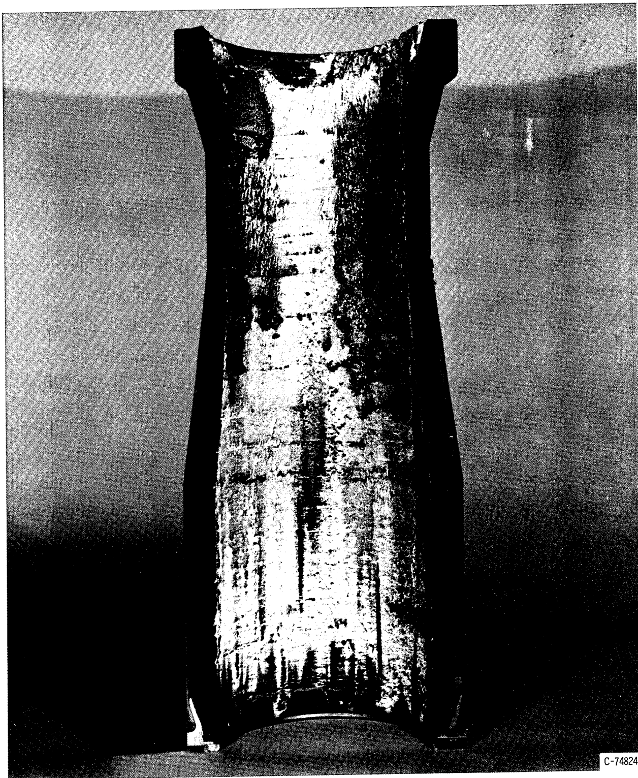
(c) Cross section of chamber after 967 seconds.
