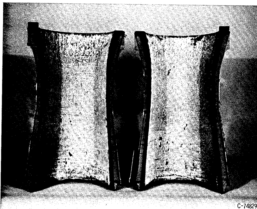
(b) Cross section of chamber after 554 seconds.
