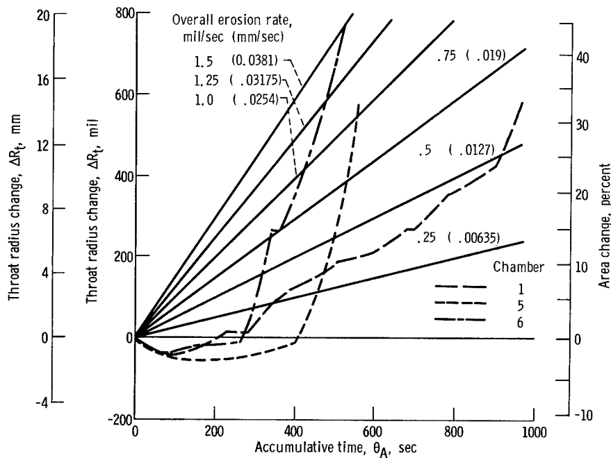
Figure 15. - Comparative effects of chamber geometry.
