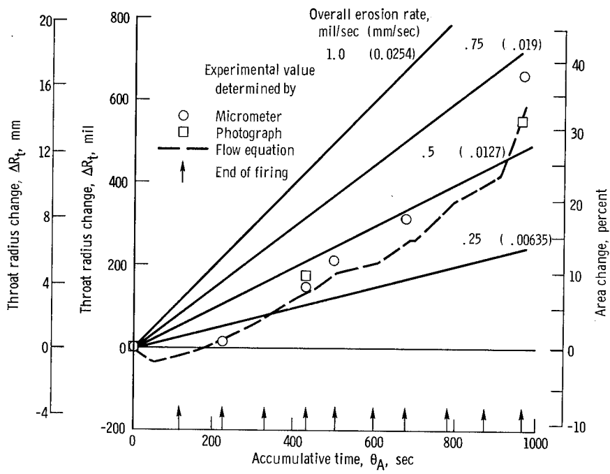
(a) Dimensional time.
