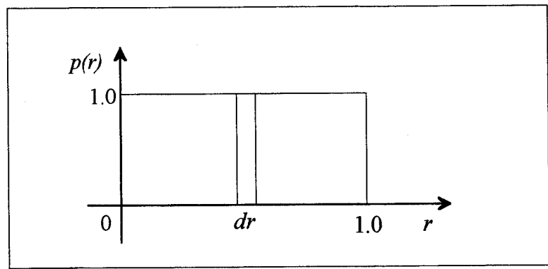
Figure 5-4. Uniform Distribution
