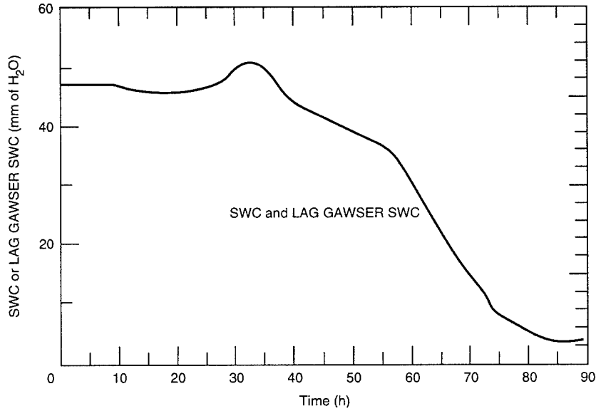
Figure 30. Behavior of the solid water content of the snowpack. SWC matches LAG_GAWSER_SWC (the Fortran prediction of SWC lagged by one hour). The one-hour difference between SWC and LAG_GAWSER_SWC is due to computational differences between Object-GAWSER and the Fortran version of GAWSER.
