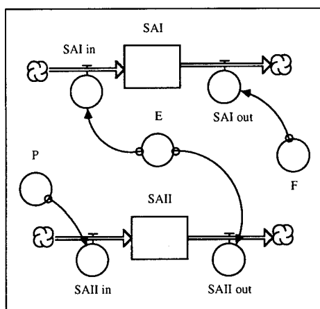
Figure 19. SA_I and SA_II . SAI , SA_I_in , SA_I_out , F , and E are used to calculate the available storage in the top soil layer ( TP_LYR ). SA_II , SA_I_in , SA_II_out , P , and E are used to calculate the available storage in the bottom soil layer ( BTM_LYR ).
