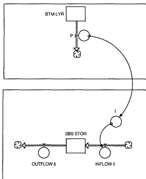
Figure 28. The link between GROFF2 and SBS_STOR_&_FLOW_1. The link between GROFF2 and SBS_STOR_&_FLOW_1 represents the percolation of water in zone two from the bottom soil layer (BTM_LYR) to surbsurface storage (SBS_STOR). "P," the output from GROFF2, is linked to "I," the input to SBS_STOR_&_FLOW_1, with a connector. The link between GROFF2 and SBS_STOR_&_FLOW_1 is identical to the link which joins GROFF3 to GDWTR_&_BASFLW_1, GROFF4 to SBS_STOR_&_FLOW_2, and GROFF5 to GDWTR_&_BASFLW_2. For simplification, only those objects which represent the linkage between GROFF2 and SBS_STOR_&_FLOW_1 are shown.
