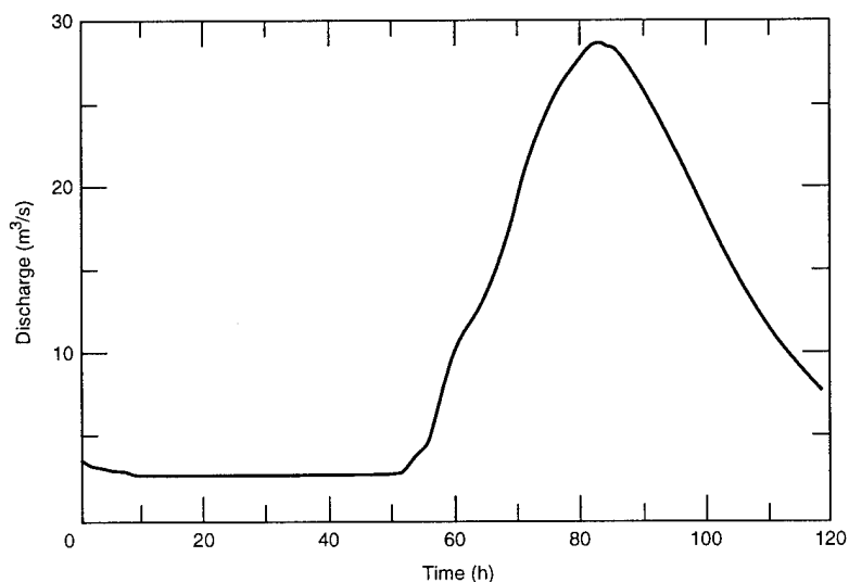
Figure 8. Discharge from a suburban watershed. The discharge begins to increase more rapidly at 50 hours, peaks at 84 hours at 28.63 m 3 /s, and then descends until the end of the simulation. This hydrograph increases and decreases more rapidly and has a larger peak discharge than the hydrograph for the agricultural watershed because the suburban watershed produces more runoff and less subsurface flow and baseflow than the agricultural watershed.
