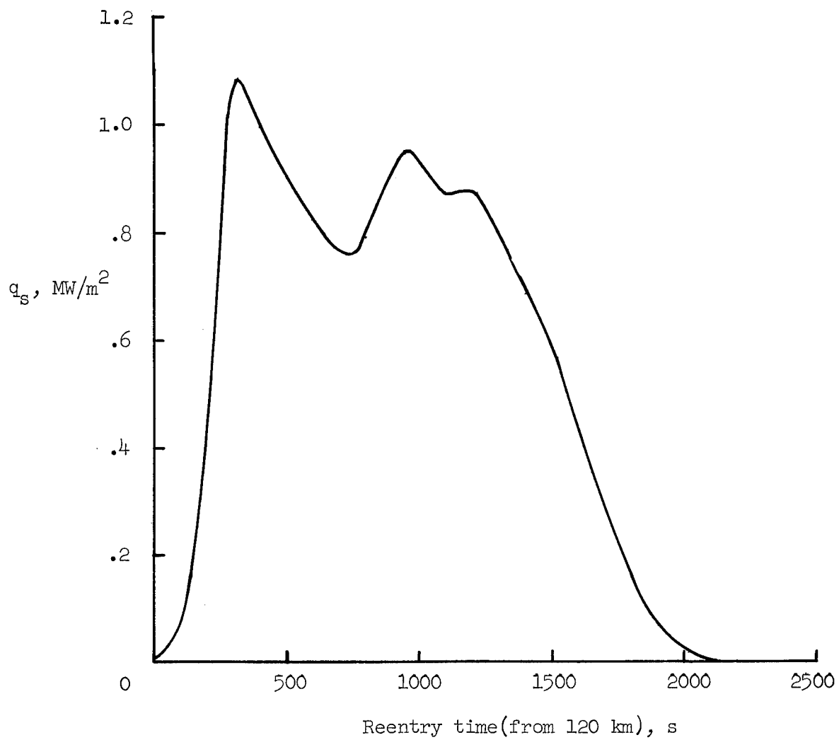
Figure 5.- Typical stagnation-point heating history for lifting-body reentry vehicle.
