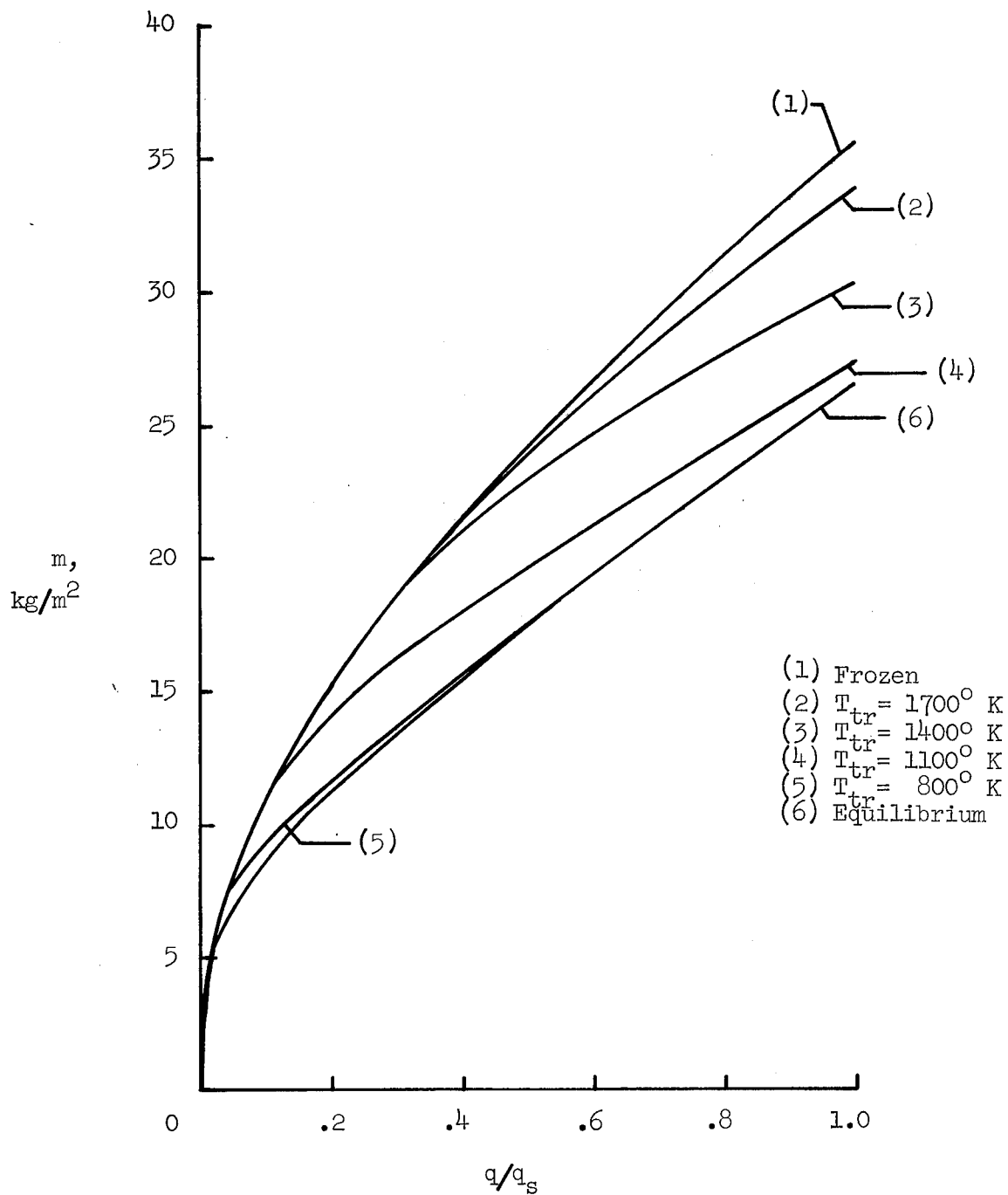
Figure 7.- Effect of the chemical state of the pyrolysis gases on unit mass required to limit back-surface temperature to 530^\circ\text{K} for the lifting-body vehicle.
