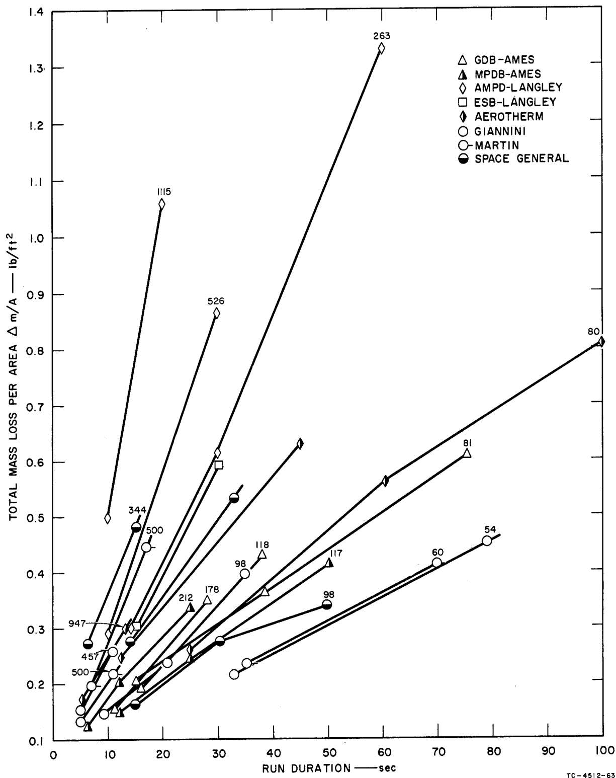
FIG. 28 MASS LOSS OF LANGLEY LOW-DENSITY PHENOLIC-NYLON AS A FUNCTION OF RUN DURATION (Heat Transfer Rate Indicated for Each Facility)
