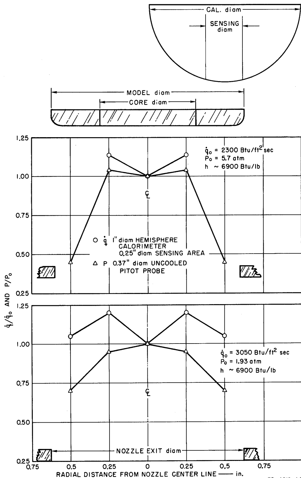
FIG. 12 PLASMA STREAM UNIFORMITY AT AVCO (10-Mw Facility)
