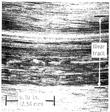
17-4 PH disk
