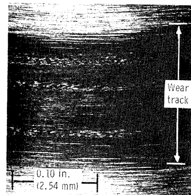
17-4 PH disk
