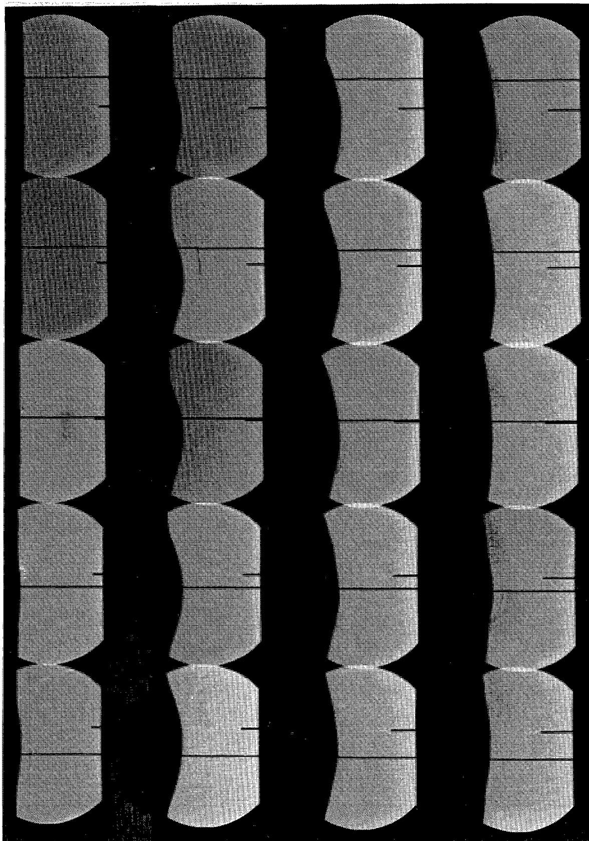
Figure 2.2 Shadowgraphs of Shot No. 10968, side view, v_p = 1007 m/s, Cer/GRP 24" x 24", total time 530 \mu\text{s}
