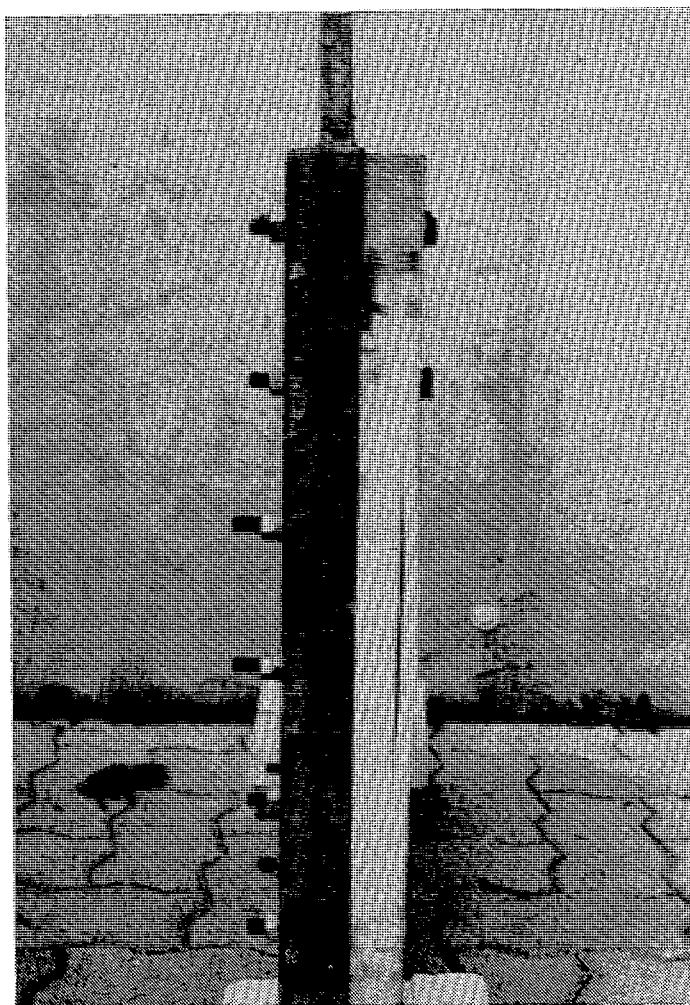
b) Side view, showing the delamination
