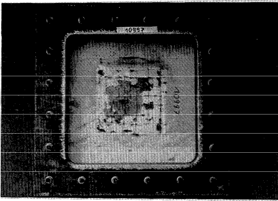
a) Impacted side
