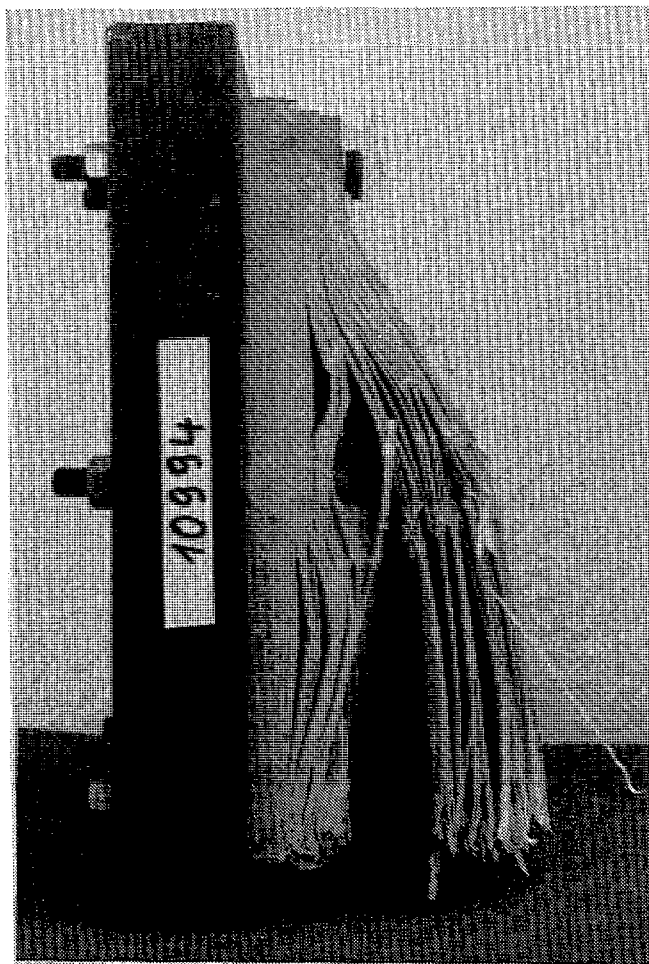
b) Side view, showing the delamination
