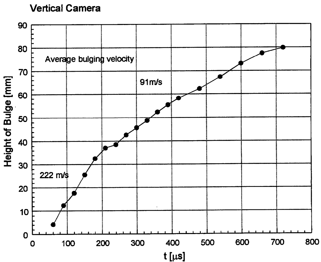
Figure 2.12 Distance-time curves of Shot No. 10973
