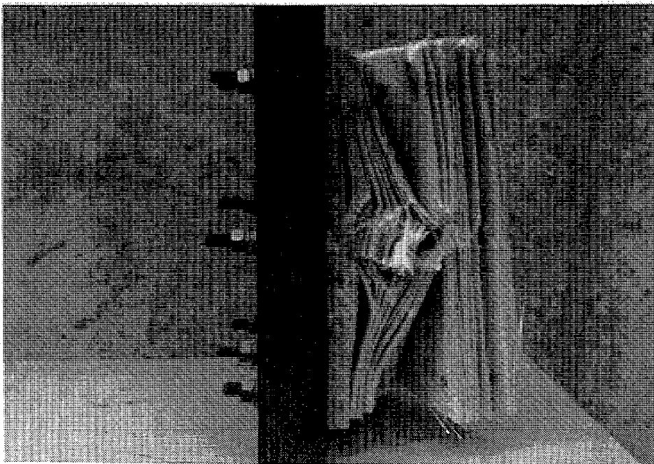
Figure 2.13 Photographs of the impacted target, Shot No. 10973
