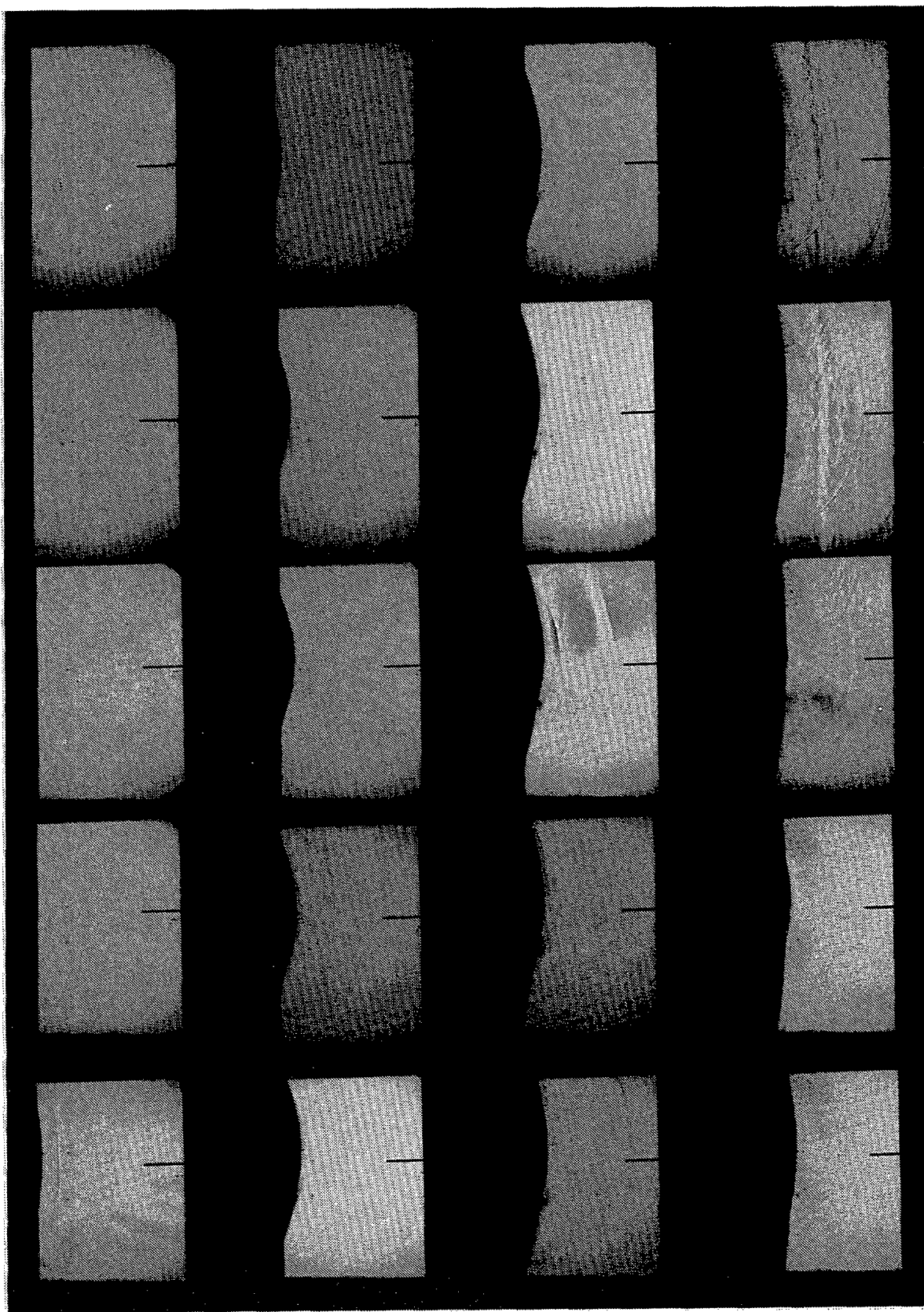
Figure 2.2 Shadowgraphs of Shot No. 10968, top view
