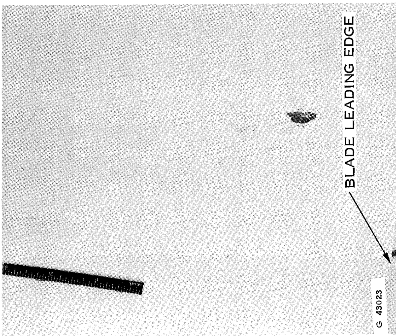
B) BOLT STRIKE — FACE SIDE OF BLADE
