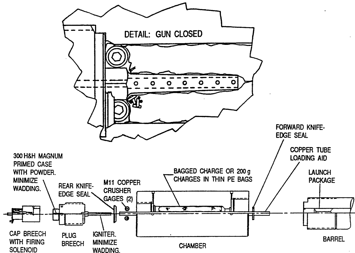
Figure 8. Original UDRI breech-end setup. (PE is polyethylene.)
