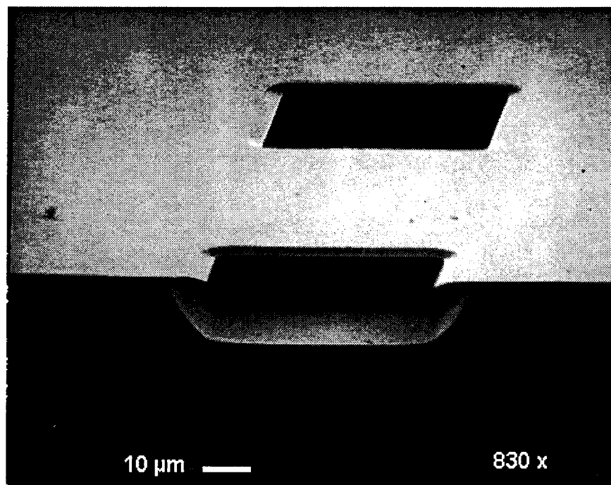
Figure 4. SEM photograph of plasma-etched recess in (100) Si. Etch parameters: power = 100 W, pressure = 200 mtorr, SF 6 flow rate = 18 sccm.
