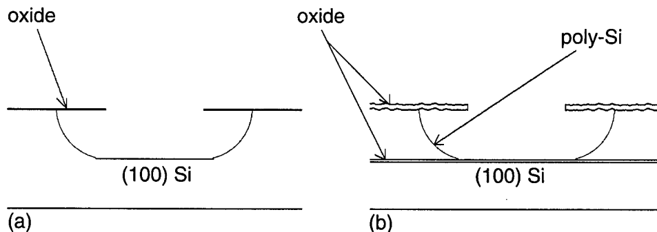
Figure 1. Two possible configurations that would allow for selective epitaxial growth in recesses. (a) Oxide masks recess, which is formed directly in single crystalline silicon. (b) Top oxide masks poly-Si recess. Bottom oxide layer protects single crystalline silicon and is removed before growth.
