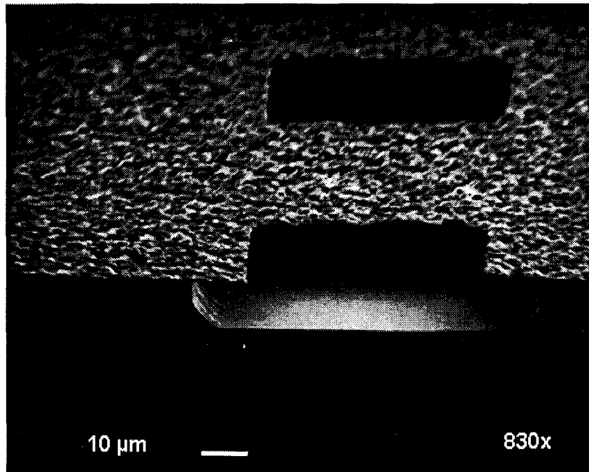
Figure 5. SEM photograph of plasma-etched poly-Si with oxide mask. Etch parameters: power = 100 W, pressure = 200 mtorr, and \text{SF}_6 flow rate = 18 sccm.
