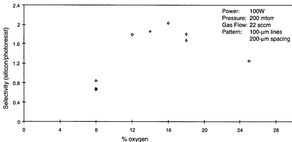
Figure 2. Etch rate selectivity (silicon/photoresist) versus percentage of oxygen content in CF 4 .
