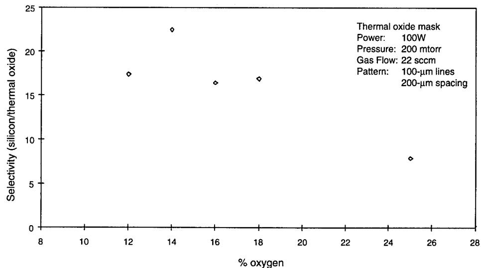
Figure 3. Etch rate selectivity (silicon/thermal oxide) versus percentage of oxygen content in CF 4 .
