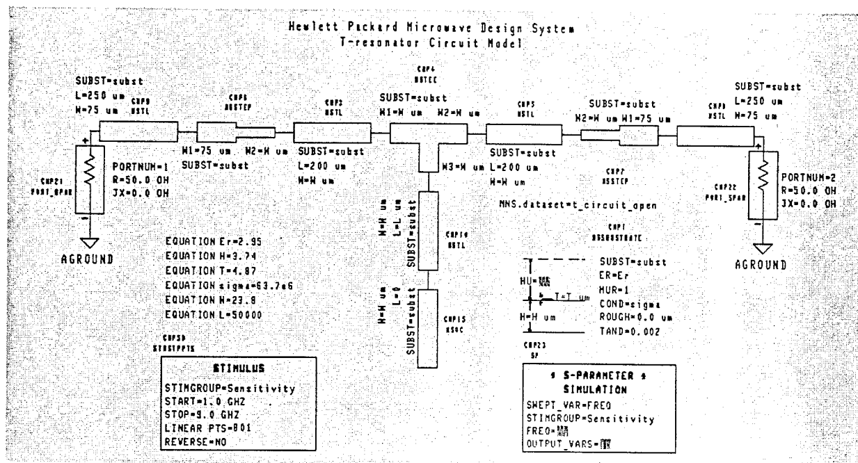
Figure 2: Schematic of T-resonator as simulated in the Hewlett-Packard Microwave Design System Software
