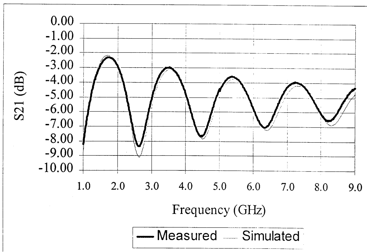
Figure 3: Plot showing measured and simulated T-resonator data
