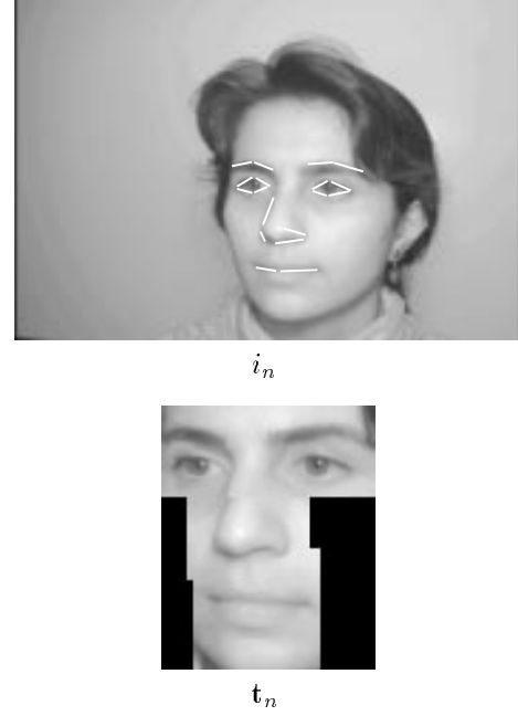
Figure 14: Using correspondences from our face vectorizer, we can geometrically normalize input i_n , producing the “shape free” texture \mathbf{t}_n .
