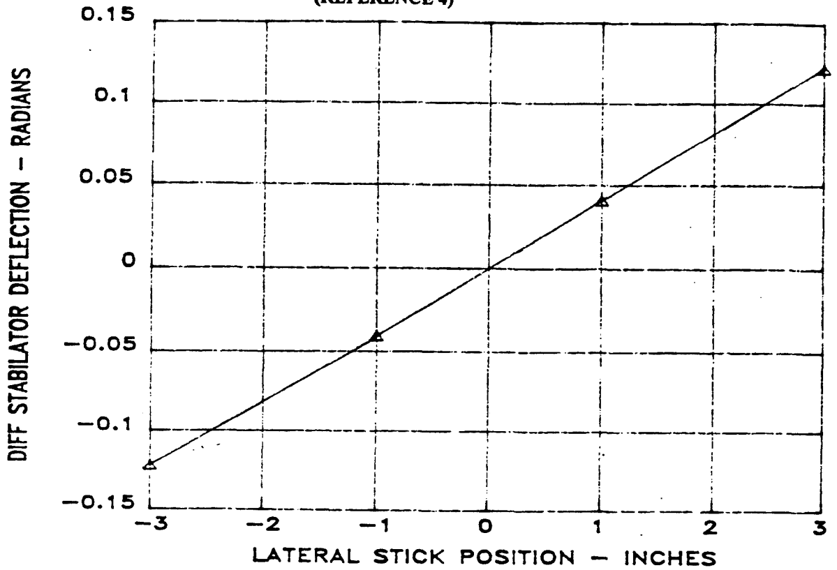
FIGURE B5. AILERON GEARING CURVE (REFERENCE 4)
