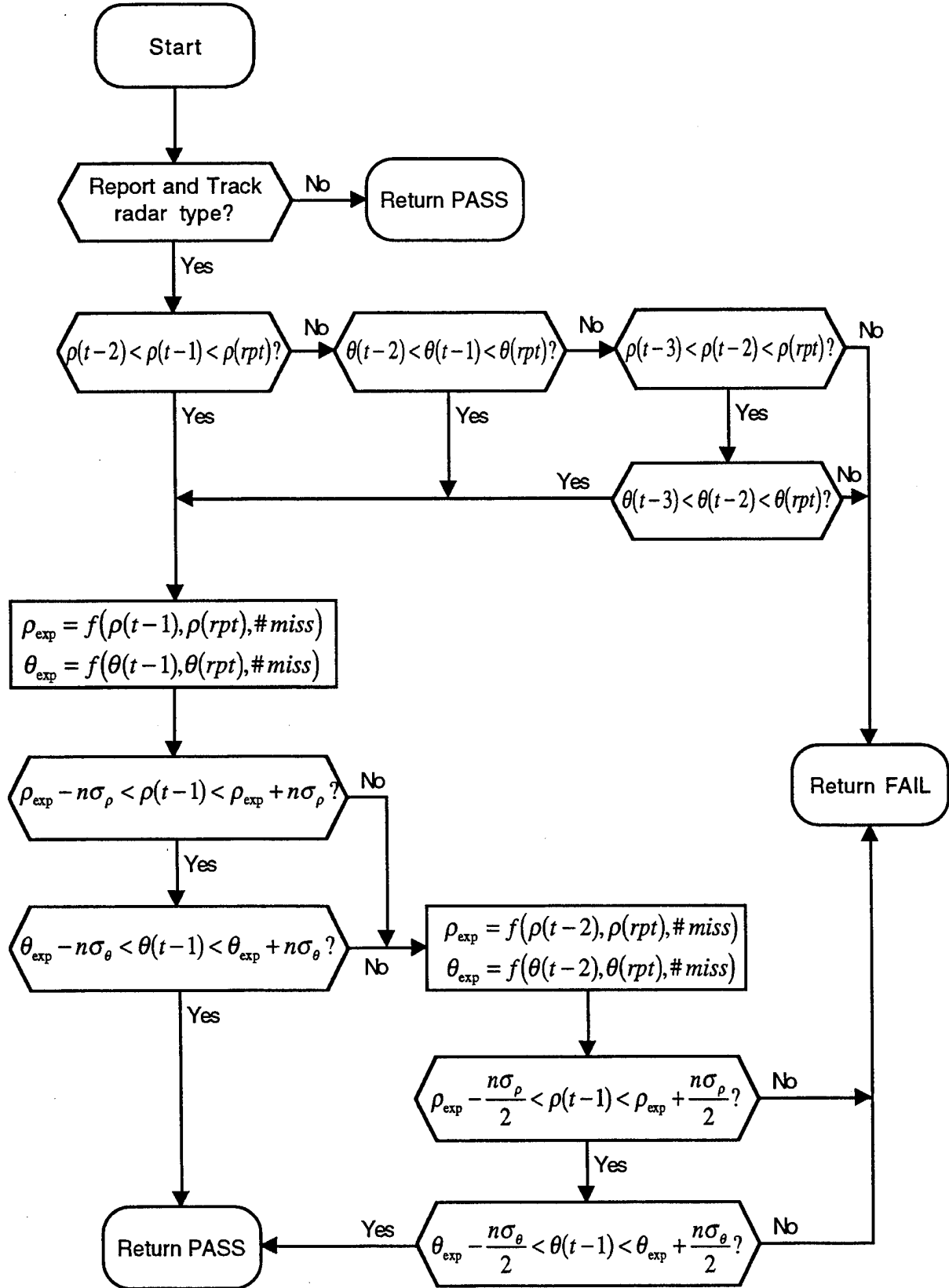
Figure 7. Linearity test.
