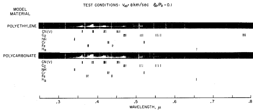
Figure 11.- Spectra of shock layer and near wake.
