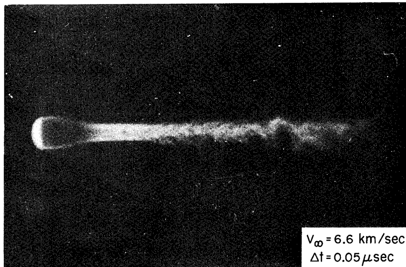
Figure 3.- Self-luminous photograph of ablating polycarbonate model.
