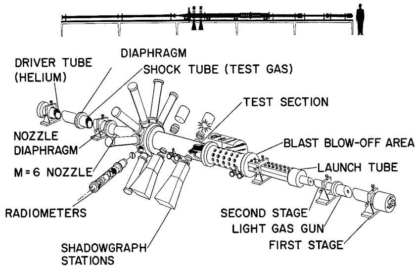
Figure 1.- Schematic drawing of Pilot Hypervelocity Free-Flight Facility.
