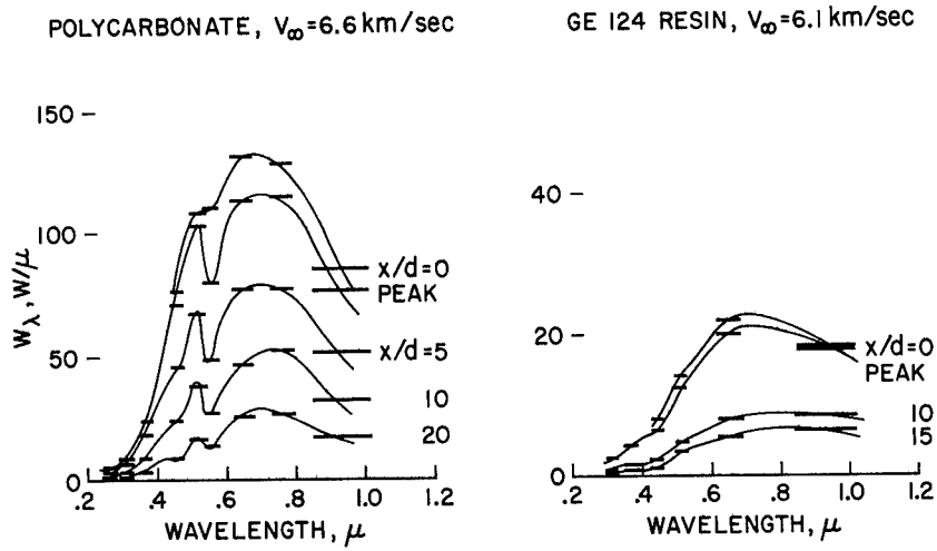
Figure 9.- Decay of wake radiance, \rho_\infty/\rho_0 = 0.08 .
