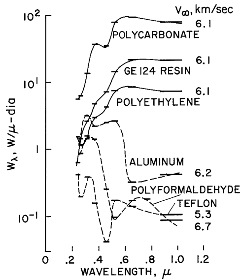
Figure 8.- Peak wake spectral radiation, \rho_\infty/\rho_0 = 0.08 .
