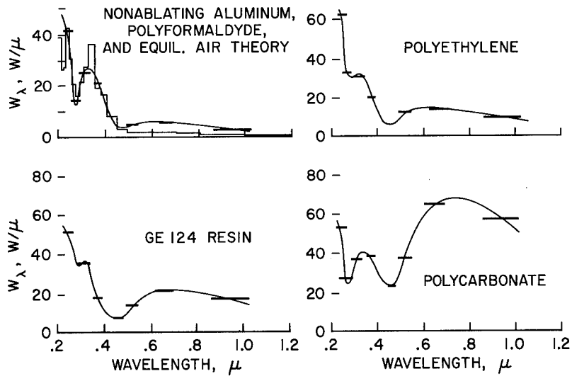
Figure 7.- Radiometric data; \rho_\infty/\rho_0 = 0.08 , V_\infty = 6 km/sec.
