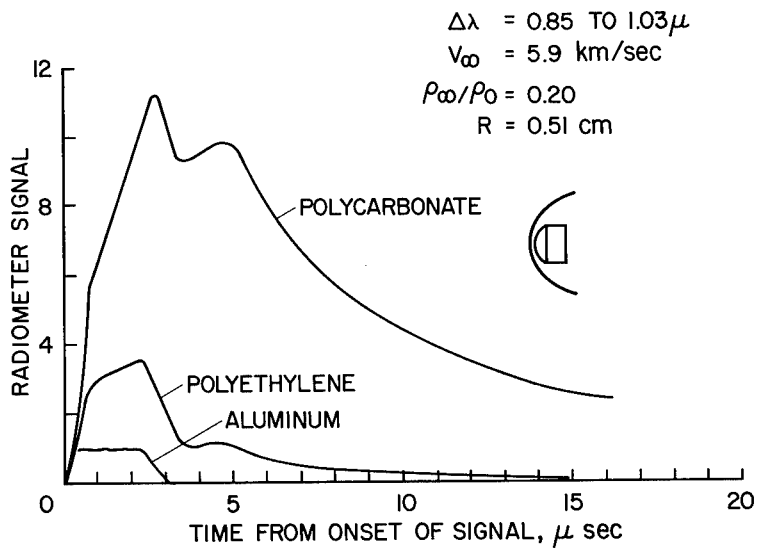
Figure 6.- Variation of infrared radiation with model material.
