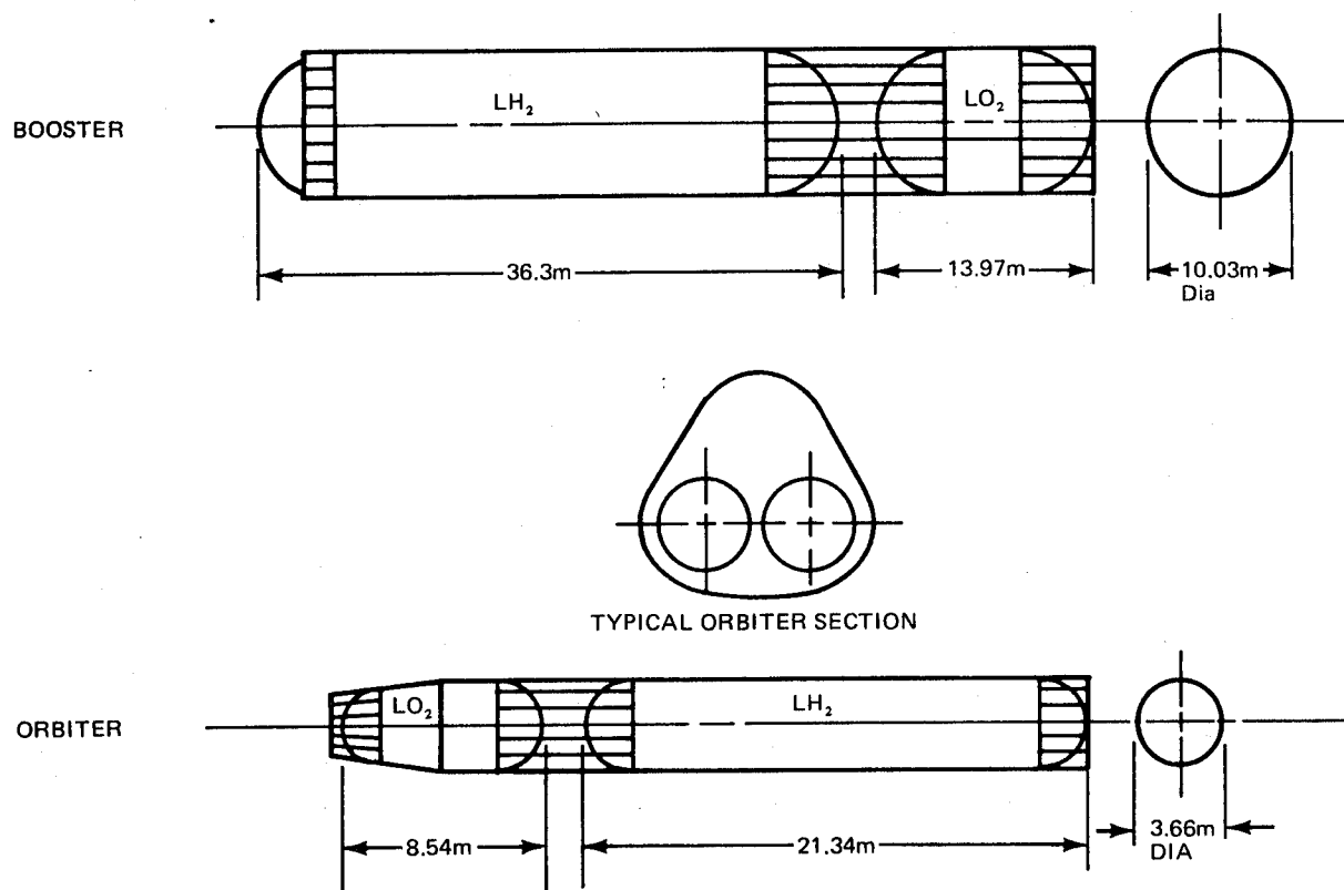
Fig. 49 Combined Orbiter/Booster Design C2F
