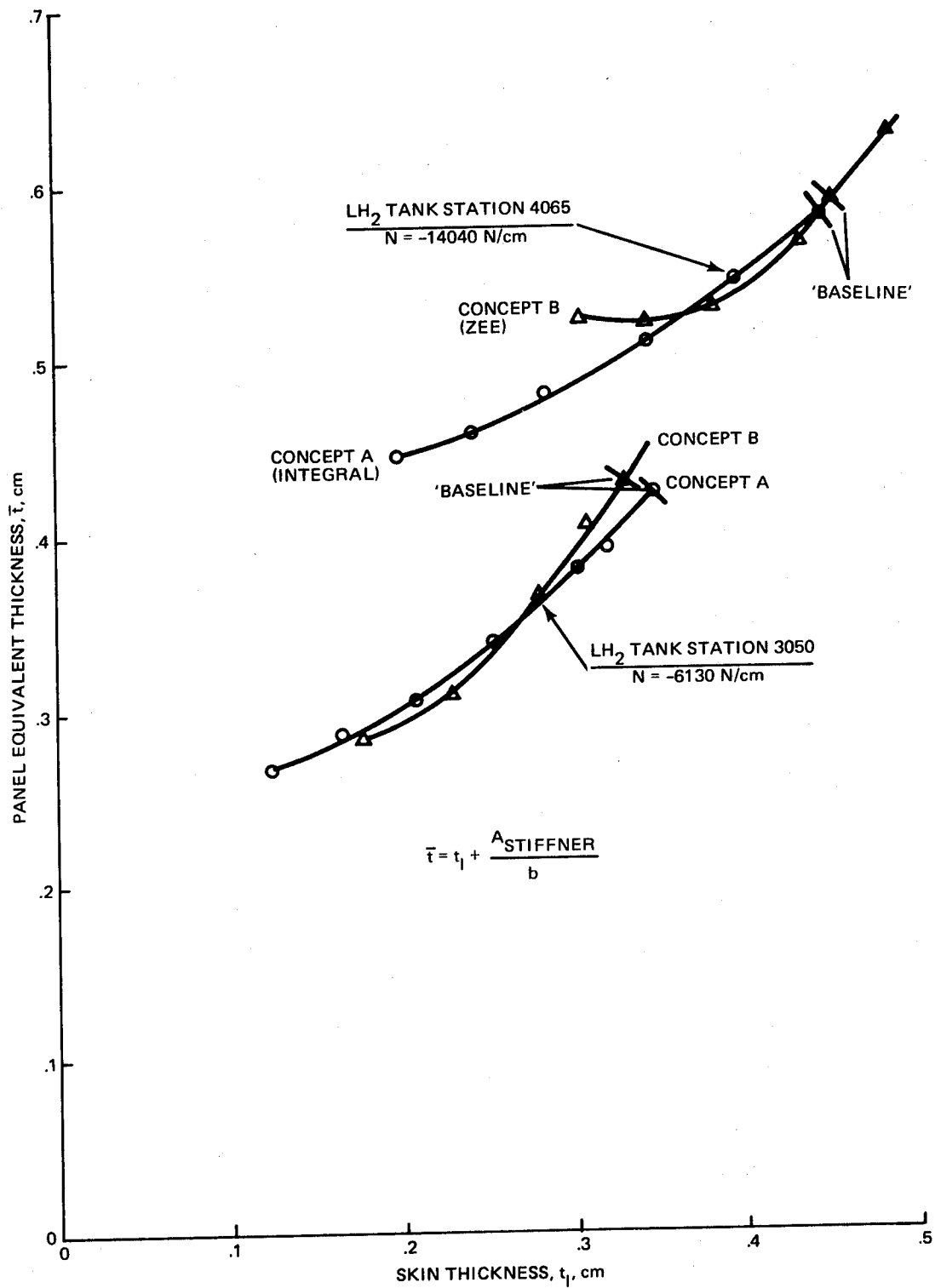
Fig. 5 Results of Compression Optimization Programs
