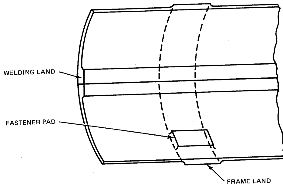
Fig. 62 Plates Rolled and Welded Longitudinally for Concept 2, Orbiter LH 2 Tank
